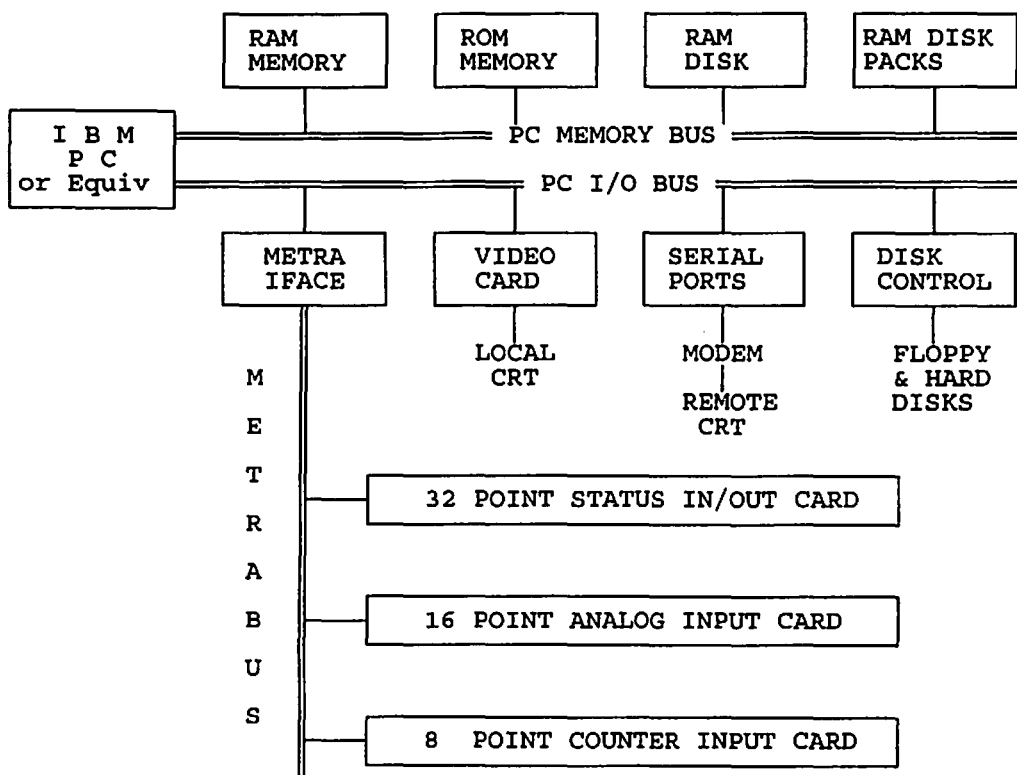
TYPICAL METRABUS BASED RTU CONFIGURATION
