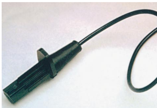
Fig. 28. Wheel speed sensor for ABS system encapsulated in RYNITE® 530 PET.
