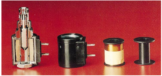
Fig. 1. Hydraulic cartridge valve from HydraForce. Coil form in RYNITE® 530 (Foremost Plastic Products Co.). RYNITE® encapsulated solenoid produced by Warsaw Coil Co.
