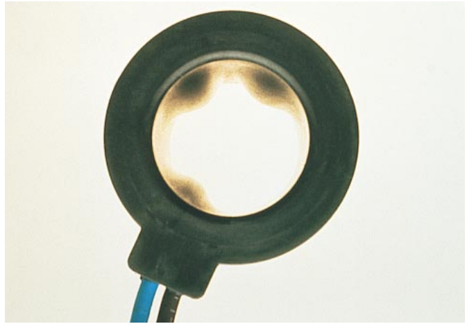
Fig. 17. Result of encapsulating a wound coil bobbin that is not fully crystallized.
