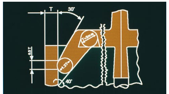
Fig. 15. Gate design for encapsulation recommended by DuPont.
