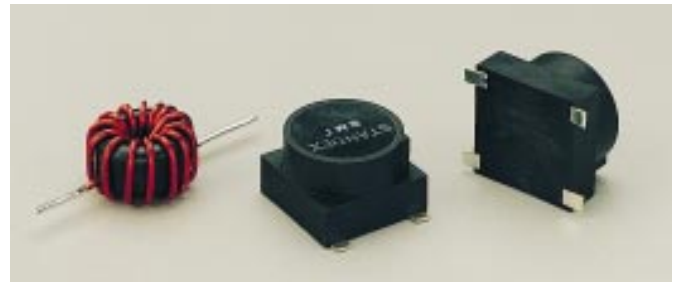
Fig. 32. ZYTEL® nylon resin encapsulated toroids for surface-mount applications (Standex Electronics).
