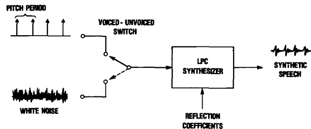
Fig. 1. Block diagram of an LPC speech synthesizer using a periodic pulse train for synthesizing voiced speech and white noise for synthesizing unvoiced speech.
