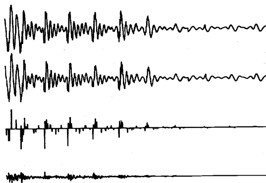
Fig. 9. Another example of the waveforms of the original speech, the synthetic speech, the excitation signal, and the error.
