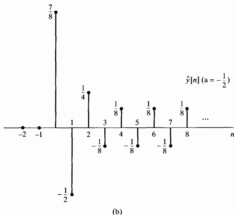
Figure 6.62 Response of the first-order system of Figure 6.61 to an impulse. (a) a = 1/2 . (b) a = -1/2 .
