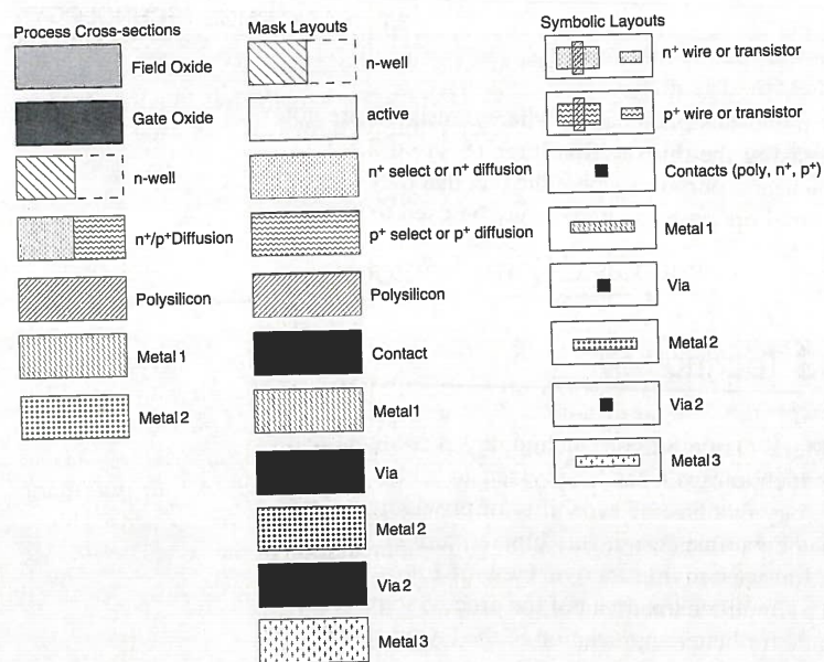
FIGURE 3.6 CMOS process and layout drawing conventions
