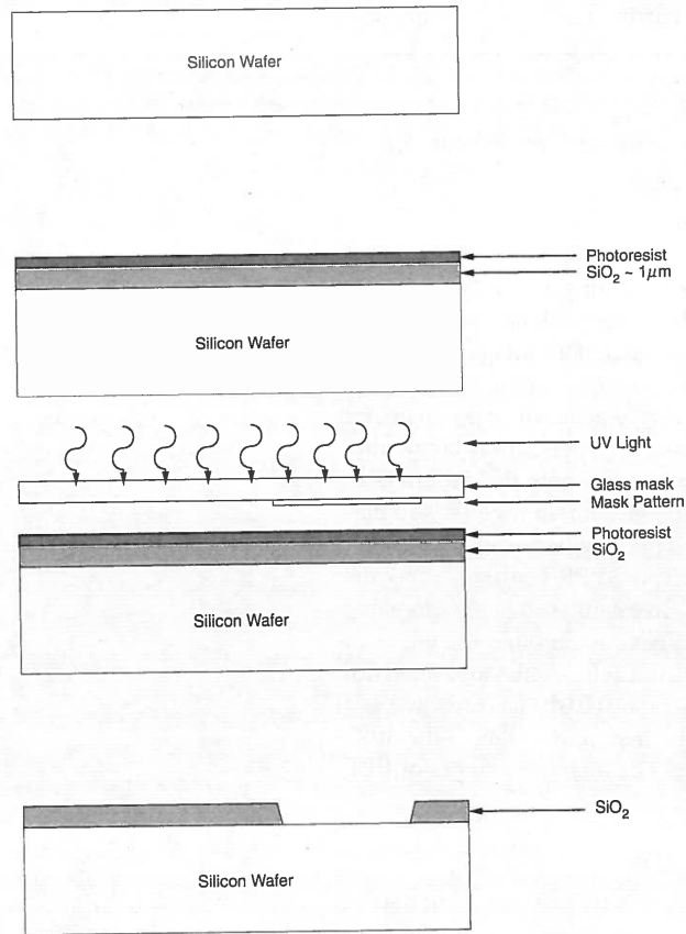
FIGURE 3.3 Simplified steps involved in the patterning of SiO 2 : (a) Bare silicon wafer; (b) Wafer with SiO 2 and resist; (c) Exposing resist to UV light; (d) Final etched SiO 2
