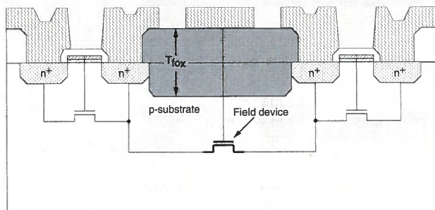
FIGURE 3.5 A parasitic MOS transistor or field device
