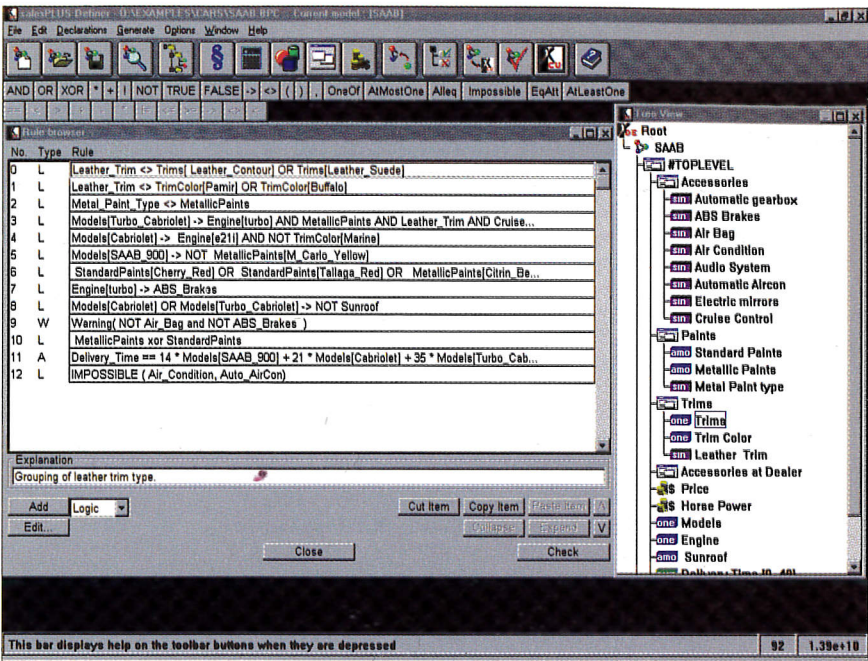
Figure 5. Saab objects and constraints in the salesPLUS Definier.
