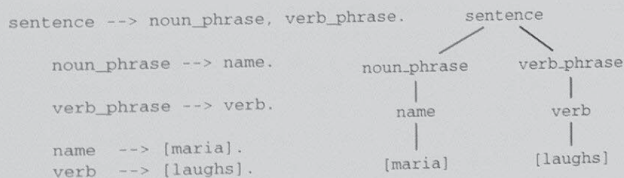
FIGURE 1. A sample grammar and parse tree.
