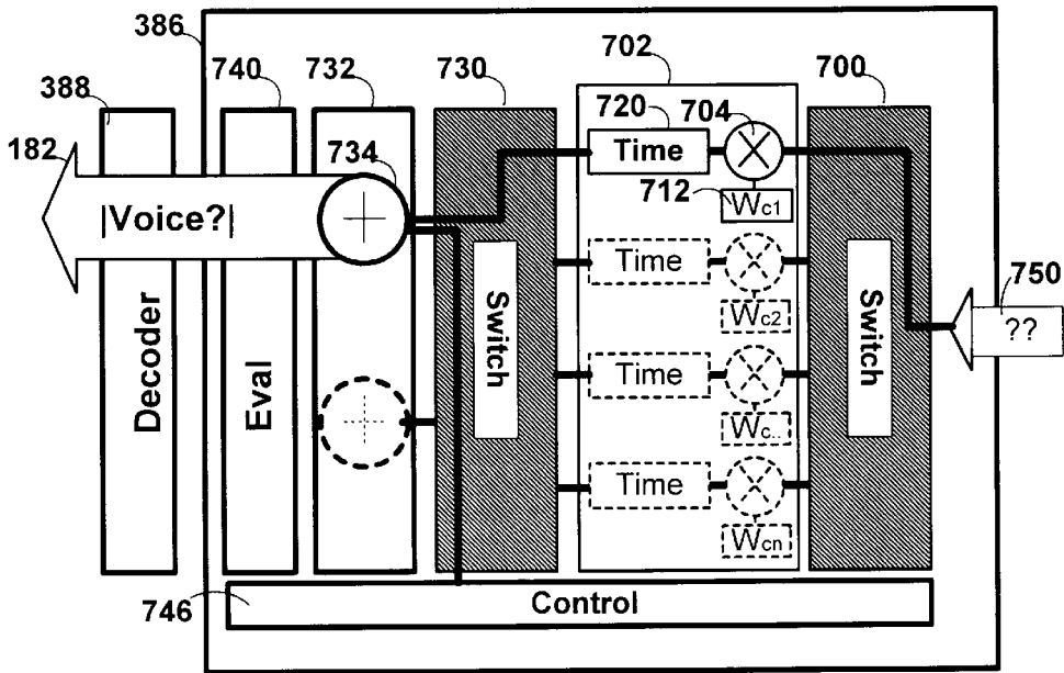
Space-Time Processor FIG. 7C
