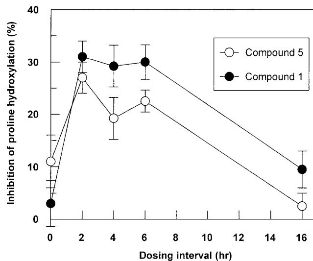
Figure 2 Time course of the inhibition in vivo of the hydroxylation of proline residues of newly synthesized uterine collagen in rats by Compounds 1 and 5
