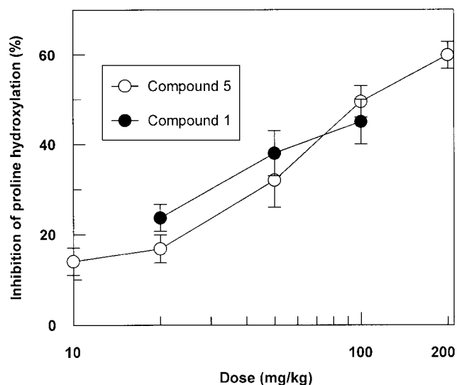
Figure 1 Dose responses for the inhibition in vivo of the hydroxylation of proline residues of newly synthesized uterine collagen in rats 6 h after single oral doses of Compounds 1 and 5
