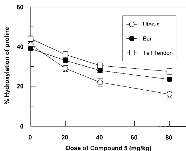
Figure 3 Inhibition by Compound 5 of the 4-hydroxylation of proline residues of newly synthesized collagen of various tissues in vivo in the rat 6 h after the compound was given orally to groups of ten animals
