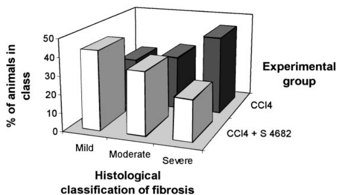
FIG. 5. Effect of S 4682 on liver fibrosis in CCl_4 fibrotic rats based on histological examination. Dark columns, rats treated with rats CCl_4 only ( n = 80 ); light columns, rats treated with CCl_4 + S 4682 ( n = 58 ). The ordinate shows the percentage of rats with histologically mild (score 1 and 2), moderate (score 3), and severe fibrosis (score 4 and 5). The percentage of rats with individual histological scores from 1 to 5 was 3.8, 22.5, 30, 27.5, and 16.3 in the CCl_4 group (mean \pm SD, 3.3 \pm 1.107 ), and 10.3, 32.8, 34.5, 20.7, and 1.7 in the CCl_4 + S 4682 group (mean \pm SD, 2.71 \pm 0.973 ), respectively. The difference between the groups was statistically significant ( P = .022 ). There were no rats with histologically normal liver in either the CCl_4 or the CCl_4 + S 4682 groups.
