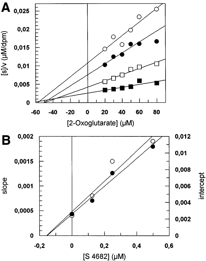
FIG. 3. (A) [s]/v versus [s] plot for the inhibition of P4H by S 4682 using 2-oxoglutarate as the variable substrate. [s], concentration of substrate; v, reaction velocity. The plot is best described as noncompetitive. The concentrations of S 4682 were: (○) = 0.5 µmol/L; (●) = 0.25 µmol/L; (□) = 0.125 µmol/L; (■) = uninhibited samples. Each point is the average of three independent experiments. (B) Secondary transformation of the data presented in (A). The K is value is calculated from the slopes of the regression line of (A) (○). The K ii value is calculated from the intercepts of the regression line of (A) (●).
