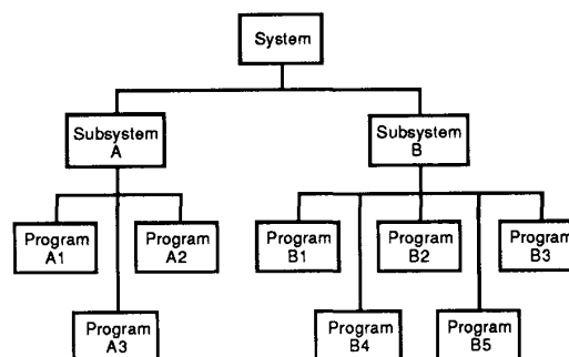
Fig 16 Structure Chart
