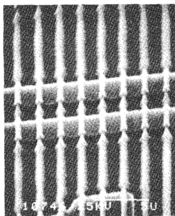
Fig. 5. 1- \mu m lines and spaces in 1 \mu m of resist over 0.5- \mu m polysilicon steps.
