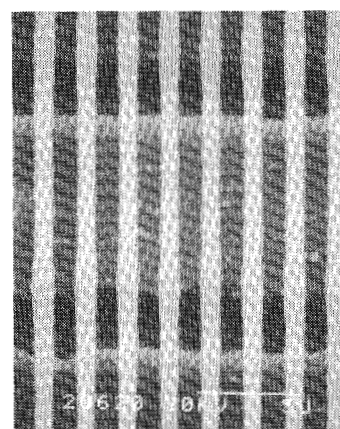
Fig. 14. 1- \mu m lines and spaces in tri-layer resist with 2.0- \mu m HPR 204 + 1.5-percent dye as the bottom polymer over 1.0- \mu m aluminum steps after reactive etching.
