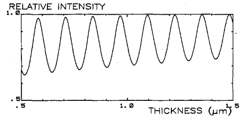
Fig. 3. The fractional intensity coupled into HPR 204 positive resist ( N = 1.69 - i0.12 ) on a silicon substrate as a function of the resist thickness.
