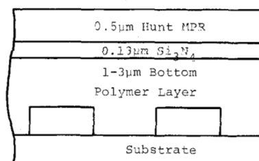
Fig. 6. Tri-layer resist system.
