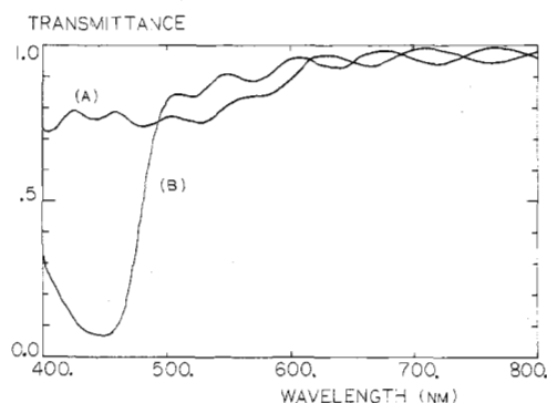
Fig. 7. Transmittance spectra of (A) 1.5- \mu m HPR 204 and (B) 1.7- \mu m HPR 204 with 1.5-percent concentration of dye by weight in solution after hard bake in a box oven at 160°C for 30 min.
