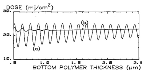
Fig. 8. Nominal dose versus bottom polymer thickness for the tri-layer system of Fig. 6 on an aluminum substrate for (a) HPR 204 for the bottom polymer and (b) HPR 204 with 1.5-percent dye. Simulations are for 1- \mu m lines and spaces under perfect focus.
