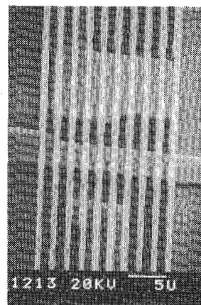
Fig. 13. 1- \mu m lines and spaces in tri-layer resist with 2.0- \mu m HPR 204 as the bottom polymer over 0.5- \mu m aluminum steps after reactive ion etching.
