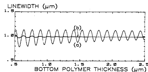
Fig. 10. Simulated linewidth versus bottom polymer thickness for 1- \mu\text{m} lines and spaces for a bottom polymer of (a) HPR 204 and (b) HPR 204 with 1.5-percent dye.
