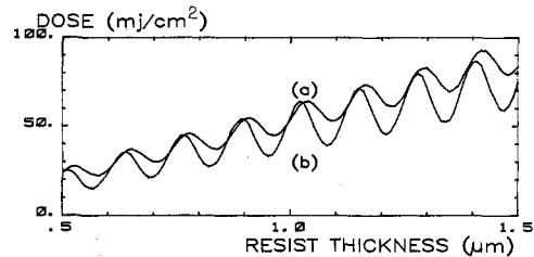
Fig. 4. The exposure energy density (dose) required at 436 nm to achieve 1- \mu m lines and spaces in HPR 204 on (a) silicon and (b) aluminum for \lambda = 436 nm, NA = 0.28, perfect focus, and partial coherence factor \sigma = 0.7 .
