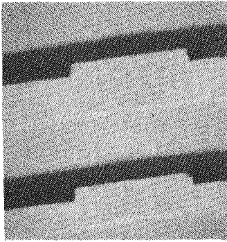
Fig. 1. Resist step coverage: 1- \mu m-thick resist pattern over 0.5- \mu m step.
