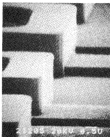
Fig. 9. Edge profile of 2.0 \mu\text{m} of HPR 204 on 0.5- \mu\text{m} polysilicon steps after reactive ion etching.
