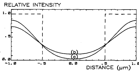
Fig. 2. The image intensity pattern of a periodic 1- \mu m line and space for the case of (a) perfect focus and (b) 3 \mu m of focus error. \lambda = 436 nm; NA = 0.28; partial coherence factor ( \sigma ) = 0.7; square aperture. (Dashed line is the intensity at the reticle.)
