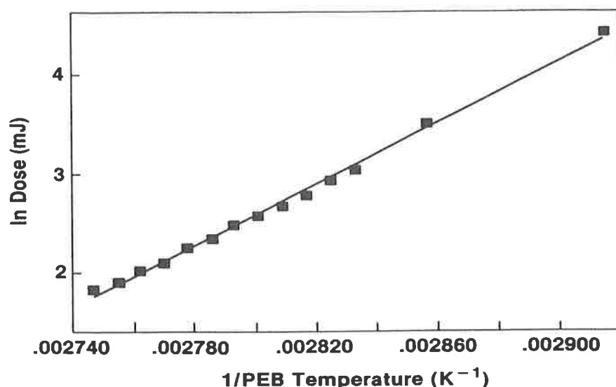
Figure 17 Arrhenius plot of resist sensitivity vs. PEB temperature for a DUV CAR resist. Dose required to print 0.5 \mu\text{m} lines with a 90 second bake is plotted against 1/PEB temperature. An effective activation energy can be calculated from such a plot (130 kJ/mole in this case). (From Ref. 41.)
