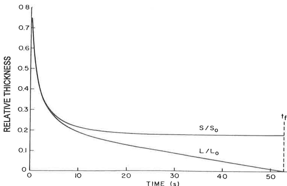
Figure 2 Calculated time dependance during spin coating on the volume of solids ( S ) and solvent ( L ) per unit area normalized to initial values. When the resist thickness drops to one third of its original value, evaporation dominates and the solvent content reaches its final value. (From Ref. 19.)
