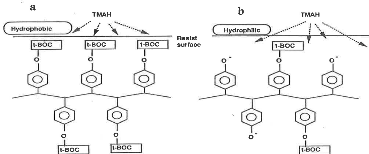
Figure 28 A proposed dissolution model for positive DUV chemically amplified resist derived from Arrhenius plot analysis. Two situations are considered: (a) before deprotection where TMAH penetration is prevented by strong hydrophobicity and (b) after deprotection. (From Ref. 69.)
