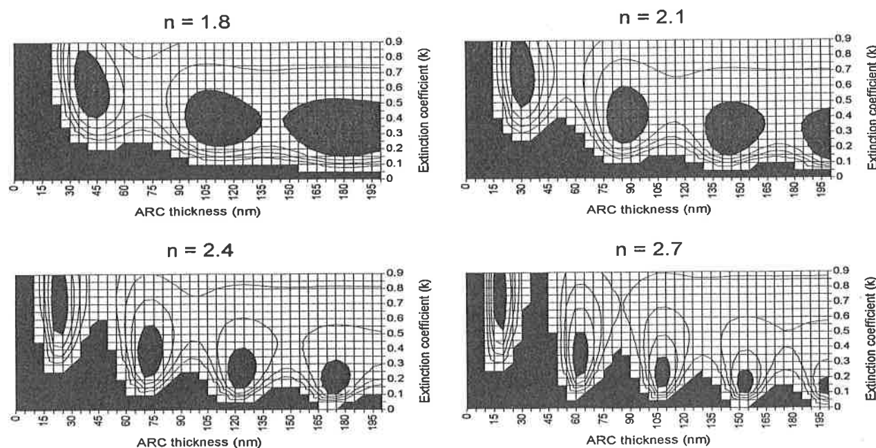
Figure 8 Contour plots of substrate reflectivity (over silicon) at 248 nm as a function of bottom ARC thickness for materials with refractive indices between 1.8 and 2.7 and extinction coefficient values to 0.9. Central contour areas correspond to 0-2% reflectivity and 2% constant contours are shown. Results beyond 10% reflectivity are shown in black [ n_{\text{resist}}(248) = 1.75 ].
