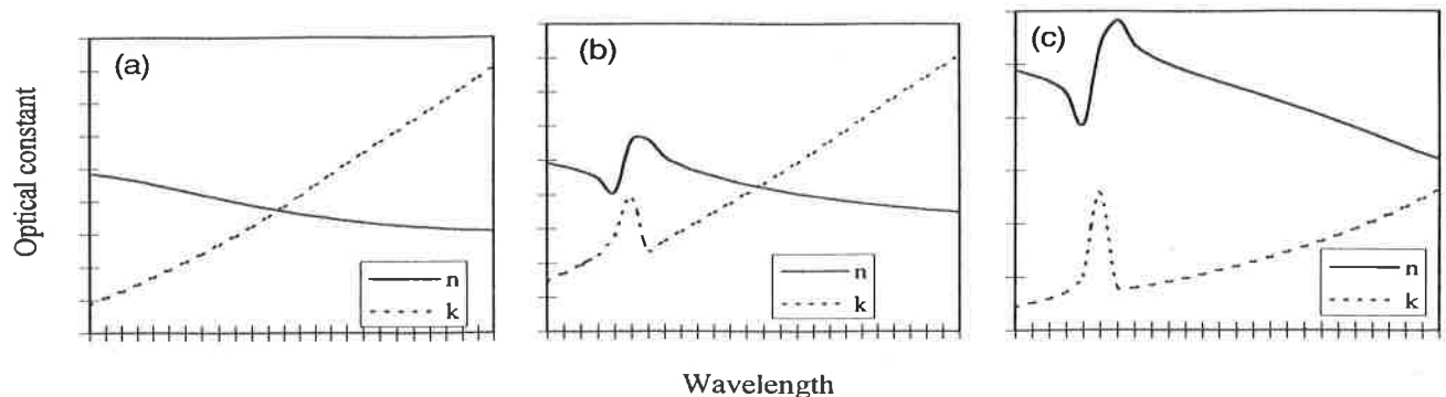
Figure 12 Plots of optical constants for a metallic film using the Drude model for free electron motion and metallic-dielectric composite films using combined free and bound electron models. (a) A metallic film; (b) a dielectric film; and (c) a dielectric composite film with increasing metallic content.
