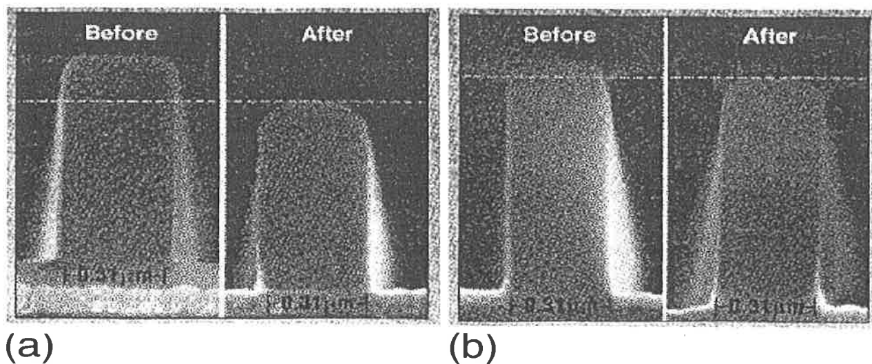
Figure 15 A comparison of resist loss during pattern transfer to bottom ARC layers. (a) Organic spin-on ARC; and (b) dielectric inorganic ARC. [From C. Bencher, C. Ngai, B. Roman, S. Lian, and T. Vuong, Solid State Technol. , 111, (1997).]
