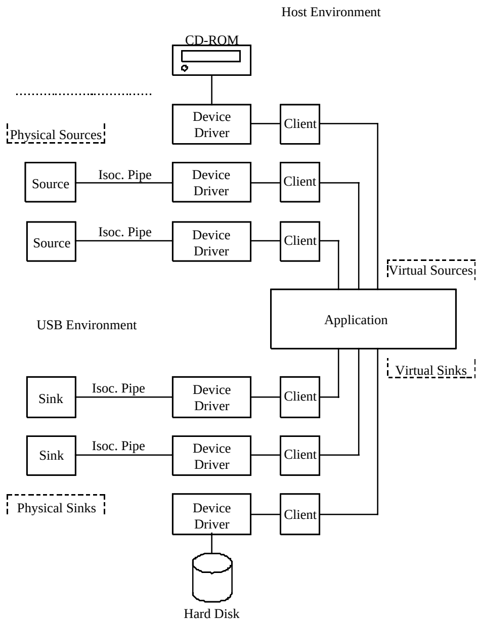
Figure 5-18. Example Source/Sink Connectivity
