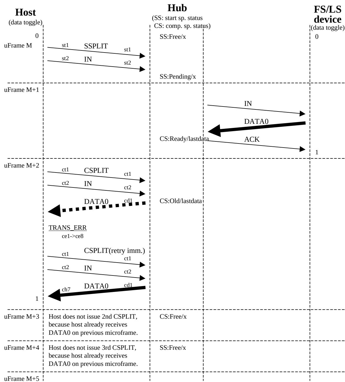
Figure A-68. Normal HS DATA0/1 Smash
