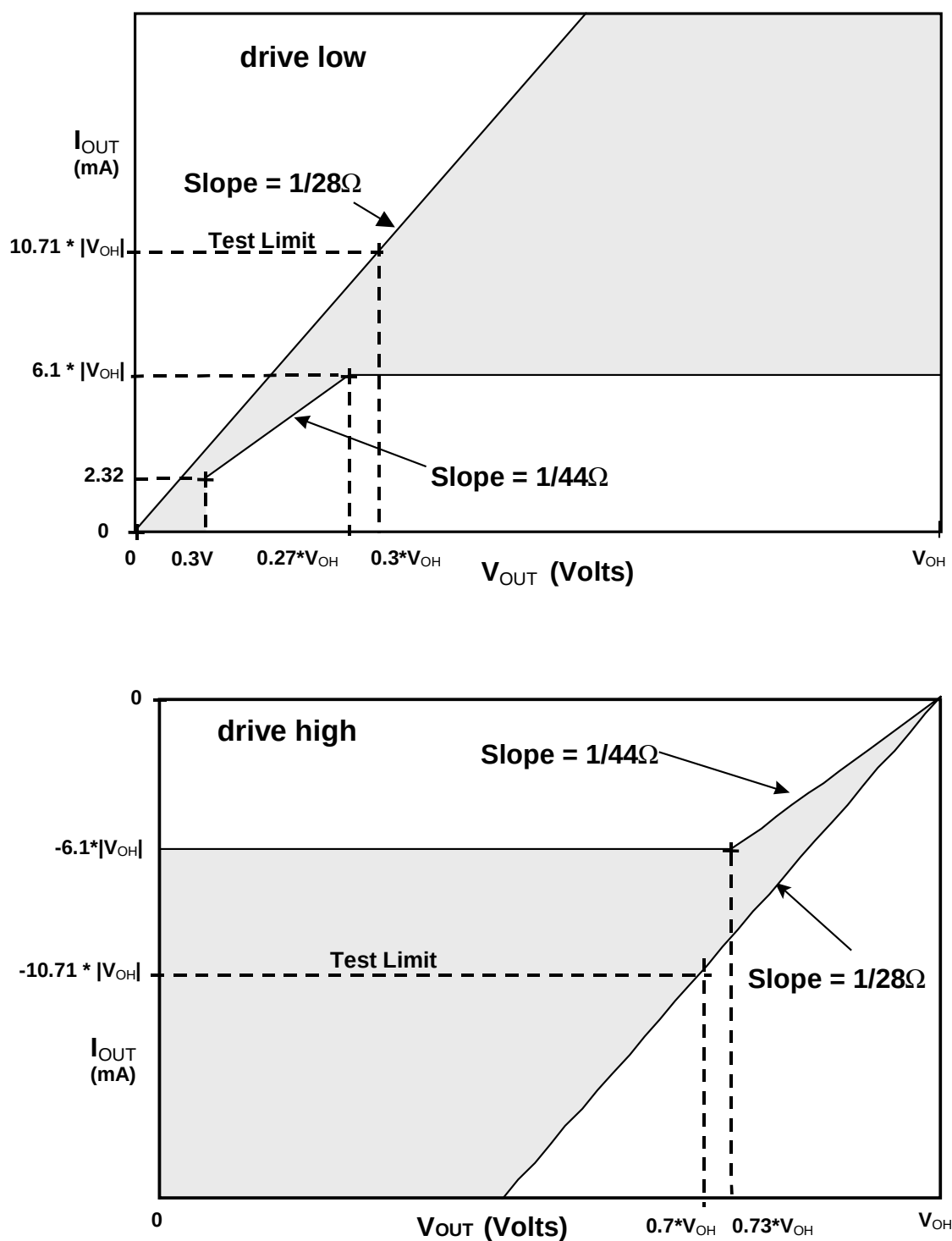
Figure 7-4. Full-speed Buffer V/I Characteristics
