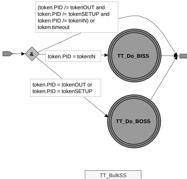
Figure 11-42. TT_BulkSS
