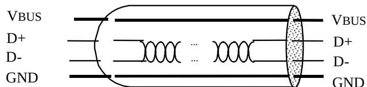
Figure 4-2. USB Cable
