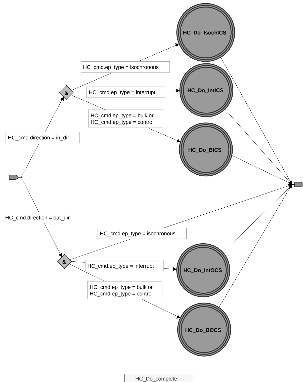
Figure 11-37. HC_Do_Complete
