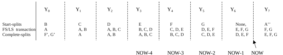
Figure 11-66. Microframe Pipeline
