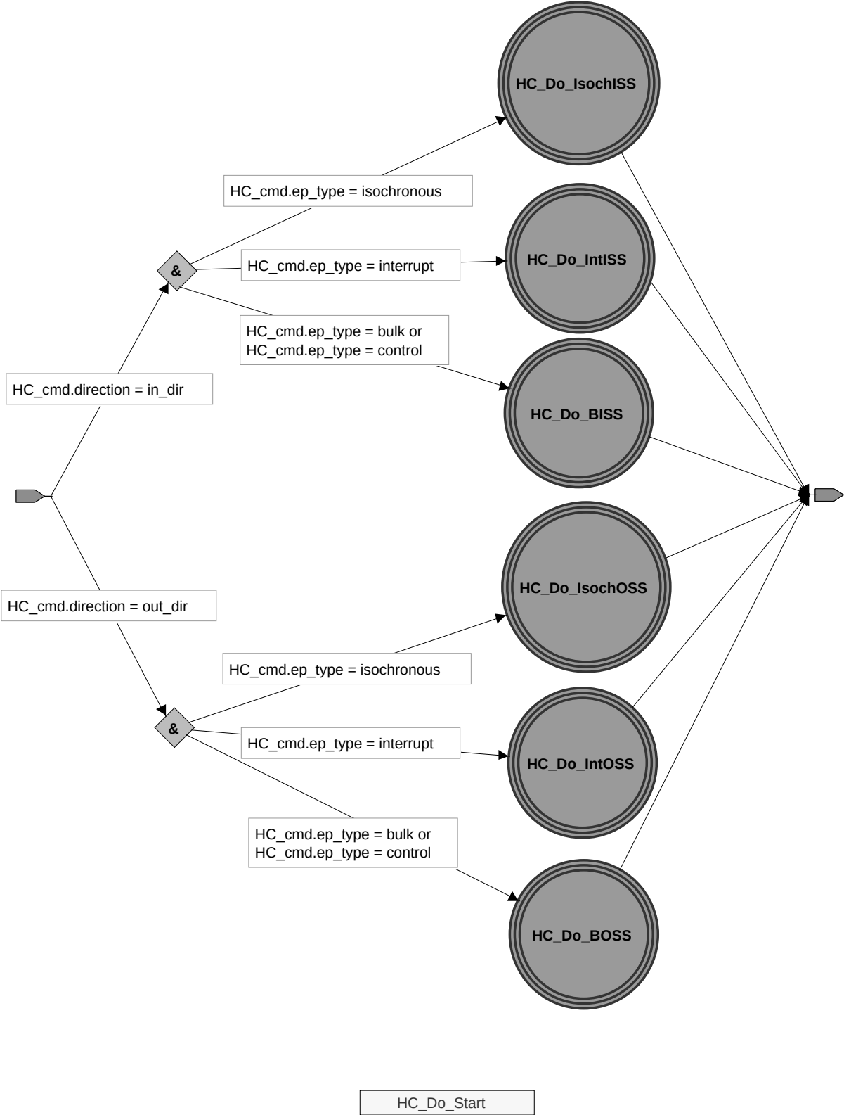
Figure 11-36. HC_Do_Start
