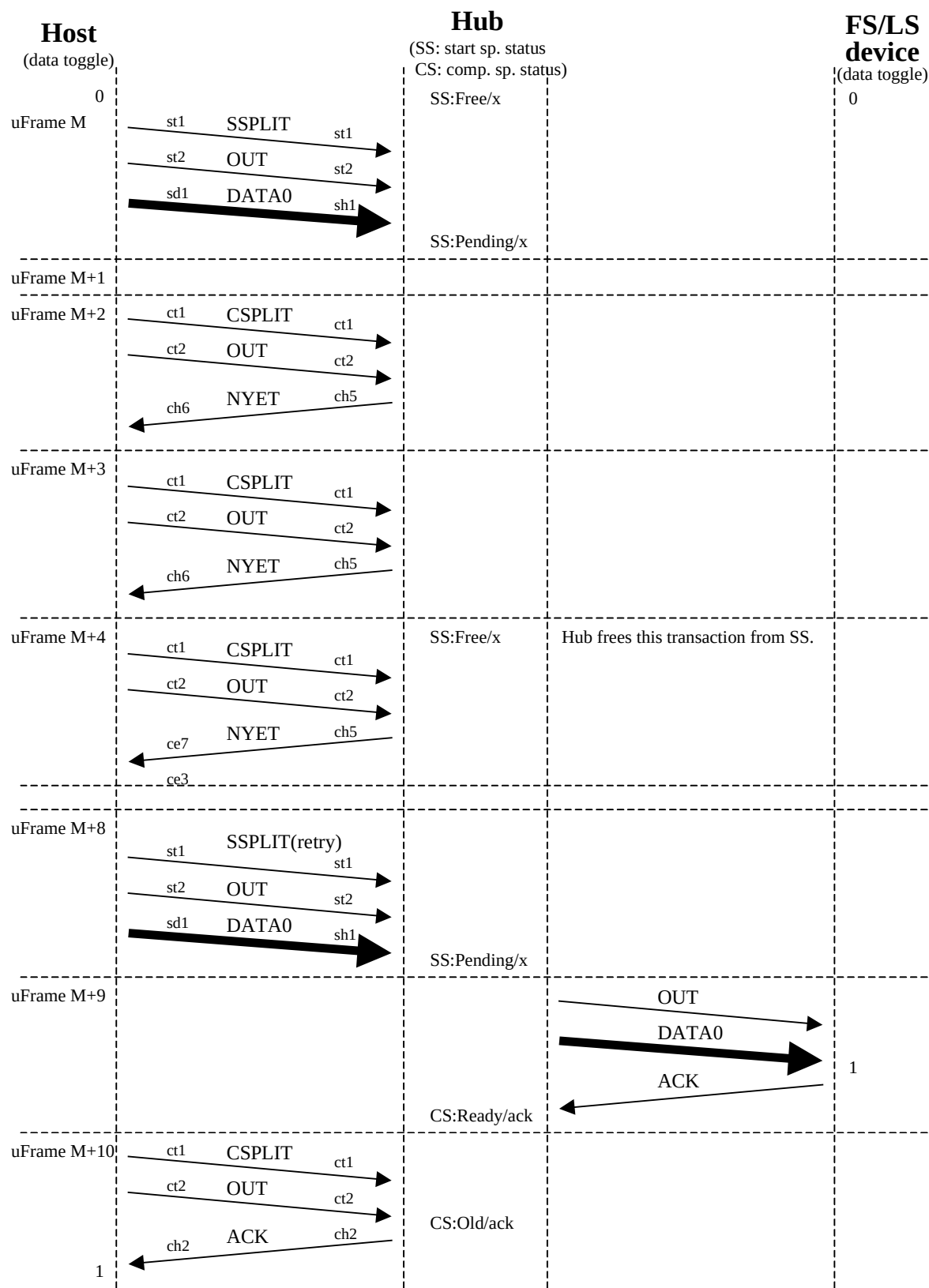
Figure A-61. Abort and Free Free(FS/LS Transaction is not Started at End of M+3)
