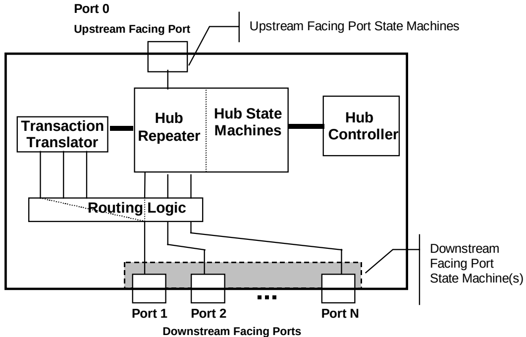
Figure 11-1. Hub Architecture
