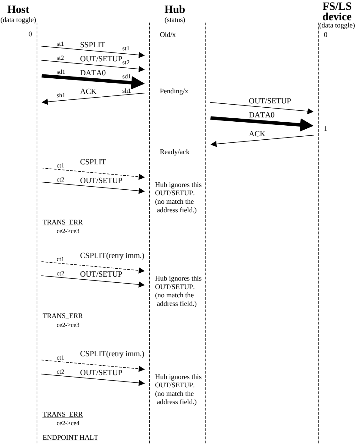
Figure A-8. Normal HS CSPLIT 3 Strikes Smash
