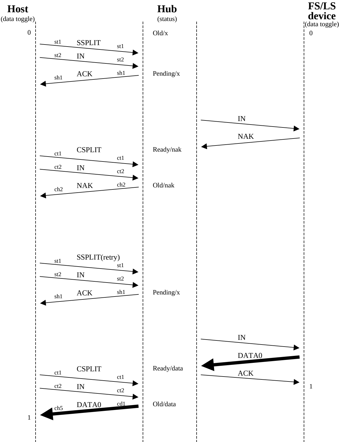
Figure A-45. Device Busy No Smash(FS/LS NAK)
