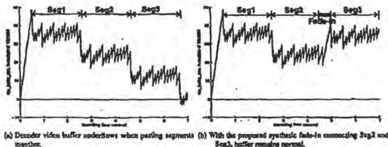
FIGURE 4. Connecting MPEG video segments in the compressed domain.
