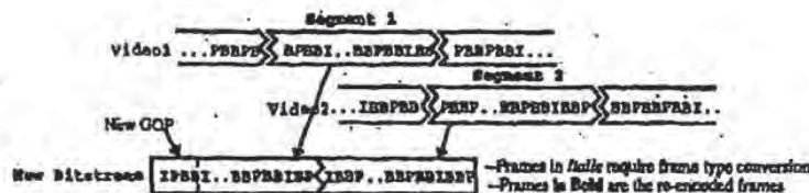
FIGURE 3. Cut and Paste MPEG Bitstreams in the compressed domain.
