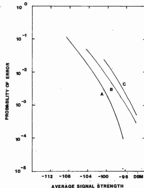
Fig. 12. Retransmission failure probability P_2 for a Type II hybrid SRT ARQ in fading. A: 20 mi/h. B: 10 mi/h. C: 6 mi/h.
