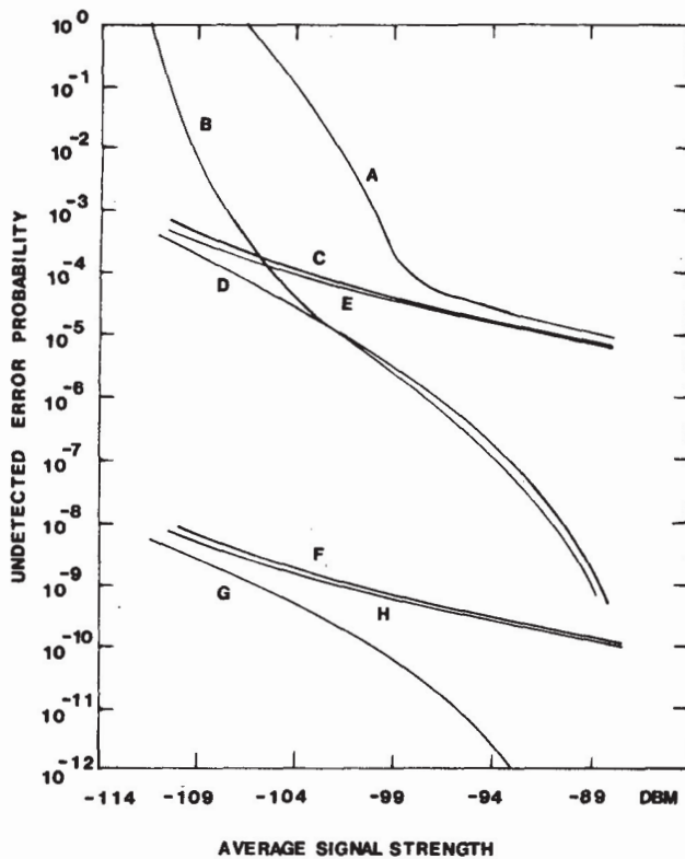
Fig. 15. Undetected error rates for 20 mi/h fading. A: Plain ARQ. B: Type I hybrid ARQ with whole message CRC. C: SRT ARQ. D: Type I hybrid SRT ARQ. E: Type II hybrid SRT ARQ with per block CRC. F: SRT ARQ. G: Type I hybrid SRT ARQ. H: Type II hybrid SRT ARQ with per block and whole message CRC.
