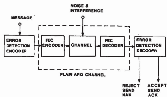
Fig. 3. Type I hybrid ARQ forward channel.
