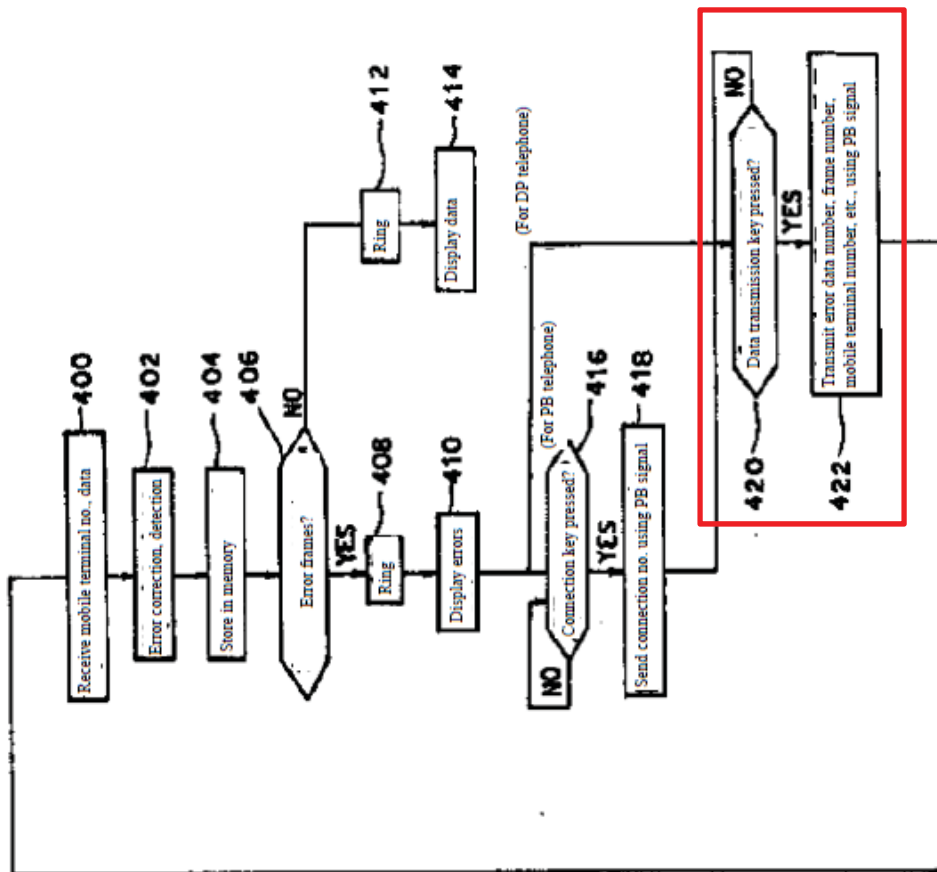
Operation flow of mobile terminal
