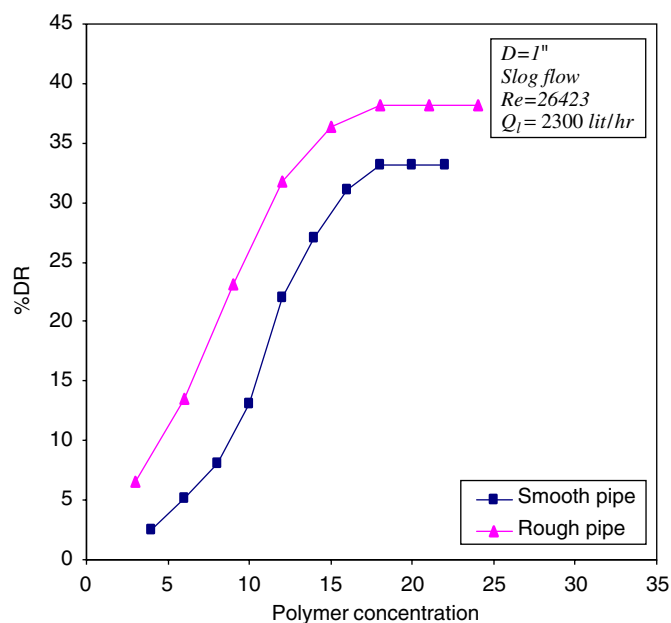
Fig. 6. Comparison of %DR versus DRA concentration for smooth and rough pipes.
