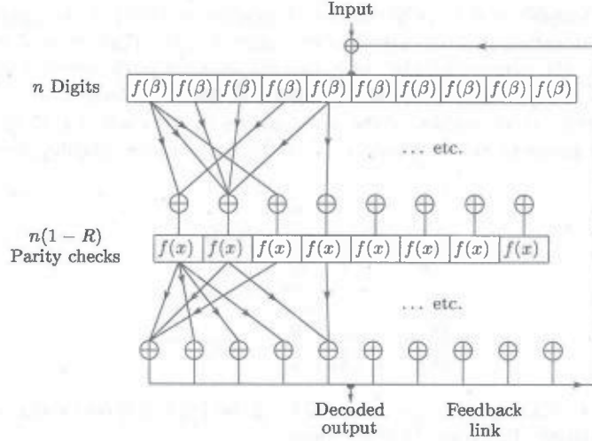
Figure 4.2: Decoding apparatus
