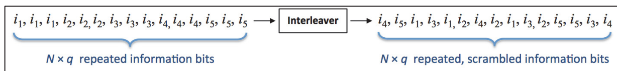
Example of Interleaving as Described in Divsalar, with N=5 and q=3
