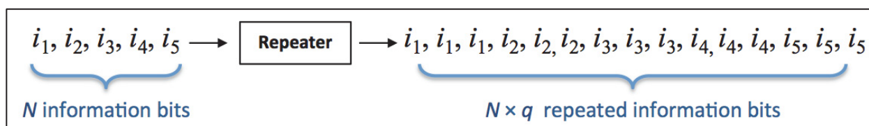
Example of Repetition as Described in Divsalar, with N=5 and q=3
