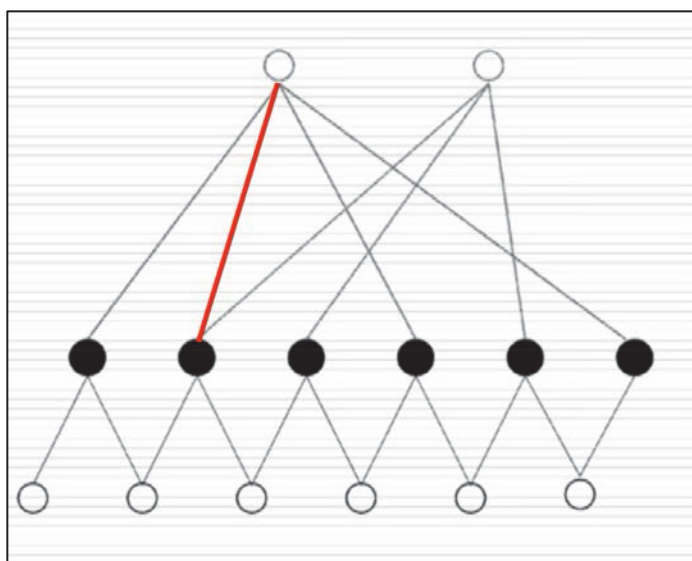
Tanner Graph of an IRA Code
