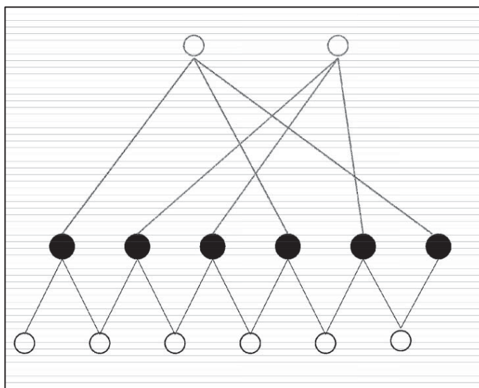
Tanner Graph of an RA Code (CALTECH000007326)
