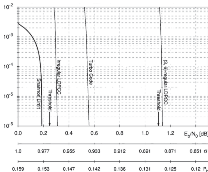
Richardson, Fig. 2, comparing performance of various codes
