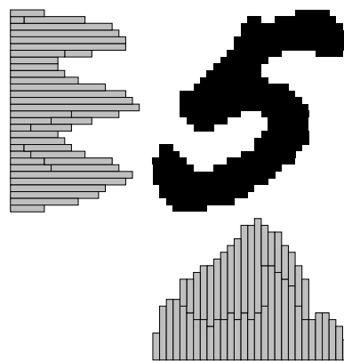
Figure 11: Horizontal and vertical projection histograms.
