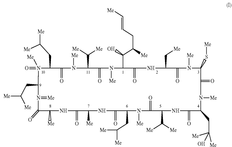
Formula IV
