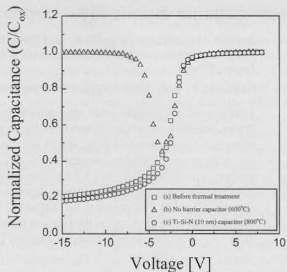
FIG. 3. 1 kHz C-V measurements for MOS capacitors. Cu (100 nm)/10 nm Ti-Si-N barrier layer (or without the barrier layer)/ \text{SiO}_2 (100 nm)/N-type Si. (a) and (b) are the C-V profiles for the MOS capacitor without the barrier layer before and after thermal treatment at 600 °C for 60 min in \text{H}_2 (10%)/Ar (90%), respectively. (c) is the C-V profiles for the MOS capacitor with a 10 nm Ti-Si-N barrier layer after thermal treatment at 800 °C for 60 min in \text{H}_2 (10%)/Ar (90%).
