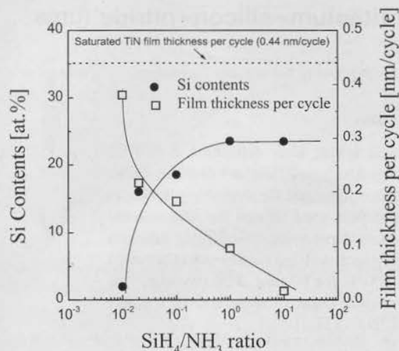
FIG. 2. Dependence of the Si content in the Ti-Si-N films and deposition thickness per cycle on the \text{SiH}_4/\text{NH}_3 ratio for the films grown on \text{SiO}_2 at the substrate temperature of 180 °C. \text{SiH}_4 and \text{NH}_3 were simultaneously supplied in the sequence of TDMAT for 5 s and \text{SiH}_4/\text{NH}_3 for 10 s. On the contrary, when TDMAT and \text{NH}_3 were alternately supplied without \text{SiH}_4 , the saturated TiN deposition thickness per cycle was 0.44 nm/cycle.
