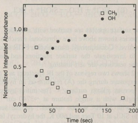
Figure 8. Normalized integrated absorbances of the AlO–H and AlC–H 3 stretching vibrations versus time during a 0.01 Torr of H 2 O exposure on porous alumina membranes at 500 K. The reduction of the AlC–H stretching vibration at \sim 2900 cm -1 is concurrent with the growth of the AlO–H stretching vibration at \sim 3500 cm -1 .
