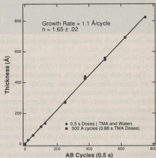
Figure 12. Thickness of Al 2 O 3 films deposited on Si(100) versus number of AB reaction cycles performed with (A) and (B) exposure times of 0.5 s at 450 K.
