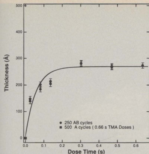
Figure 10. Thickness of Al 2 O 3 films deposited on Si(100) after 250 AB cycles at 450 K versus (A) and (B) exposure time. The film thicknesses were measured using ellipsometry.
