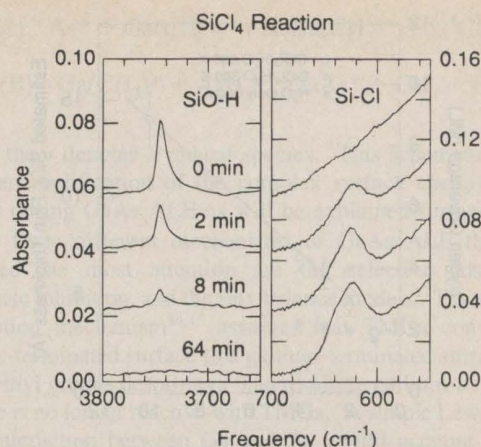
Figure 2. FTIR spectra during the SiCl 4 reaction at 600 K and 10 Torr on a hydroxylated oxidized porous silicon surface. The reduction of the SiO-H stretching vibration at ~3740 cm -1 is concurrent with the growth of the Si-Cl stretching vibration at ~625 cm -1 .
