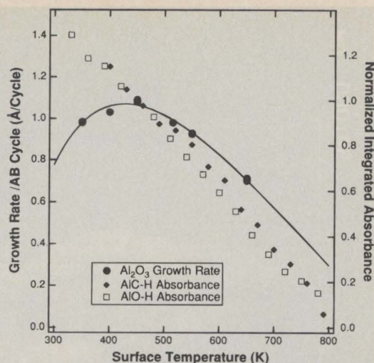
Figure 11. Al 2 O 3 growth rate per AB reaction cycle as a function of surface temperature. These growth rates were determined by ellipsometry using Al 2 O 3 film thicknesses measured after 250 AB reaction cycles. The thermal stabilities of the hydroxyl and methyl surface species are shown for comparison. These coverages were measured using the integrated absorbances of the AlO–H and AlC–H stretching vibrations.
