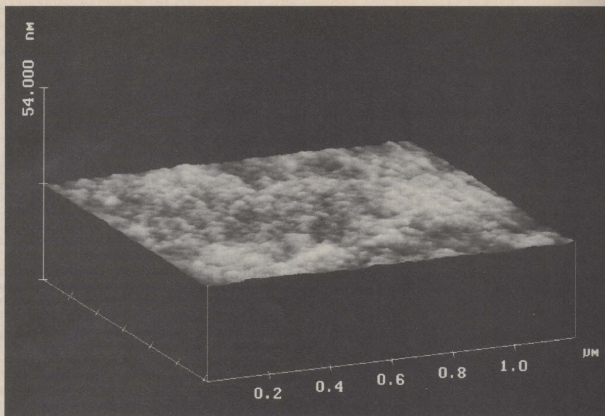
Figure 13. Atomic force microscope image of a \text{Al}_2\text{O}_3 film deposited on Si(100) after 250 AB cycles with (A) and (B) exposure times of 0.5 s at 450 K.
