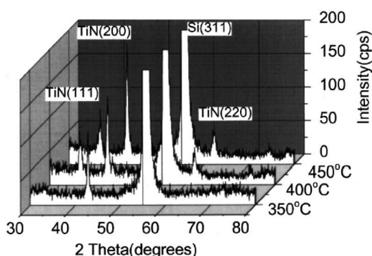
FIG. 15. X-ray diffractograms of TiN films deposited from \text{TiCl}_4 and \text{NH}_3 at 1000 ALD cycles at temperatures 350 , 400 , and 450^\circ\text{C} . Reprinted with permission from H. Jeon, J.-W. Lee, Y.-D. Kim, D.-S. Kim, and K.-S. Yi, J. Vac. Sci. Technol. A 18 , 1595 (2000). Copyright 2000 American Vacuum Society.
