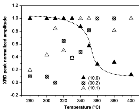
FIG. 13. Relative ratio of XRD peak intensities of ZnO films as a function of temperature deposited from zinc acetate and water. 1285 Reprinted with permission from A. Wójcik, M. Godlewski, E. Guziewicz, R. Minikayev, and W. Paszkowicz, J. Cryst. Growth 310 , 284 (2008). Copyright 2008 Elsevier.
