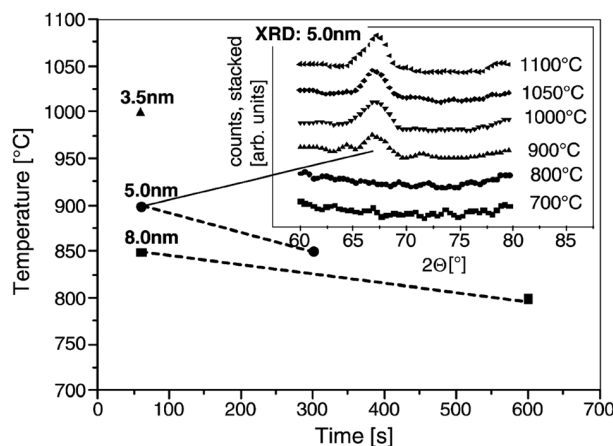
FIG. 9. First appearance of long-range order in \text{Al}_2\text{O}_3 films, as detected by XRD. The inset shows XRD spectra for 5 nm \text{Al}_2\text{O}_3 layers annealed for 60 s at different temperatures. Reprinted with permission from S. Jakschik, U. Schroeder, T. Hecht, M. Gutsche, H. Seidl, and J. W. Bartha, Thin Solid Films 425 , 216 (2003). Copyright 2003 Elsevier.
