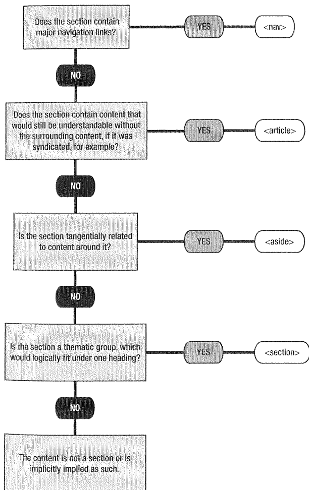
Figure 3-3. Flowchart for choosing a particular sectioning content element
