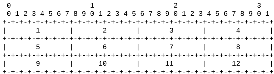
Transmission Order of Bytes
