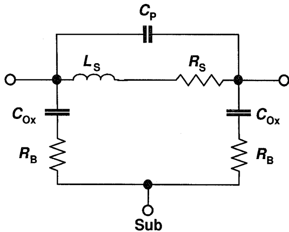
Fig. 6 Lumped-element model of the inductors
