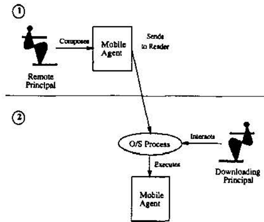
Figure 1: Mobile agent architecture
