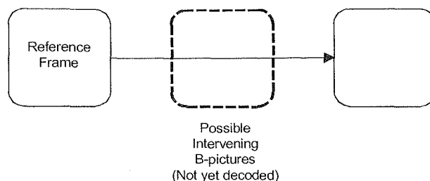
Figure 7-10 – Frame-prediction for I-pictures and P-pictures
