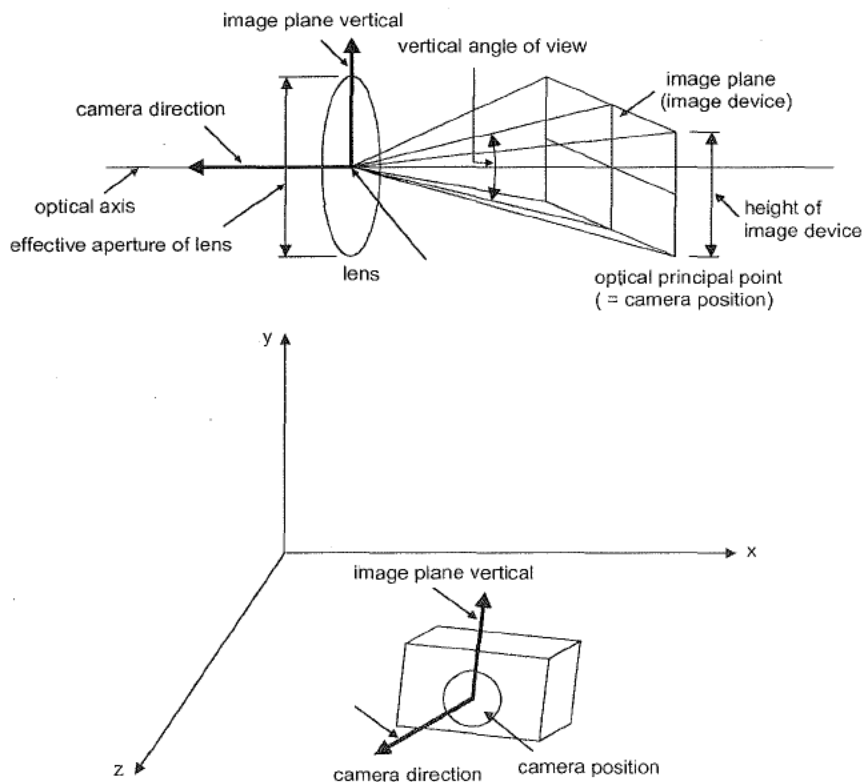
Figure 6-17 -- Camera parameters
