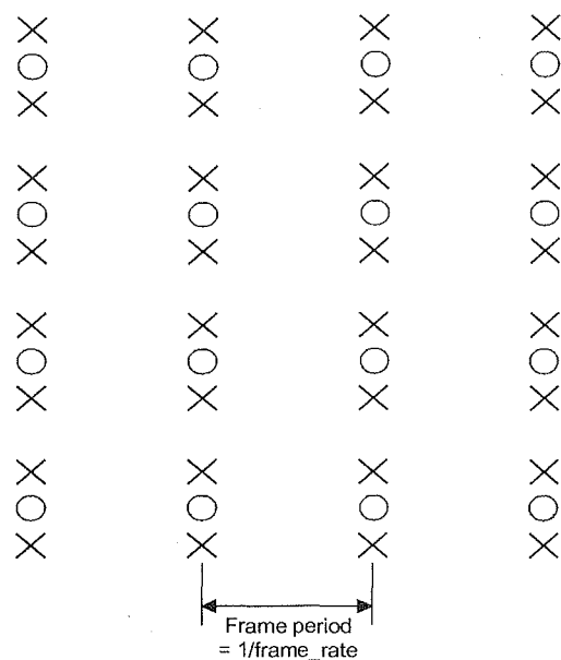
Figure 7-18 – progressive_sequence == 1
