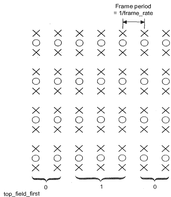
Figure 7-19 – progressive_sequence == '1'; repeat_first_field == '1'
