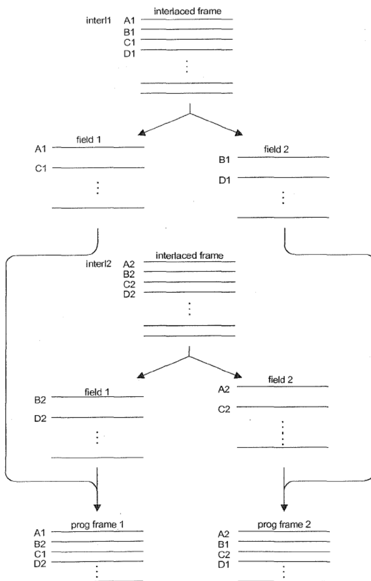
Figure D.4 – Two-interlace to progressive conversion
