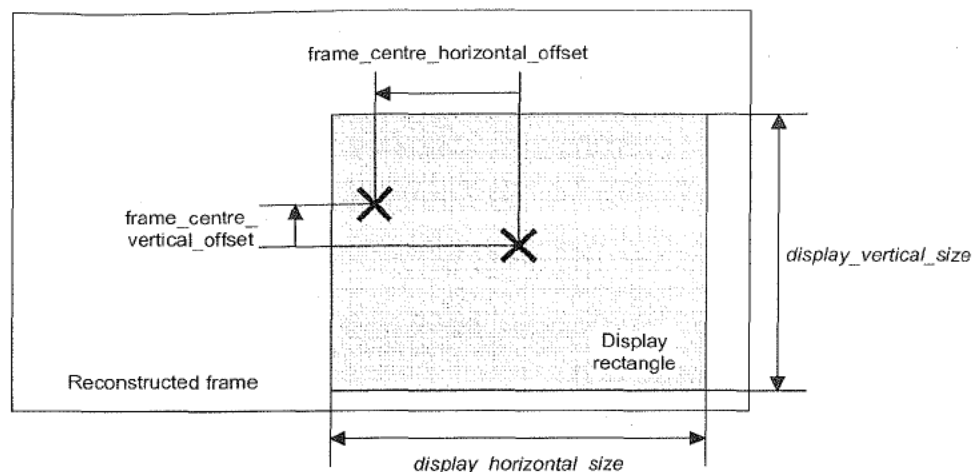
Figure 6-16 – Frame centre offset parameters
