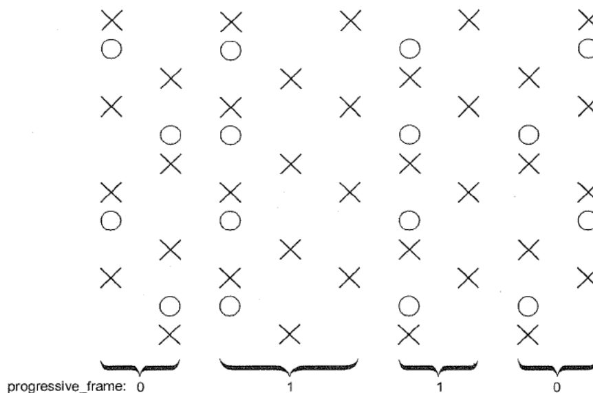
Figure 7-21 – progressive_sequence == 0 with 4:2:0 chrominance
