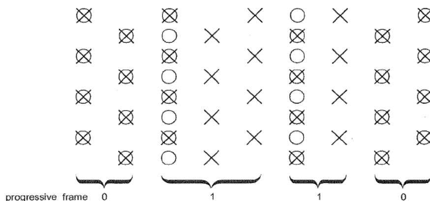
Figure 7-22 – progressive_sequence == 0 with 4:2:2 or 4:4:4 chrominance
