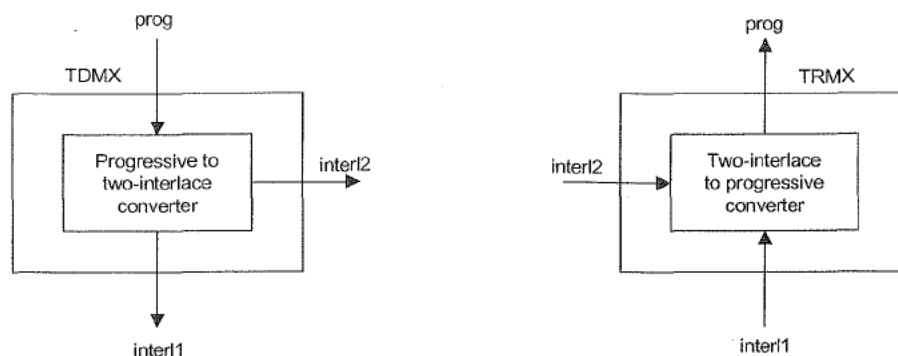
Figure D.5 – Temporal demultiplexer and remultiplexer for progressive – Interface-to-interface temporal scalability
