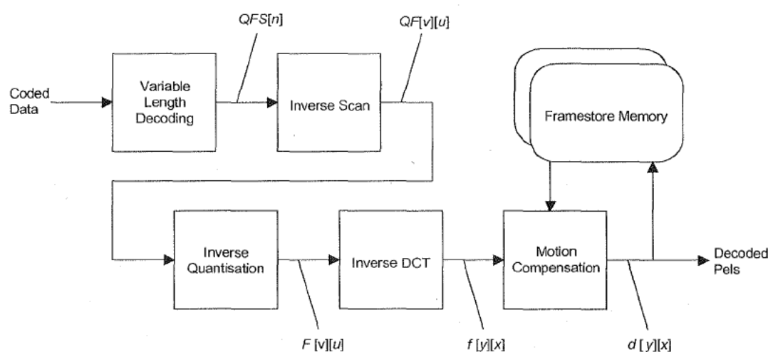
Figure 7-1 – Simplified Video Decoding Process
