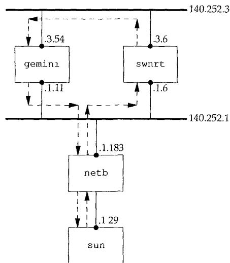
Figure 25.29 Topology of systems being used for example.
