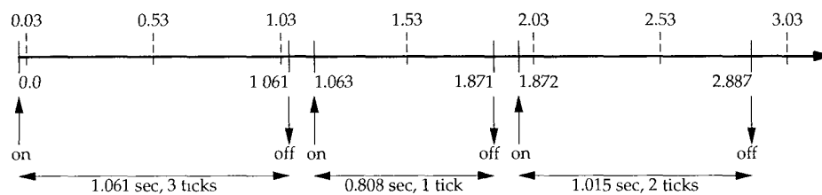
Figure 21.3 RTT measurements and clock ticks.
