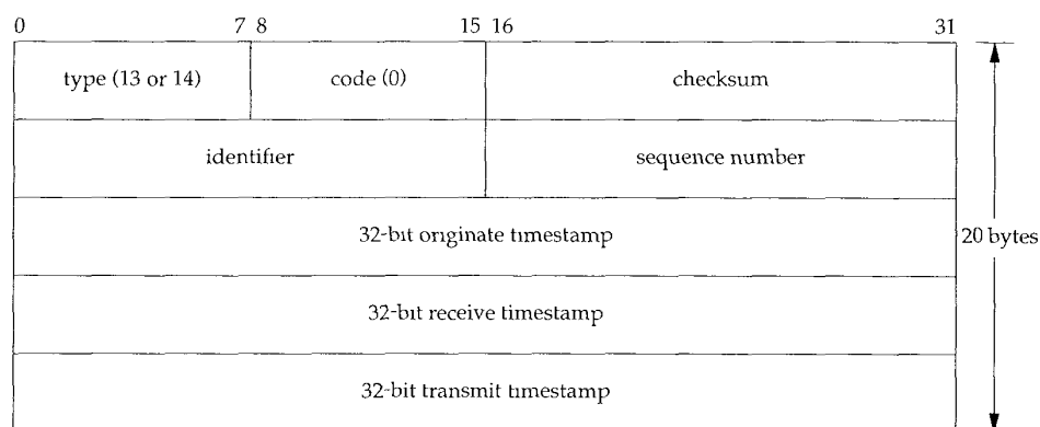
Figure 6.6 ICMP timestamp request and reply messages.
