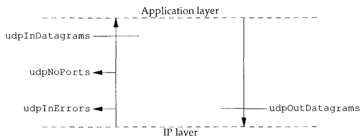
Figure 25.10 Case Diagram for UDP group.
