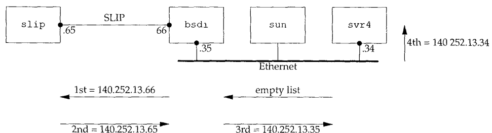
Figure 7.4 ping with record route option.
