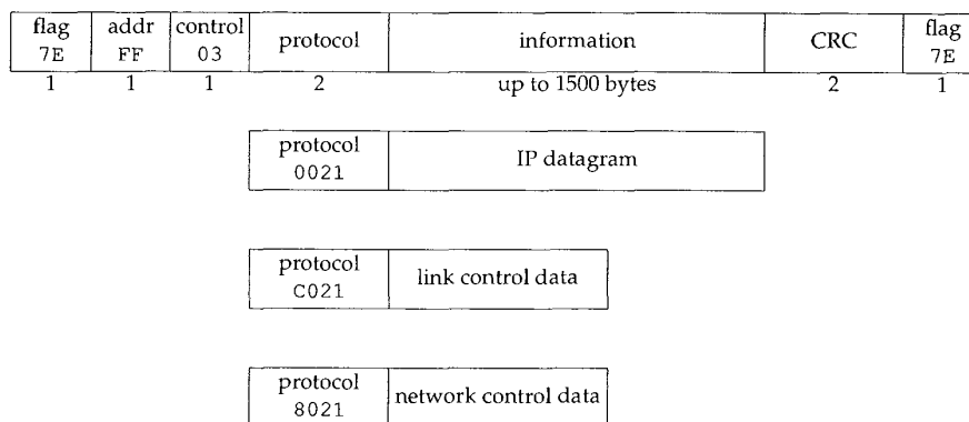
Figure 2.3 Format of PPP frames.
