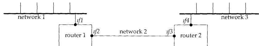
Figure 8.3 Identification of interfaces printed by traceroute.
