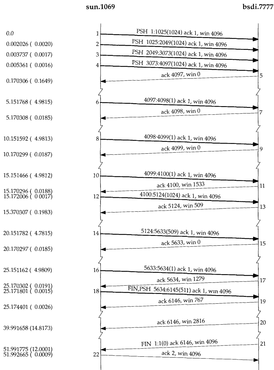
Figure 22.2 Time line showing receiver avoidance of silly window syndrome.
