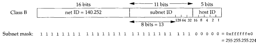
Figure 3.11 Using variable-length subnets.
