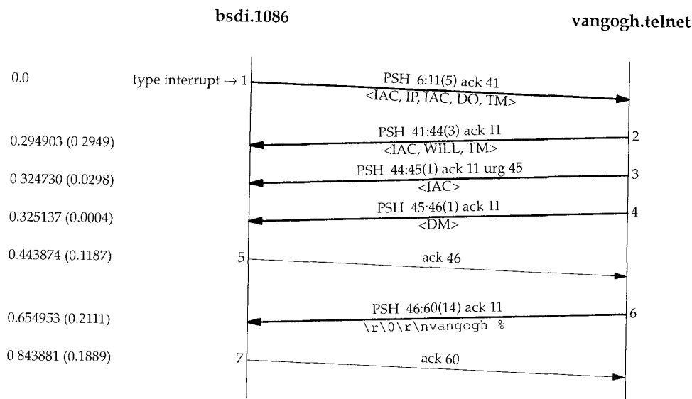
Figure 26.17 Typing interrupt key during linemode operation.
