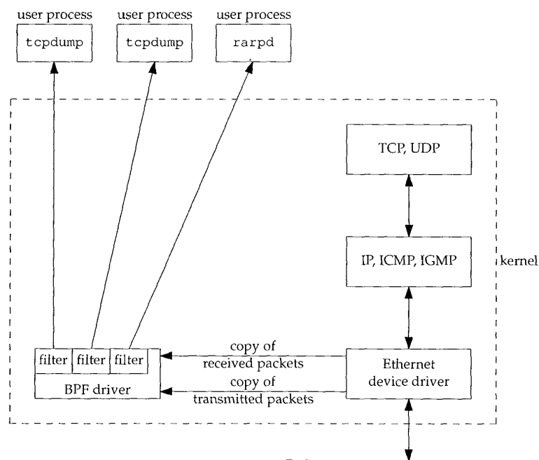
Figure A.1 BSD Packet Filter.
