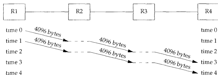
Figure 24.3 Sending two 4096-byte packets through four routers.
