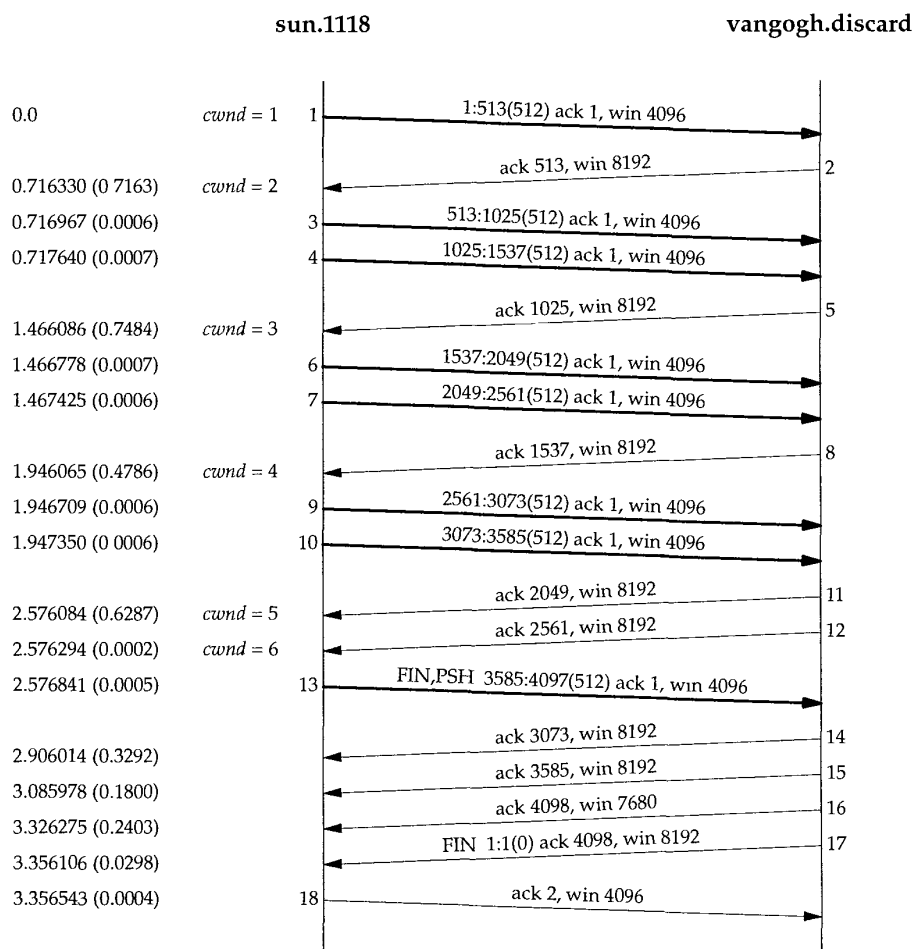
Figure 20.8 Example of slow start.
