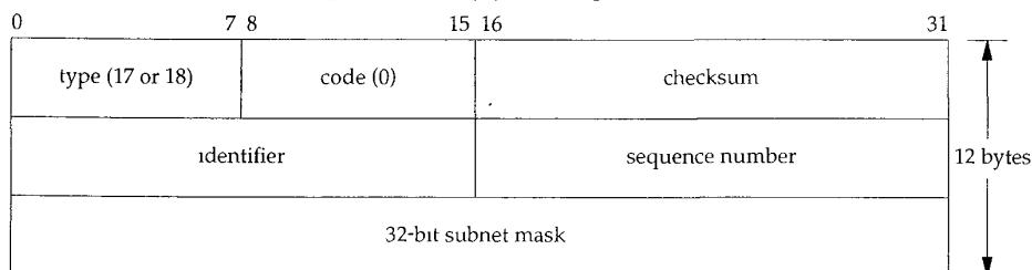
Figure 6.4 ICMP address mask request and reply messages.
