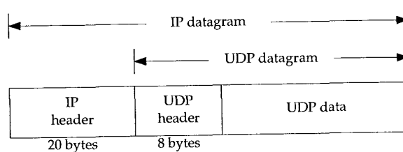
Figure 11.1 UDP encapsulation.
