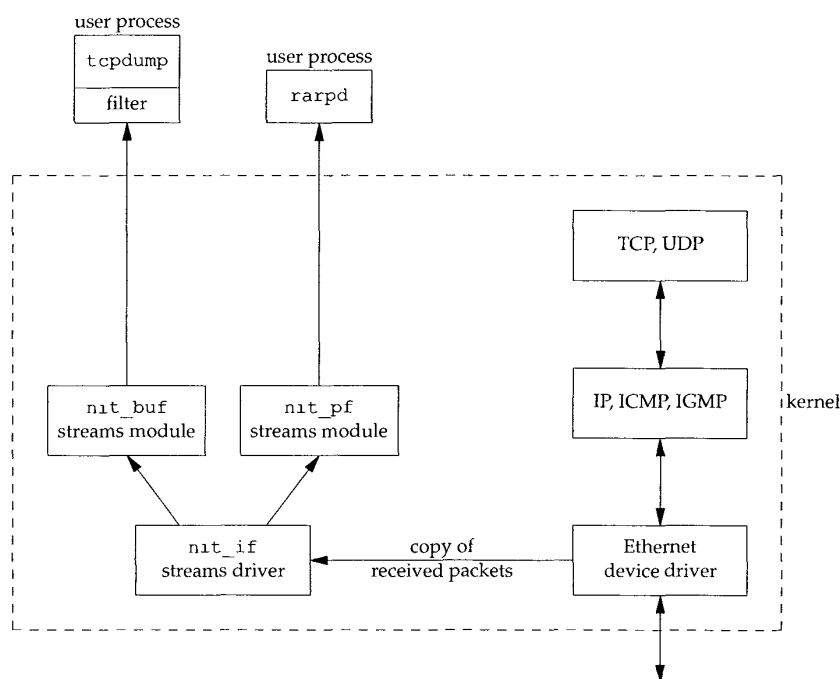
Figure A.2 SunOS Network Interface Tap.
