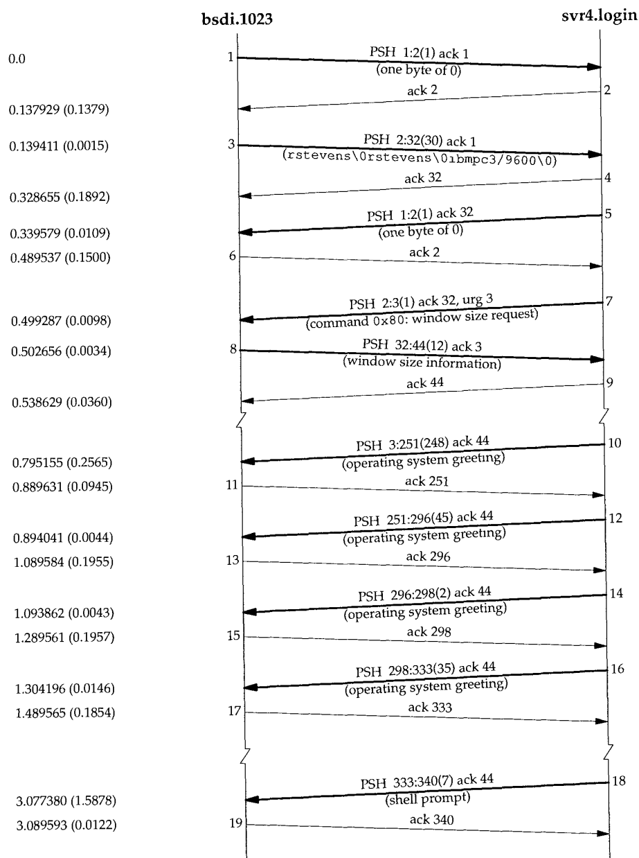
Figure 26.5 Time line for an Rlogin connection.
