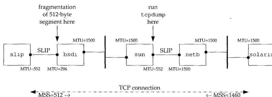
Figure 24.1 Topology for path MTU example.
