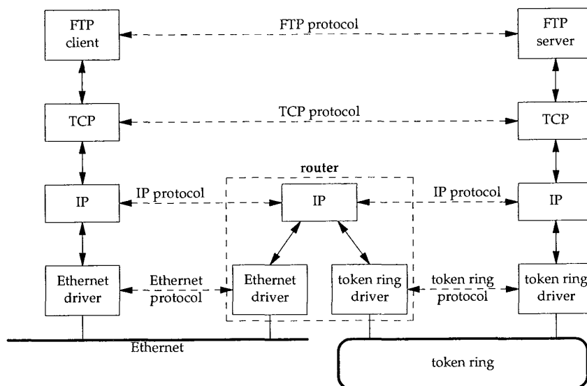
Figure 1.3 Two networks connected with a router.
