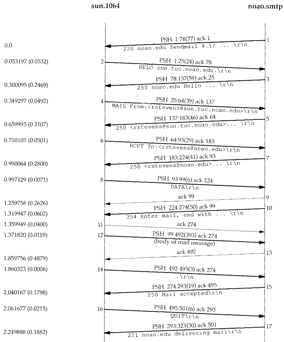
Figure 28.2 Basic SMTP mail delivery
