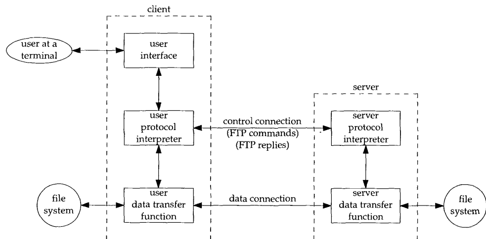
Figure 27.1 Processes involved in file transfer.
