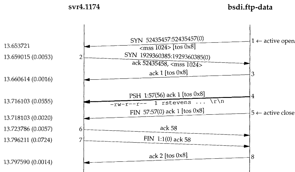
Figure 27.7 Data connection for FTP example.
