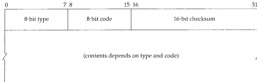
Figure 6.2 ICMP message.
