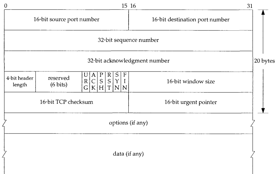
Figure 17.2 TCP header.
