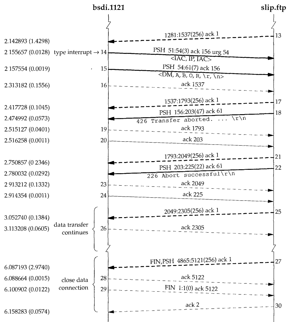
Figure 27.10 Aborting a file transfer (second half).
