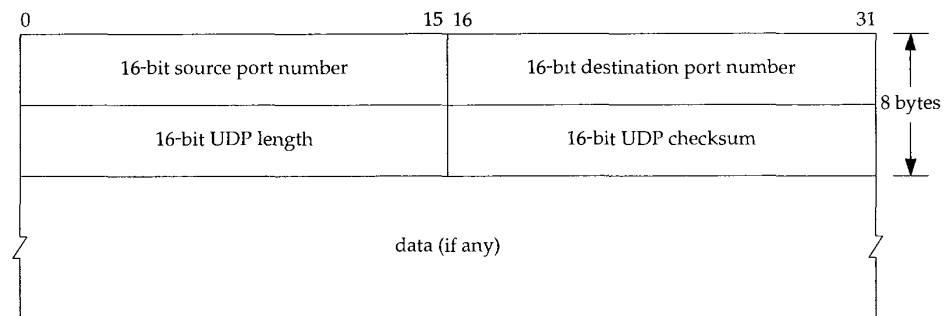
Figure 11.2 UDP header.
