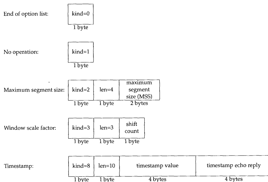
Figure 18.20 TCP options.
