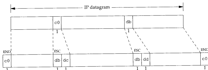
Figure 2.2 SLIP encapsulation.
