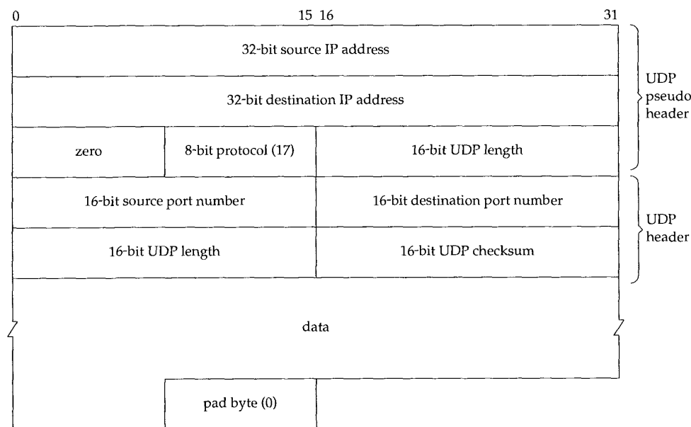
Figure 11.3 Fields used for computation of UDP checksum.
