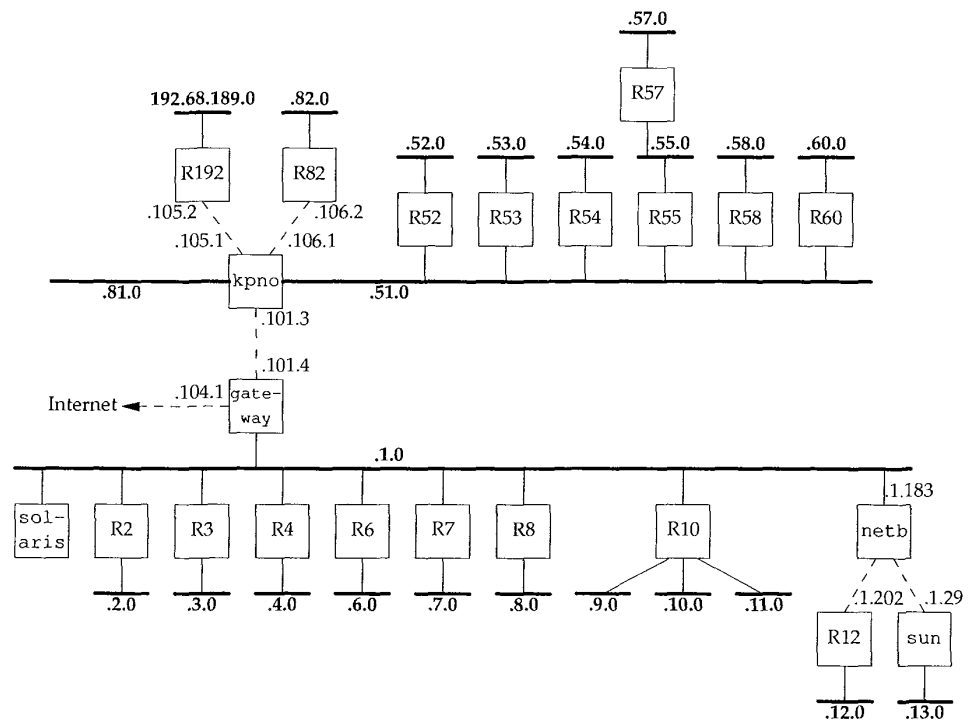
Figure 10.7 Many of the noao.edu 140.252 networks.
