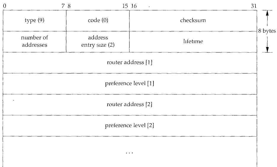
Figure 9.7 Format of ICMP router advertisement message.
