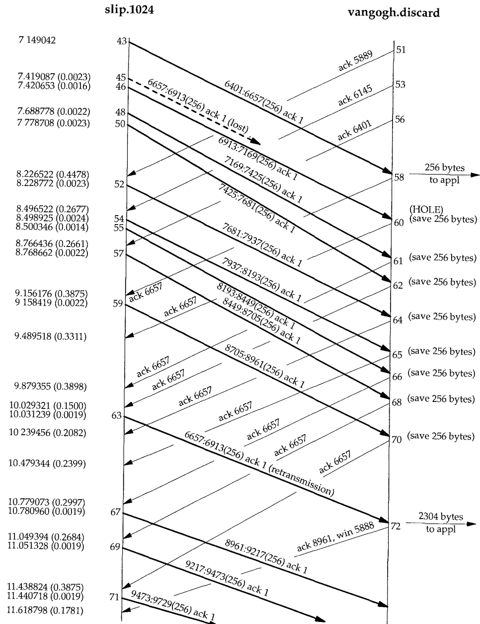
Figure 21.7 Packet exchange for retransmission around the 10-second mark.
