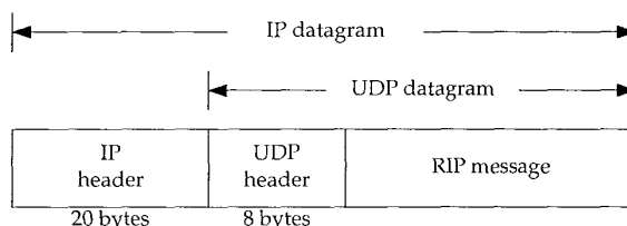
Figure 10.2 RIP message encapsulated within a UDP datagram.
