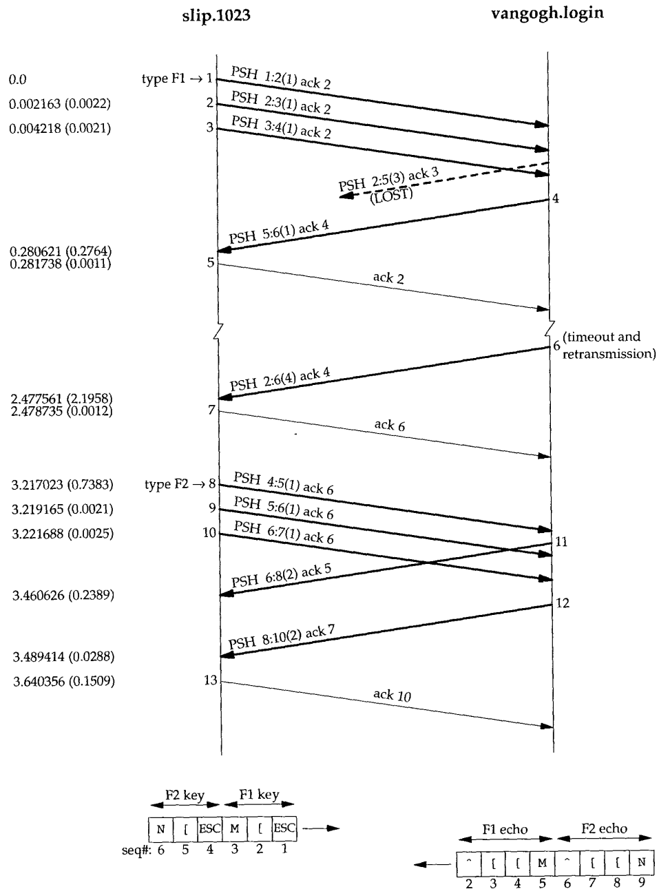
Figure 19.8 Time line for Figure 19.7 (Nagle algorithm disabled).
