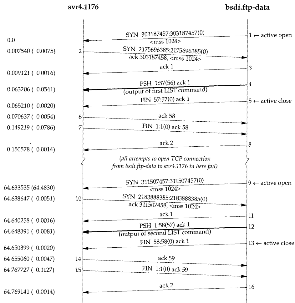
Figure 27.8 Data connection for two consecutive LIST commands.
