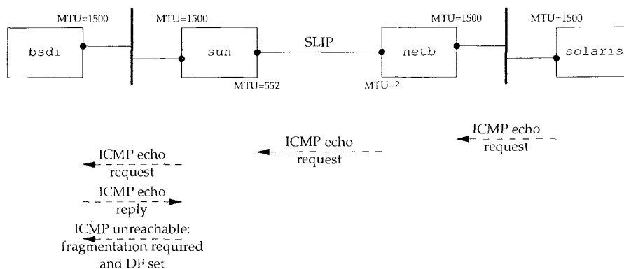
Figure 11.12 Packets exchanged in example.
