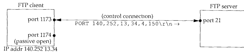
Figure 27.4 PORT command going across FTP control connection.
