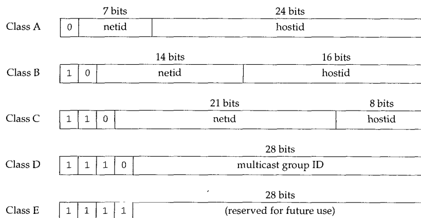
Figure 1.5 The five different classes of Internet addresses.
