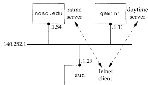
Figure 14.9 Systems being used for simple DNS example.
