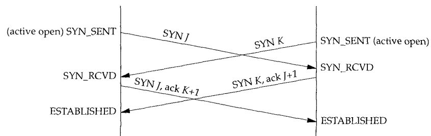
Figure 18.17 Segments exchanged during simultaneous open.
