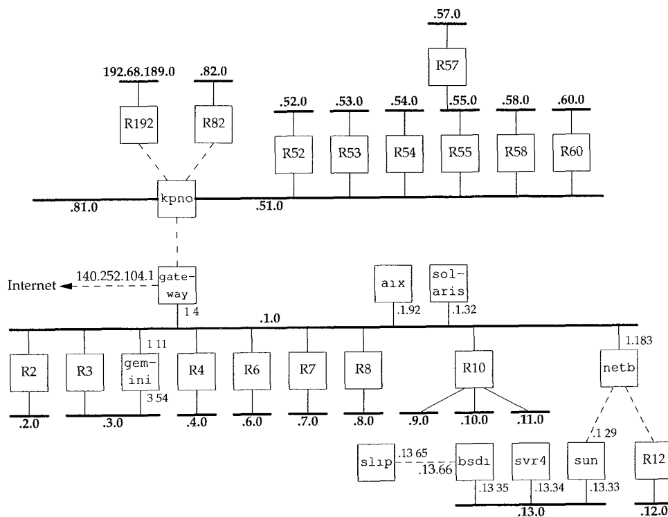
Figure 3.6 Arrangement of most of the noao.edu 140.252 subnets.
