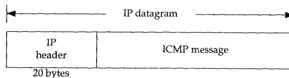
Figure 6.1 ICMP messages encapsulated within an IP datagram.
