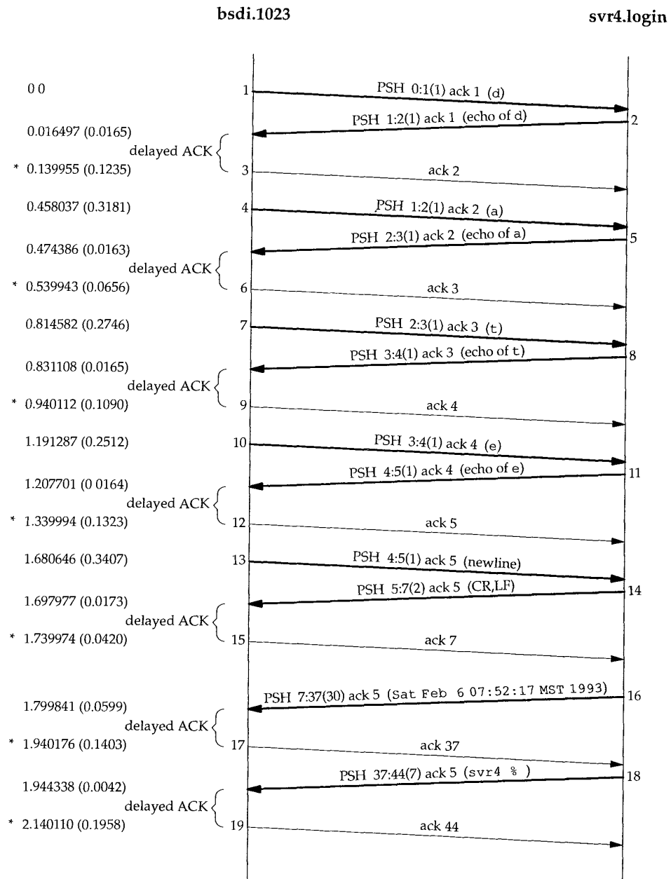
Figure 19.3 Time line of data flow for date command typed on an rlogin connection.
