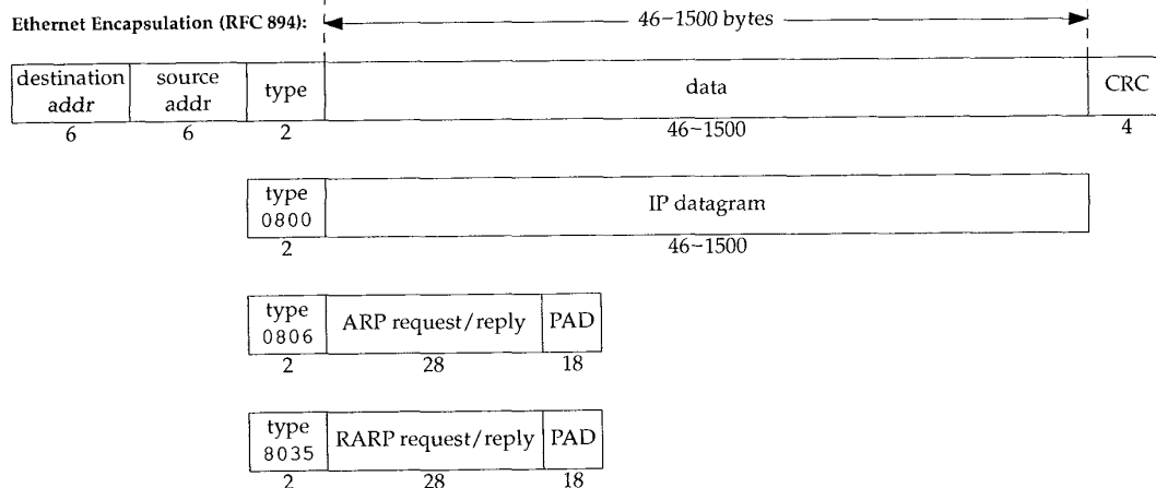
Figure 2.1 IEEE 802.2/802.3 encapsulation (RFC 1042) and Ethernet encapsulation (RFC 894).
