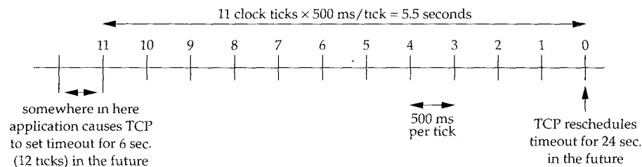
Figure 18.7 TCP 500-ms timer.
