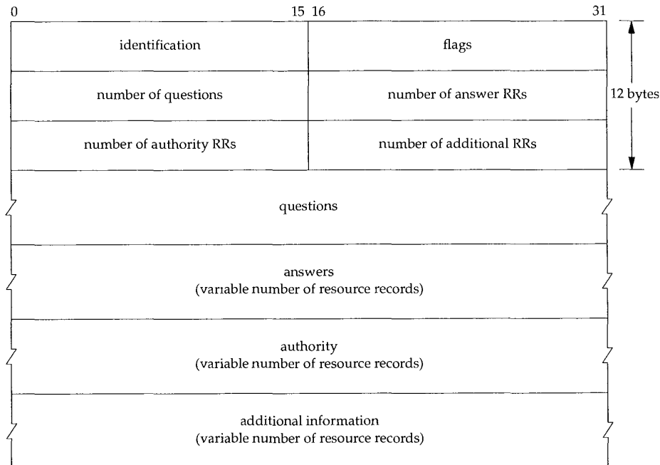
Figure 14.3 General format of DNS queries and responses.
