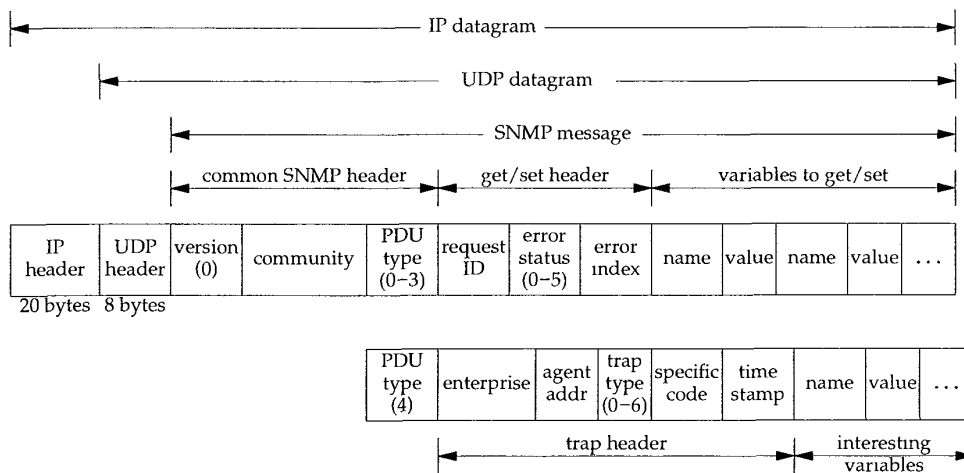
Figure 25.2 Format of the five SNMP messages.
