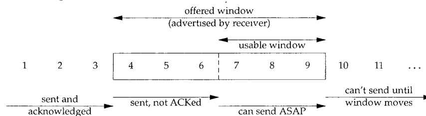
Figure 20.4 Visualization of TCP sliding window
