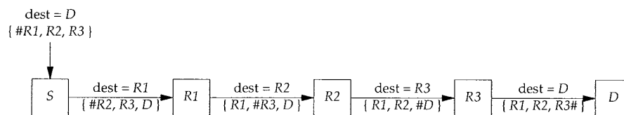
Figure 8.7 Example of IP source routing.
