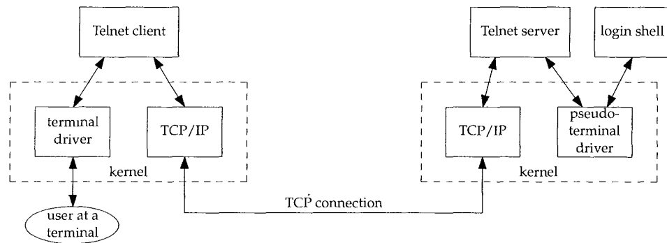
Figure 26.1 Overview of Telnet client-server.
