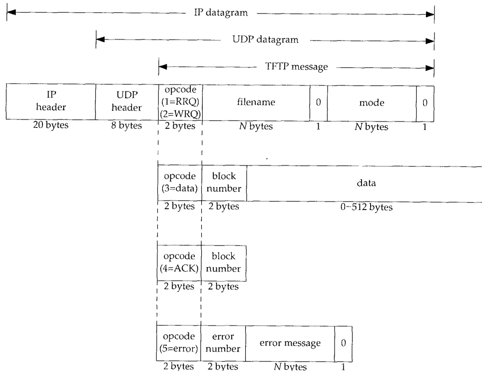
Figure 15.1 Format of the five TFTP messages.
