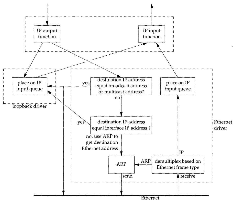
Figure 2.4 Processing of IP datagrams by loopback interface.
