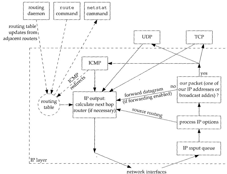
Figure 9.1 Processing done at the IP layer.
