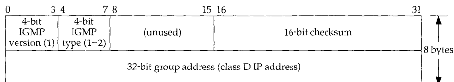
Figure 13.2 Format of fields in IGMP message.
