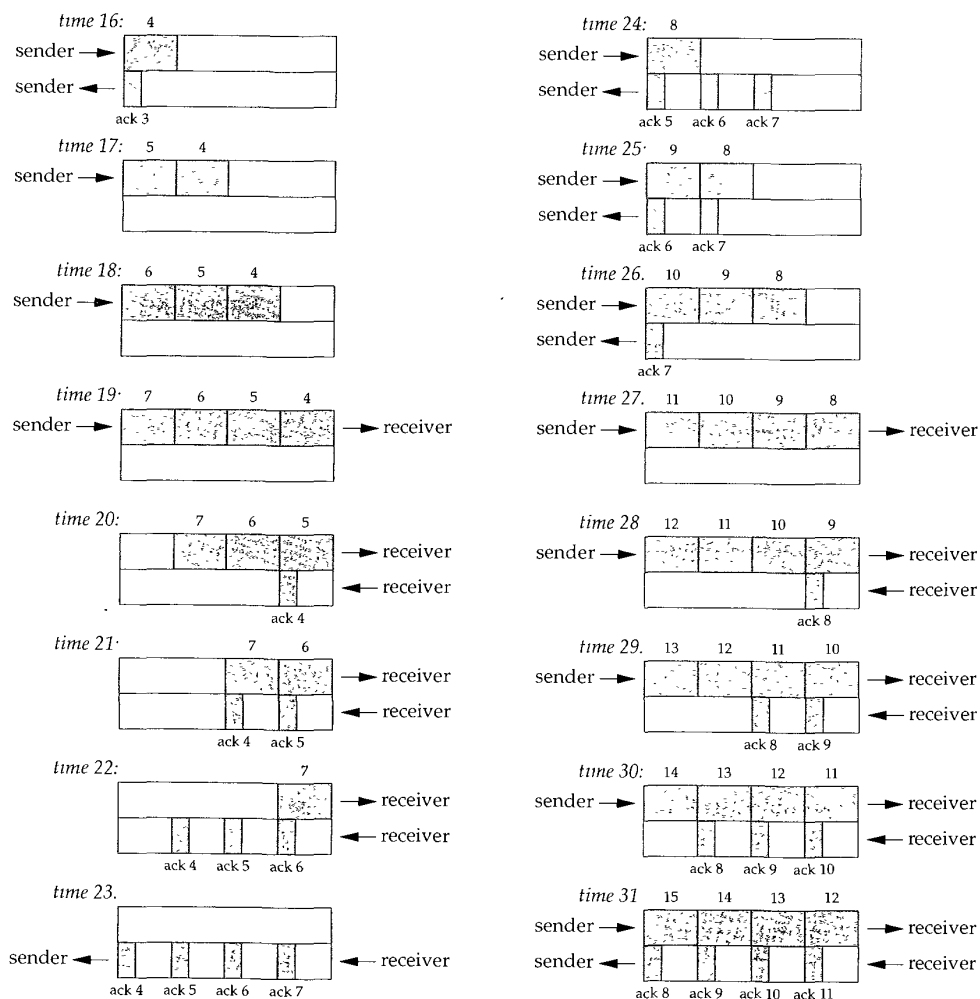
Figure 20.10 Times 16-31 for bulk data throughput example.
