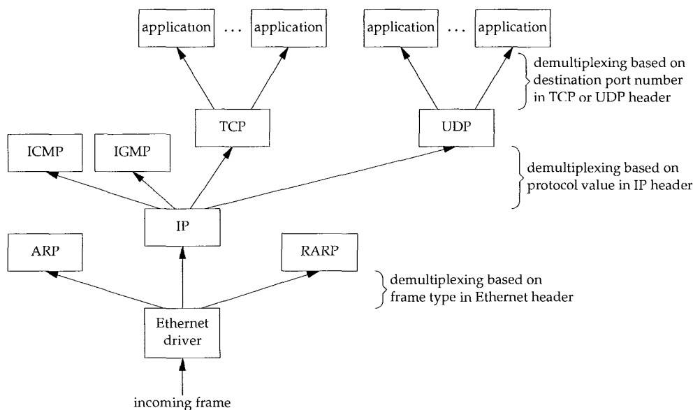
Figure 1.8 The demultiplexing of a received Ethernet frame.
