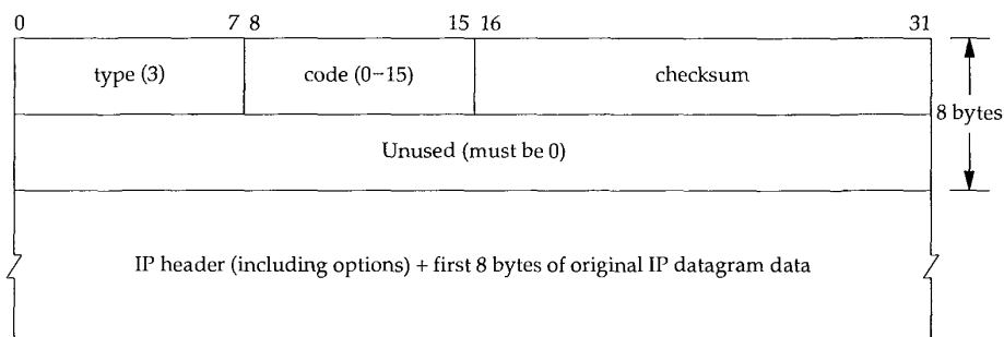
Figure 6.10 ICMP unreachable message.
