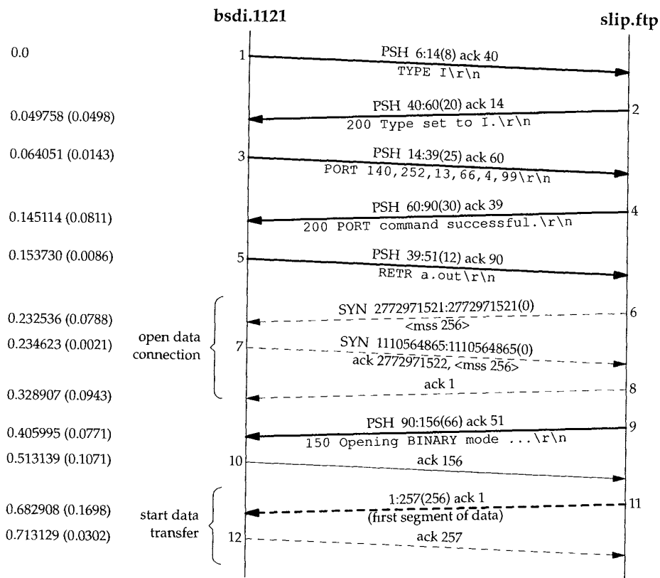
Figure 27.9 Aborting a file transfer (first half).
