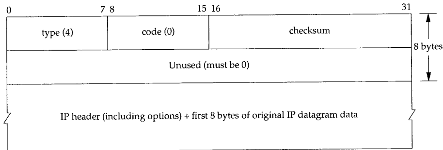
Figure 11.18 ICMP source quench error.
