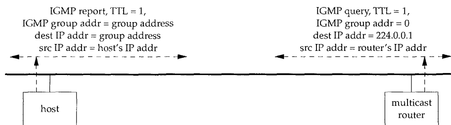
Figure 13.3 IGMP reports and queries.
