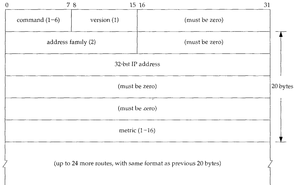
Figure 10.3 Format of a RIP message.
