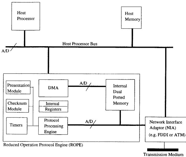
Figure 2 Block Diagram of VLSI bypass system
