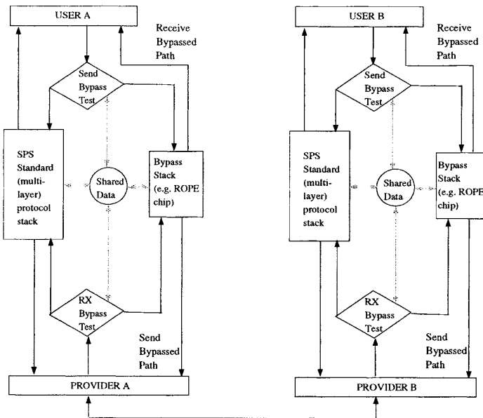
Figure 1 Bypass Architecture
