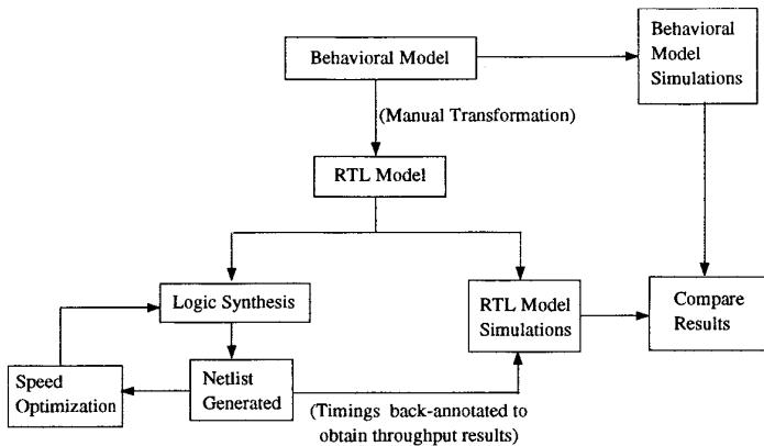
Figure 3 Design flow diagram
