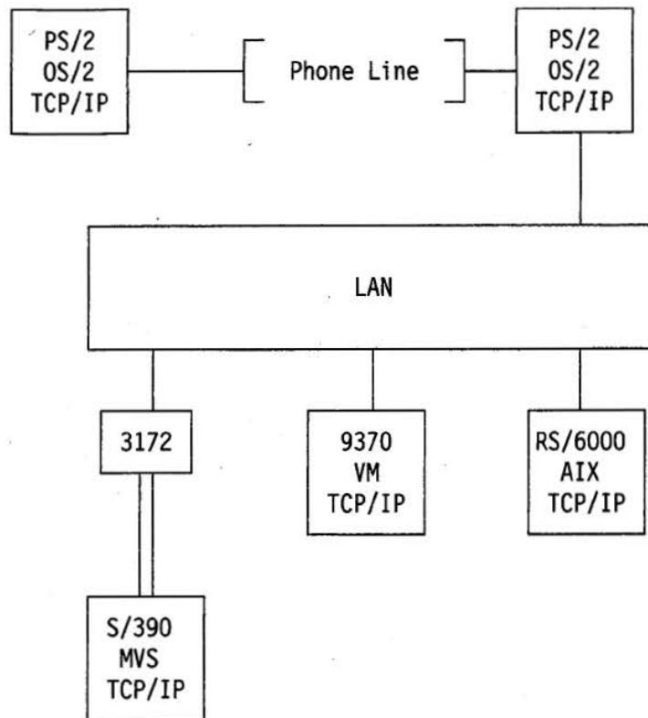
Figure 5-10. SLIP Example
