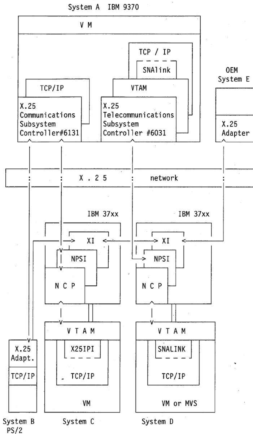
Figure 5-11. X.25 Example Scenario
