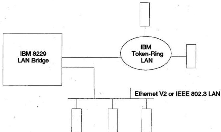
Figure 5-13. 8229 Connection Diagram
