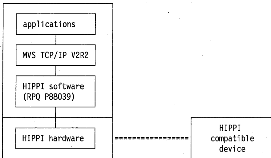
Figure 5-5. IBM HIPPI and MVS TCP/IP
