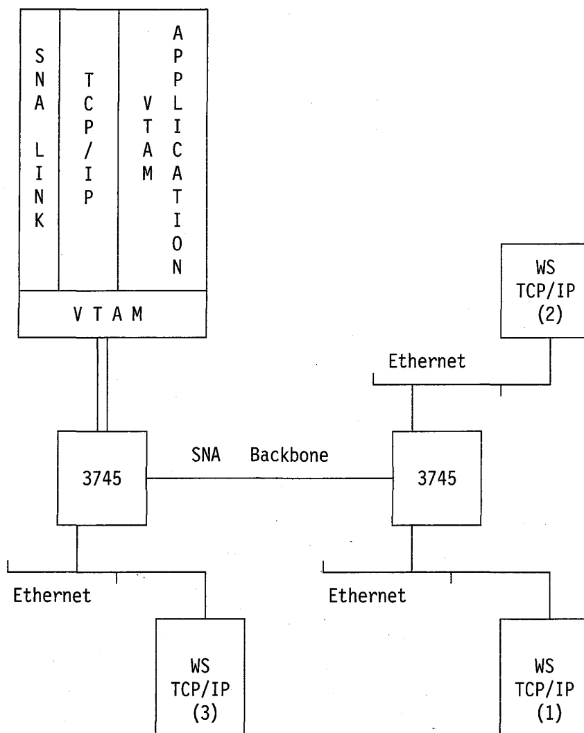
Figure 5-12. 3745 and Ethernet Adapter
