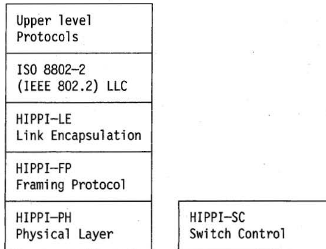
Figure 5-6. Relationship of ANSI HIPPI Draft Standards
