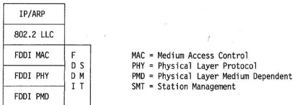
Figure 5-9. IP and ARP over FDDI
