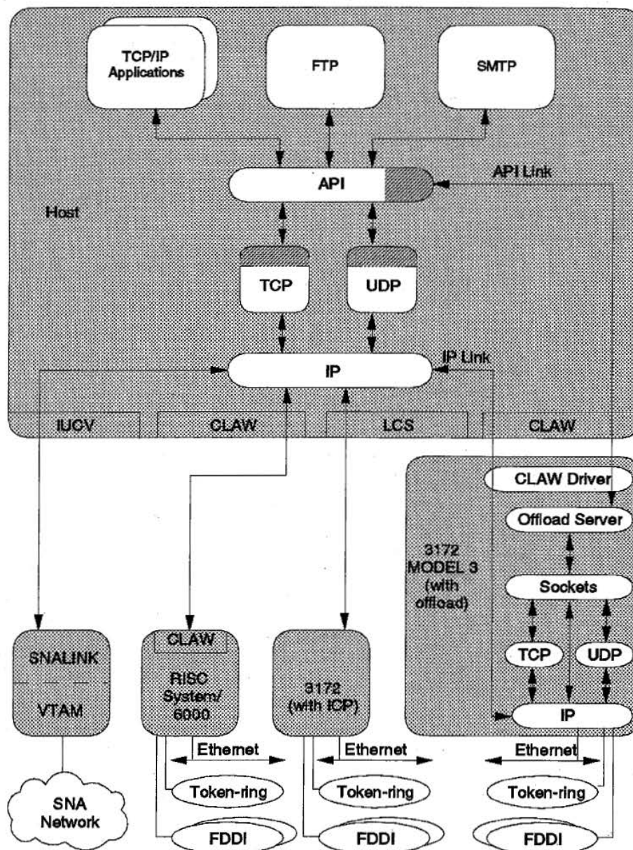
Figure 5-3. IBM 3172-3 Interconnect Controller. TCP/IP Offload Processing.
