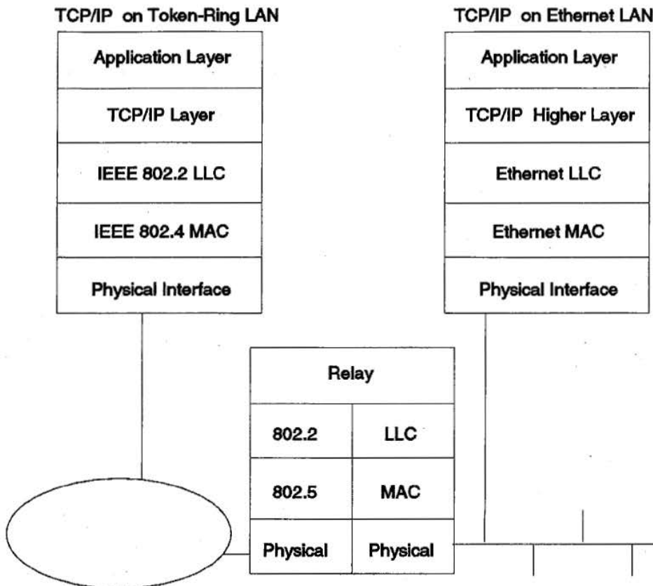
Figure 5-14. 8229 TCP/IP Support. Layered diagram.
