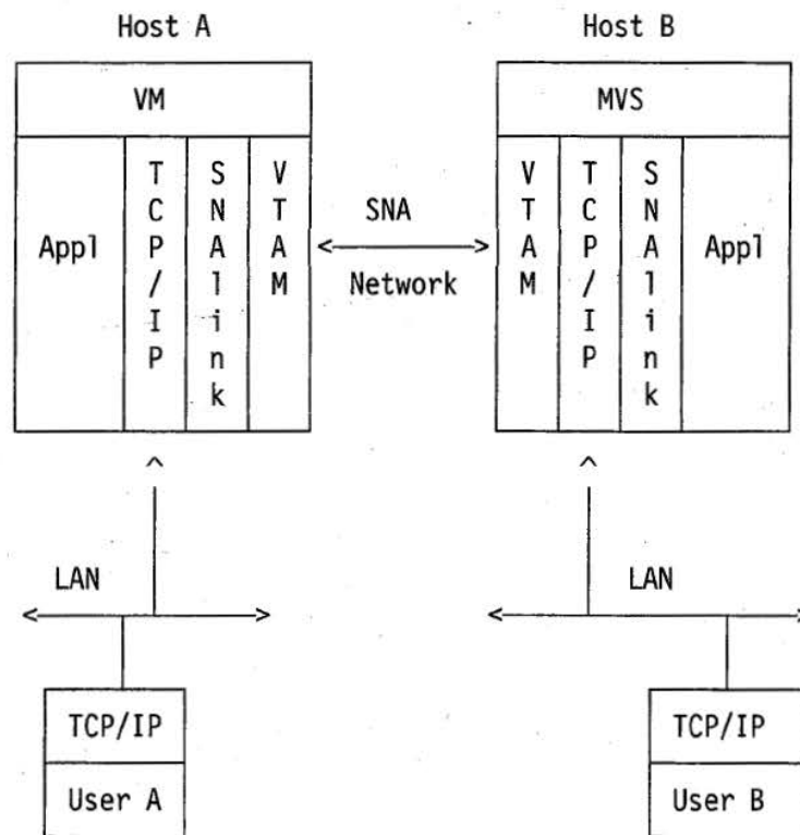
Figure 5-8. Principle of SNAlink Function
