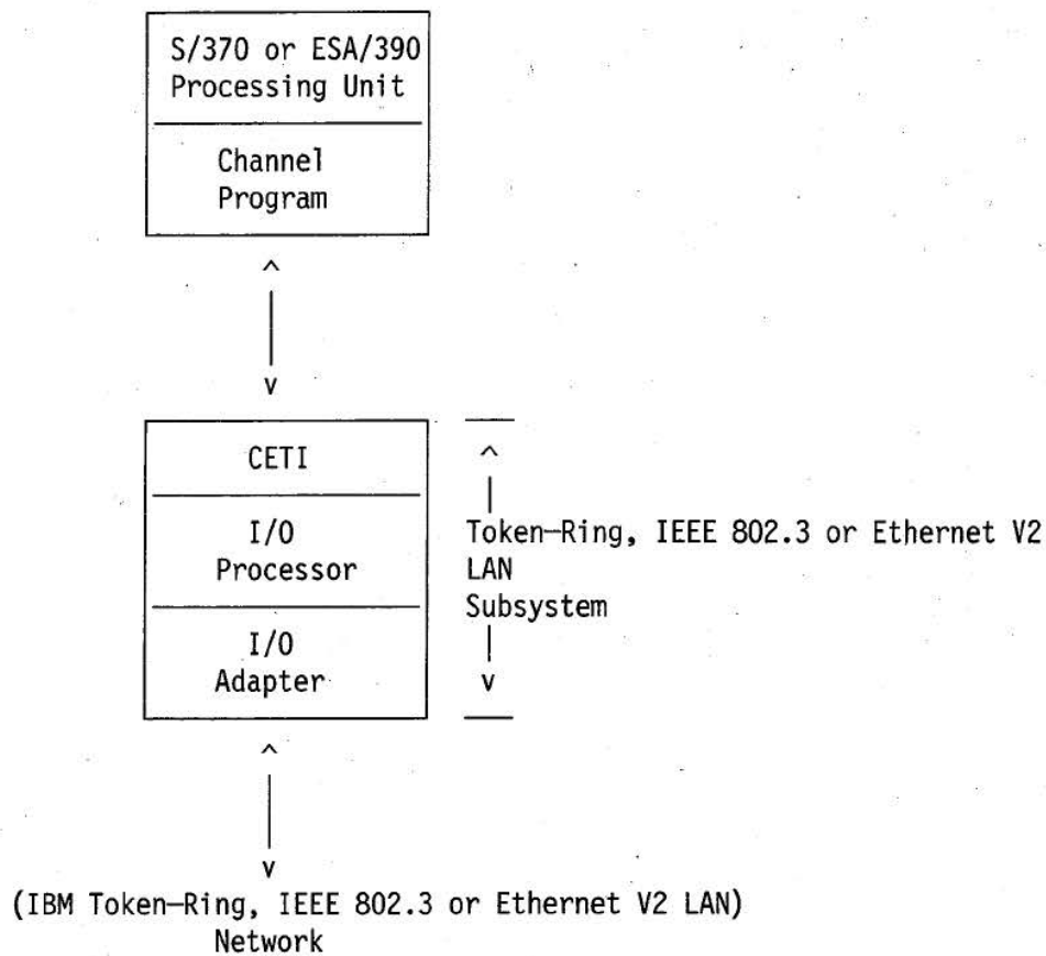
Figure 5-7. CETI Connection
