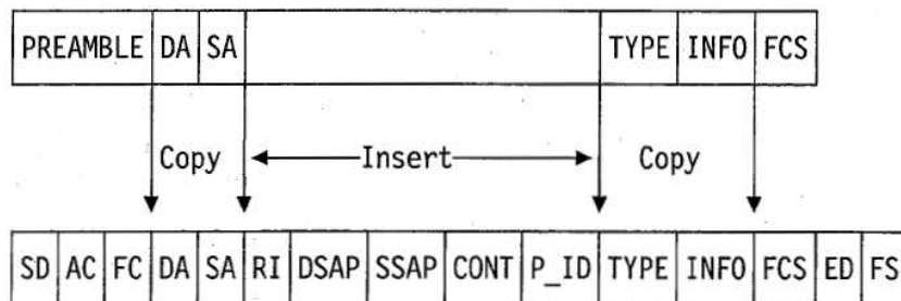
Figure 5-15. 8229 TCP/IP Support. Conversion process.
