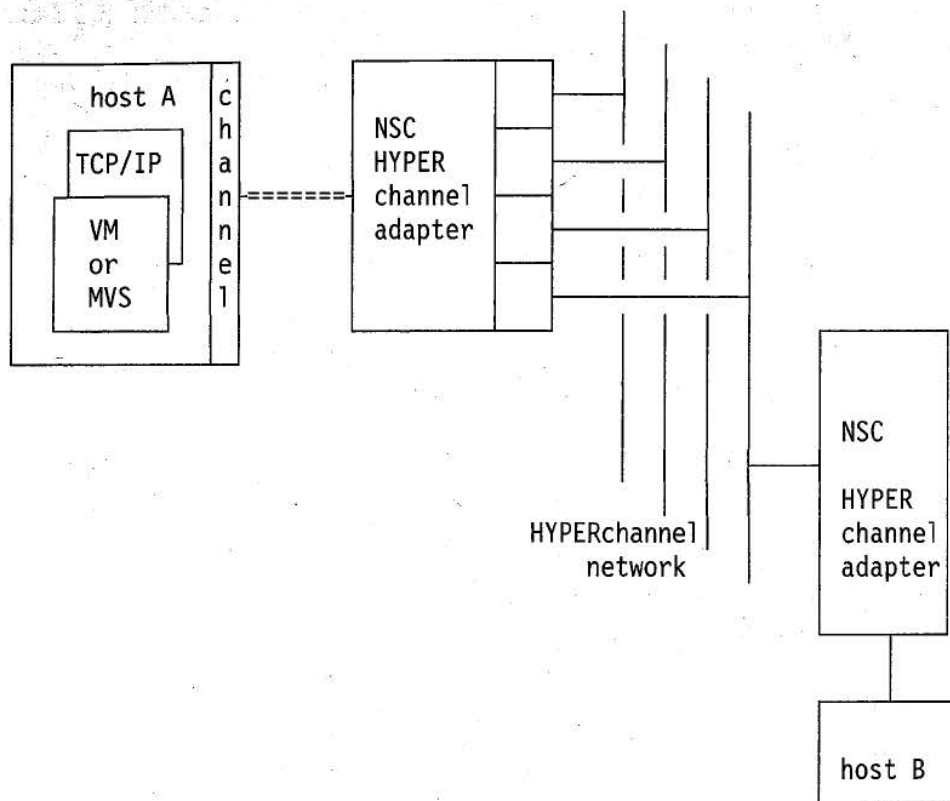
Figure 5-4. HYPERchannel Network
