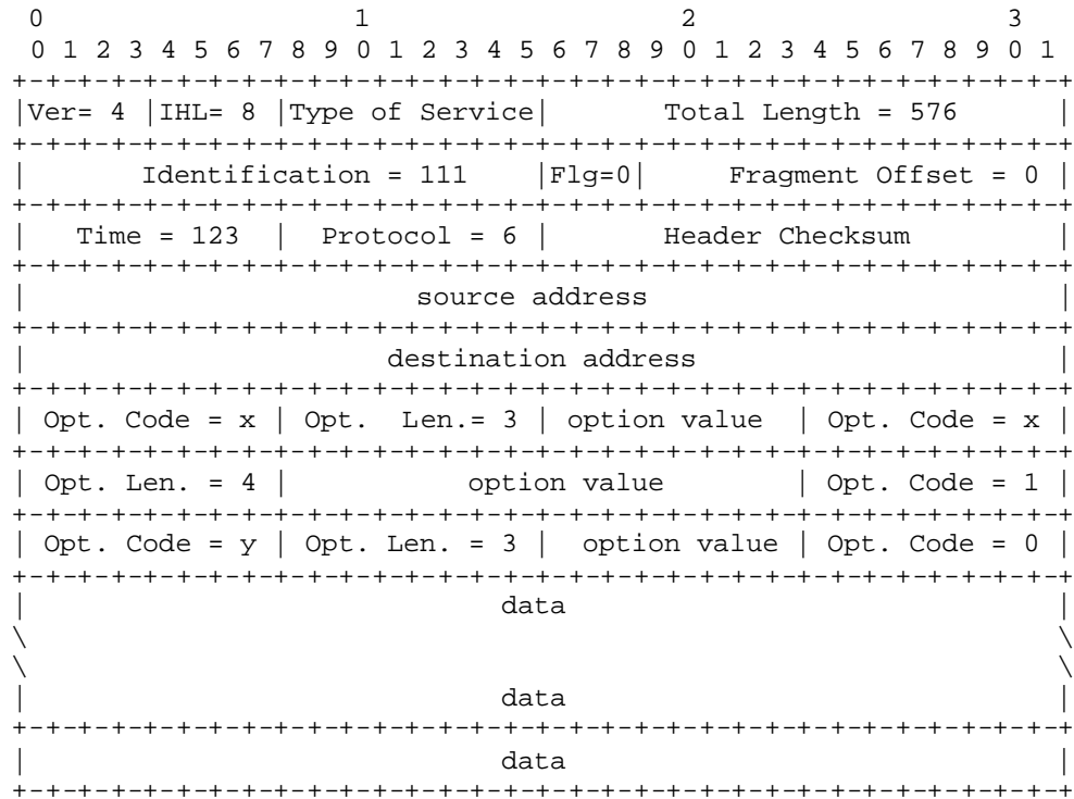
Example Internet Datagram
