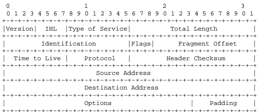
Example Internet Datagram Header
