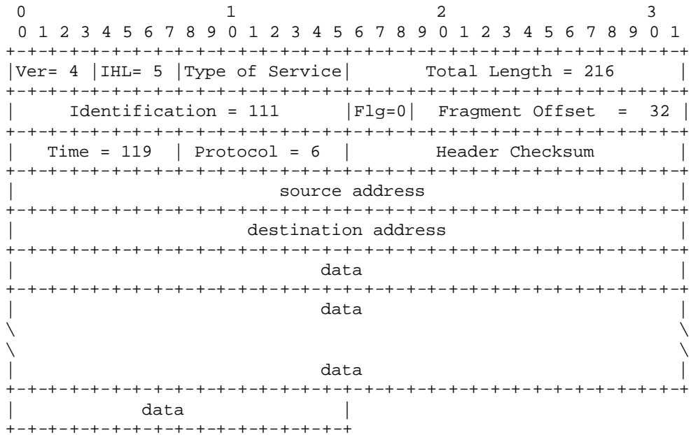
Example Internet Fragment
