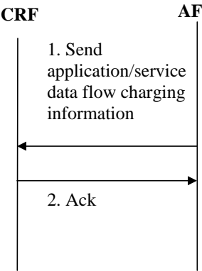
Figure 7.0a: AF input to provision of charging rules
