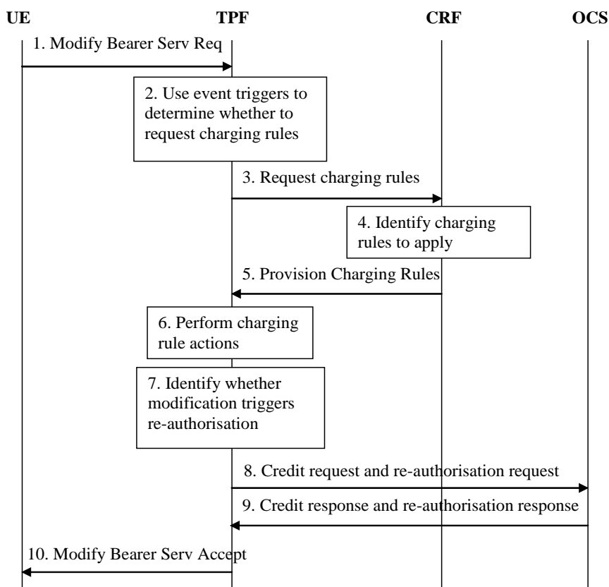
Figure 7.2c: Bearer Service Modification in case of online charging
