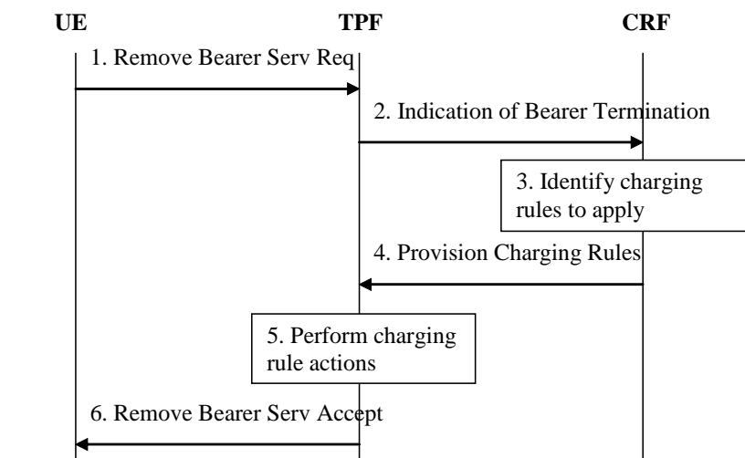
Figure 7.3: Bearer Service Termination in case of offline charging
