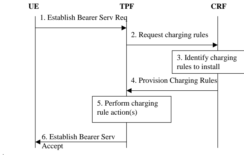
Figure 7.1: Bearer Service Establishment in case of offline charging
