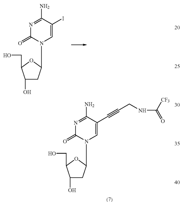
5-[3-(2,2,2-Trifluoroacetamido)-prop-1-ynyl]-2'-deoxycytidine (7)
