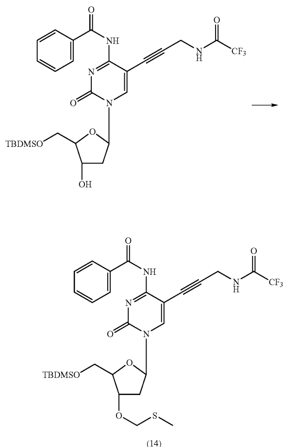
4-N-Benzoyl-5'-O-(tert-butylidimethylsilyl)-3'-O-methylthiomethyl-5-[3-(2,2,2-trifluoroacetamido)-prop-1-ynyl]-2'-deoxycytidine (14)
