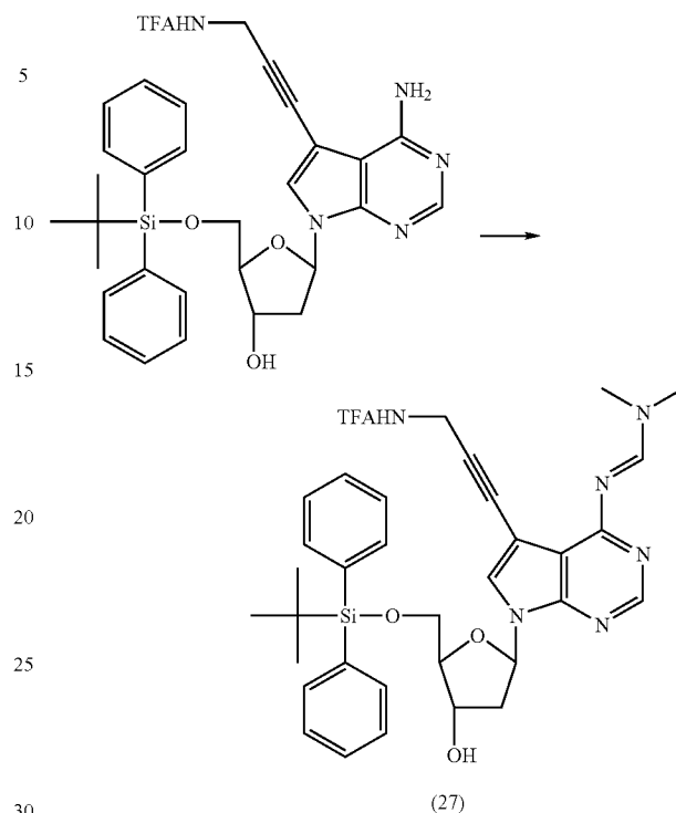
5'-O-(tert-Butyldiphenylsilyl)-7-deaza-4-N,N-dimethylformadin-7-[3-(2,2,2-trifluoroacetamido)-prop-1-ynyl]-2'-deoxyadenosine (27)
