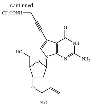
3'-O-Allyl-5'-O-(tert-butyldimethylsilyl)-7-deaza-7-[3-(2,2,2-trifluoroacetamido)-prop-1-ynyl]-2'-deoxyguanosine (47)
