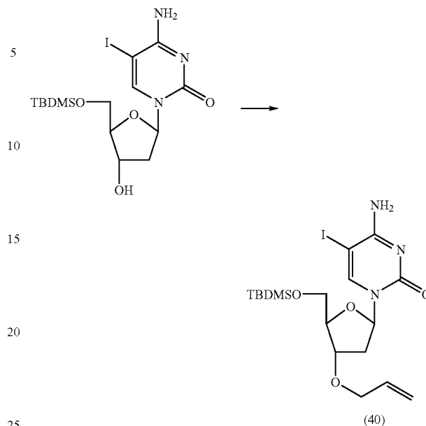
3'-O-Allyl-5'-O-(tert-butyldimethylsilyl)-5-iodo-2'-deoxycytidine (40)
