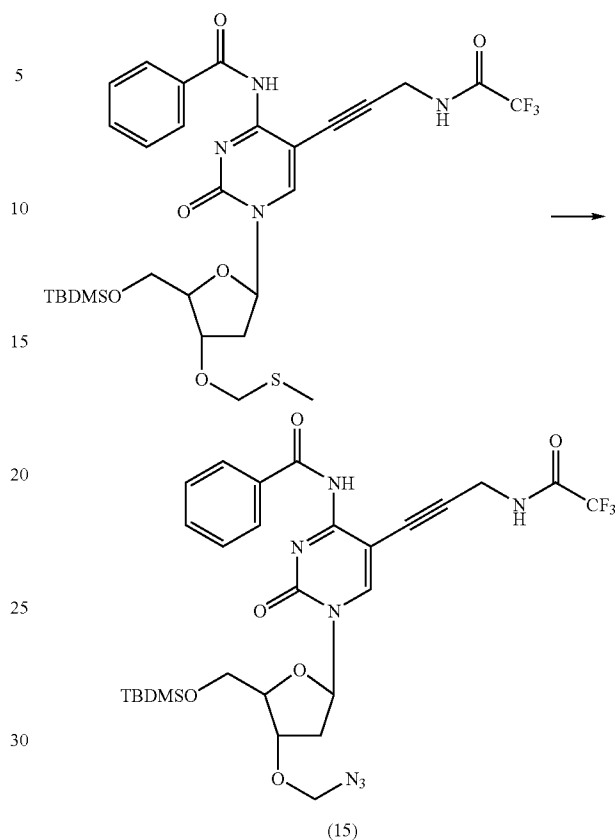
4-N-Benzoyl-5'-O-(tert-butylidimethylsilyl)-3'-O-azidomethyl-5-[3-(2,2,2-trifluoroacetamido)-prop-1-ynyl]-2'-deoxycytidine (15)
