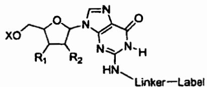
Guanosine N2-linker
