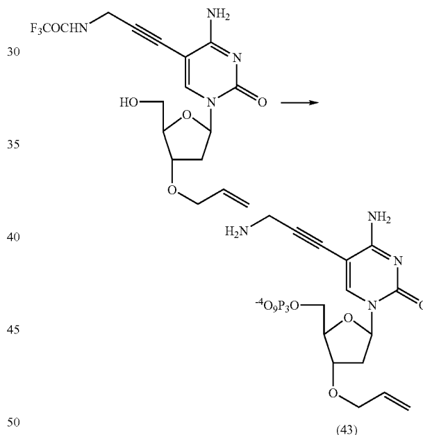
3'-O-Allyl-5-(3-amino-prop-1-ynyl)-5'-O-triphosphate-2'-deoxycytidine (43)
