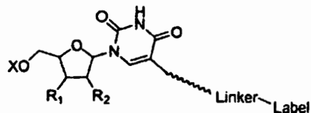
Uridine C5-linker
