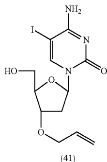
3'-O-Allyl-5-iodo-2'-deoxycytidine (41)
