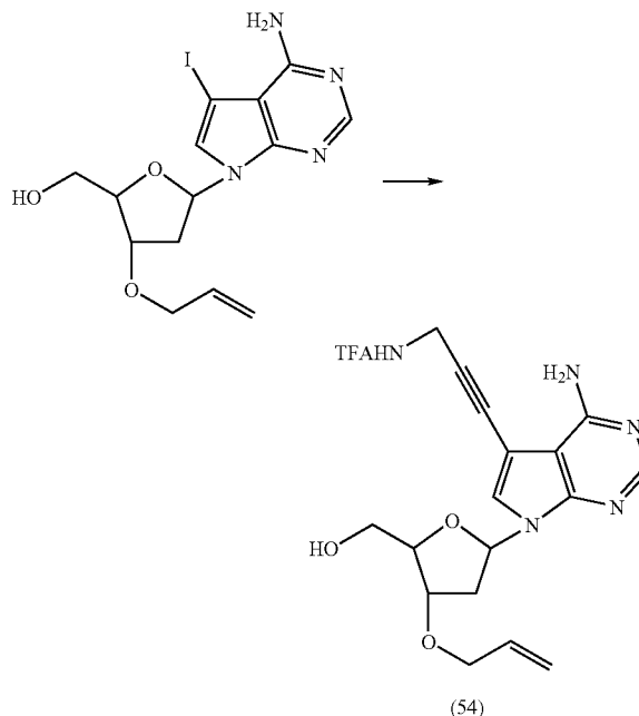
3'-O-Allyl-7-deaza-7-[3-(2,2,2-trifluoroacetamide)]-2'-deoxyadenosine (54)
