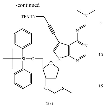
5'-O-(tert-Butyldiphenylsilyl)-7-deaza-4-N,N-dimethylformadin-3'-O-methylthiomethoxy-7-[3-(2,2,2-trifluoroacetamido)-prop-1-ynyl]-2'-deoxyadenosine (28)
