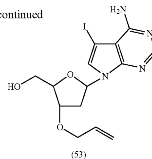
3'-O-Allyl-7-deaza-7-iodo-2'-deoxyadenosine (53)
