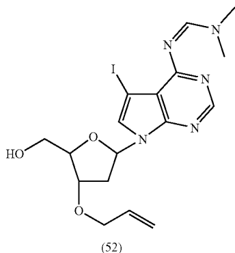
3'-O-Allyl-7-deaza-6-N,N-dimethylformidine-7-iodo-2'-deoxyadenosine (52)
