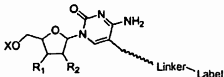
Cytidine C5-linker
