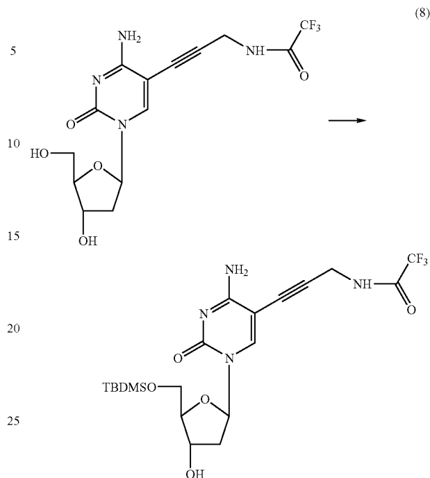
5'-O-(tert-Butyldimethylsilyl)-5-[3-(2,2,2-trifluoroacetamido)-prop-1-ynyl]-2'-deoxycytidine (8)
