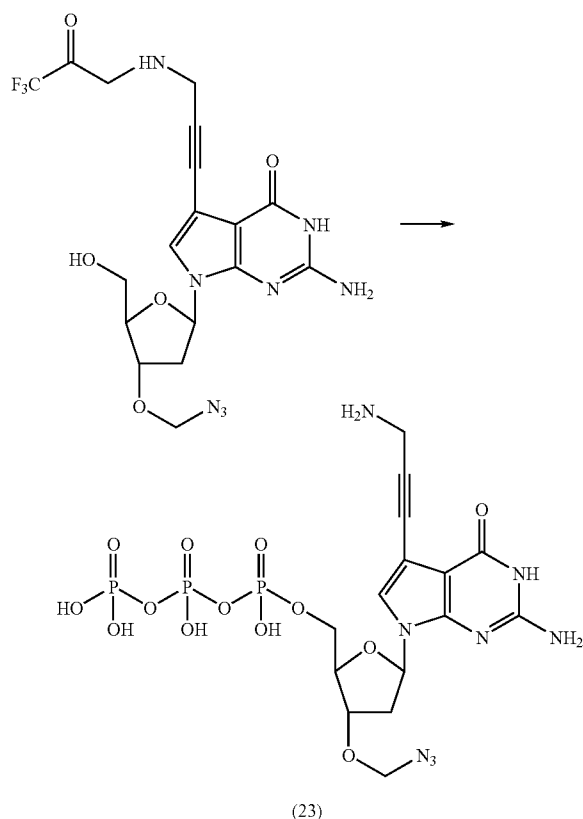
3'-O-Azidomethyl-7-deaza-7-[3-(2,2,2-trifluoroacetamido)-prop-1-ynyl]-2'-deoxyguanosine 5'-O-nucleoside triphosphate (23)
