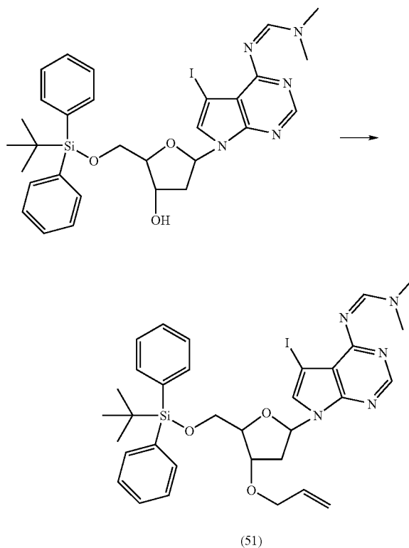
3'-O-Allyl-7-deaza-6-N,N-dimethylformadine-5'-O-diphenylsilyl-7-iodo-2'-deoxyadenosine (51)
