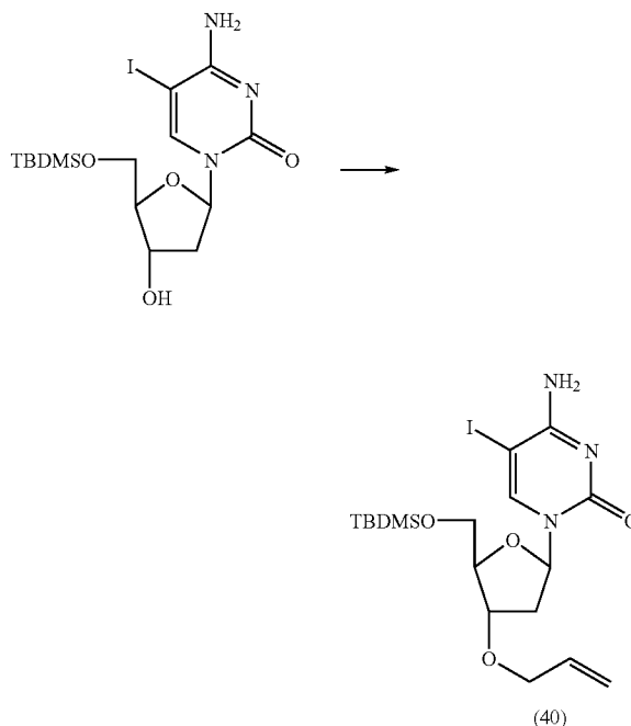
3'-O-Allyl-5'-O-(tert-butyltrimethylsilyl)-5-iodo-2'-deoxycytidine (40)
