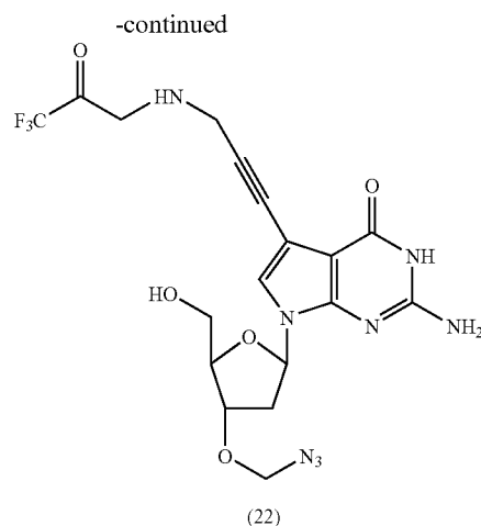
3'-O-Azidomethyl-7-deaza-7-[3-(2,2,2-trifluoroacetamido)-prop-1-ynyl]-2'-deoxyguanosine (22)
