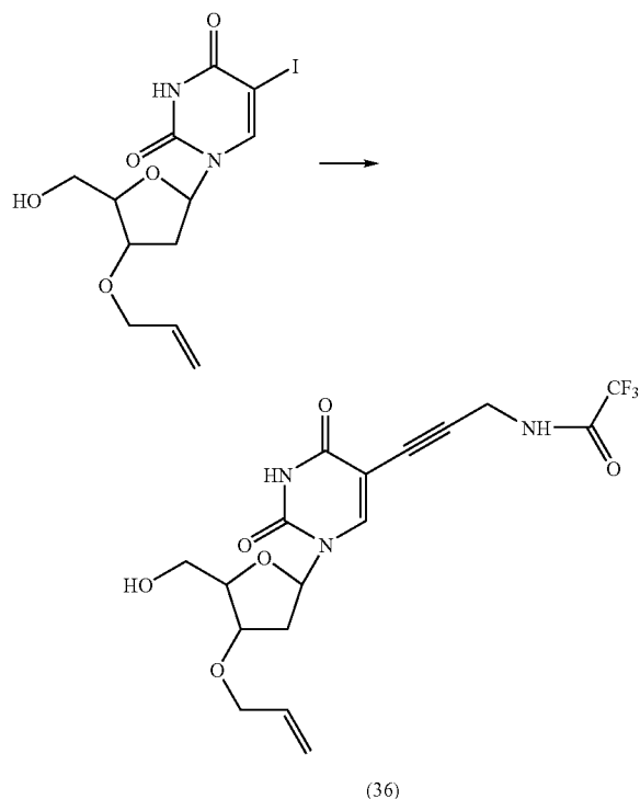
3'-O-Allyl-5-[3-(2,2,2-trifluoroacetamido)-prop-1-ynyl]-2'-deoxyuridine
