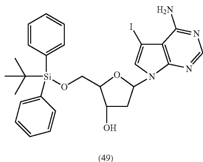
7-Deaza-5'-O-diphenylsilyl-7-iodo-2'-deoxyadenosine (49)
