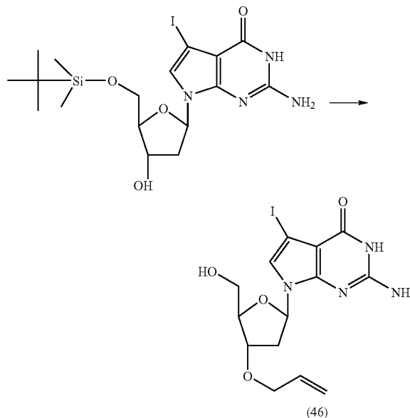
3'-O-Allyl-5'-O-(tert-butyl dimethylsilyl)-7-deaza-7-iodo-2'-deoxyguanosine (46)
