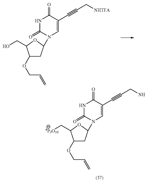
3'-O-Allyl-5-[3-(2,2,2-trifluoroacetamido)-prop-1-ynyl]-2'-deoxyuridine 5'-O-nucleoside triphosphate (37)
