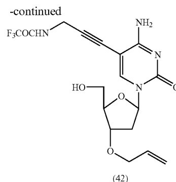
3'-O-Allyl-5-[3-(2,2,2-trifluoroacetamide)-prop-1-ynyl]-2'-deoxycytidine (42)
