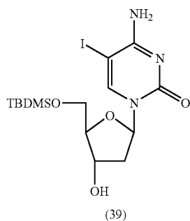
5'-O-(tert-Butyltrimethylsilyl)-5-iodo-2'-deoxycytidine (39)
