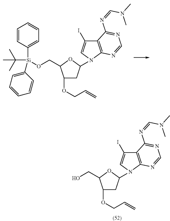
3'-O-Allyl-7-deaza-6-N,N-dimethylformadine-7-iodo-21-deoxyadenosine (52)
