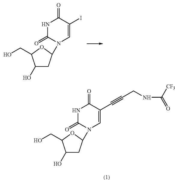
5-[3-(2,2,2-trifluoroacetamido)-prop-1-ynyl]-2'-deoxyuridine (1)
