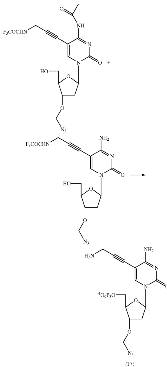
5-(3-Amino-prop-1-ynyl)-3'-O-azidomethyl-2'-deoxycytidine 5'-O-nucleoside triphosphate (17)
