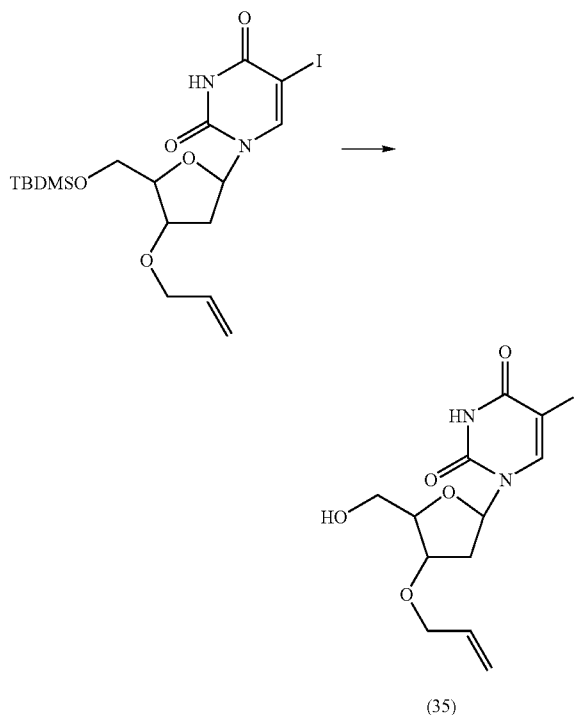
3'-O-Allyl-5-iodo-2'-deoxyuridine (35)
