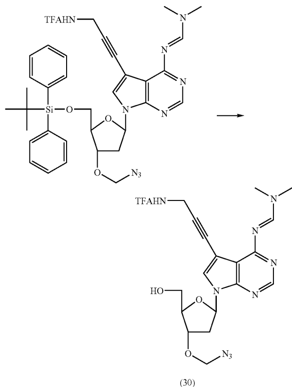
3'-O-Azidomethyl-7-deaza-4-N,N-dimethylformidin-7-[3-(2,2,2-trifluoroacetamido)-prop-1-ynyl]-2'-deoxyadenosine (30)
