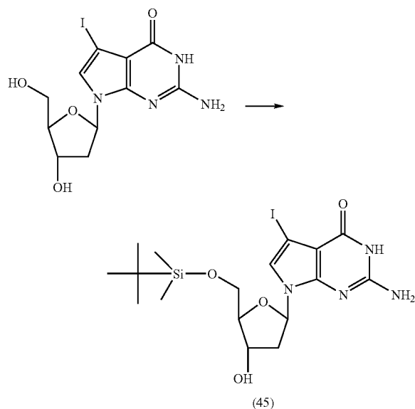
5'-O-(tert-Butyldimethylsilyl)-7-deaza-7-iodo-2'-deoxyguanosine (45)
