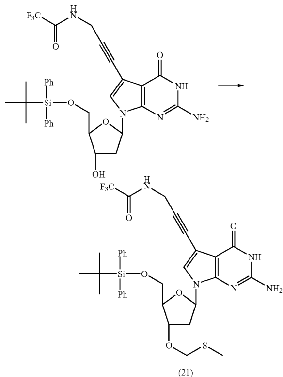
5'-O-(tert-Butyldiphenyl)-7-deaza-3'-O-methylthiol-methyl-7-[3-(2,2,2-trifluoroacetamido)-prop-1-ynyl]-2'-deoxyguanosine (21)
