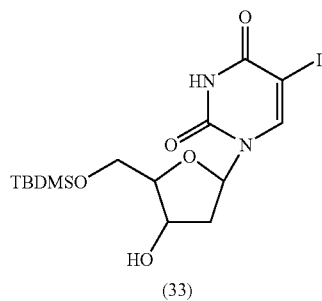
5'-O-(t-Butyldimethylsilyl)-5-iodo-2'-deoxyuridine (33)
