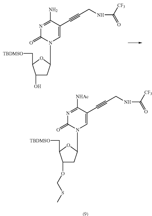
4-N-Acetyl-5'-O-(tert-butyl dimethylsilyl)-3'-O-(methylthiomethyl)-5-[3-(2,2,2-trifluoroacetamide)-prop-1-ynyl]-2'-deoxycytidine (9)
