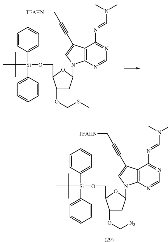
3'-O-Azidomethyl-5'-O-(tert-butyldiphenylsilyl)-7-deaza-4-N,N-dimethylformadin-7-[3-(2,2,2-trifluoroacetamido)-prop-1-ynyl]-2'-deoxyadenosine (29)
