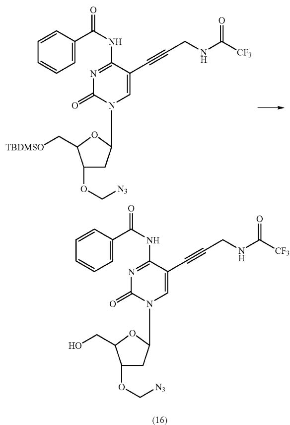
4-N-Benzoyl-3'-O-azidomethyl-5-[3-(2,2,2-trifluoroacetamido)-prop-1-ynyl]-2'-deoxycytidine (16)
