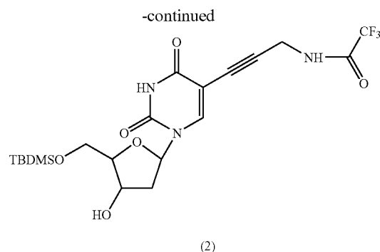
5'-O-(tert-butyldimethylsilyl)-5-[3-(2,2,2-trifluoroacetamido)-prop-1-ynyl]-2'-deoxyuridine (2)
