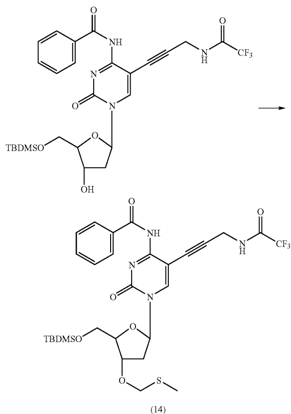
4-N-Benzoyl-5'-O-(tert-butyldimethylsilyl)-3'-O-methylthiomethyl-5-[3-(2,2,2-trifluoroacetamido)-prop-1-ynyl]-2'-deoxycytidine (14)
