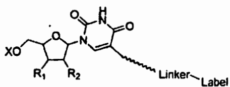
Uridine C5-linker
