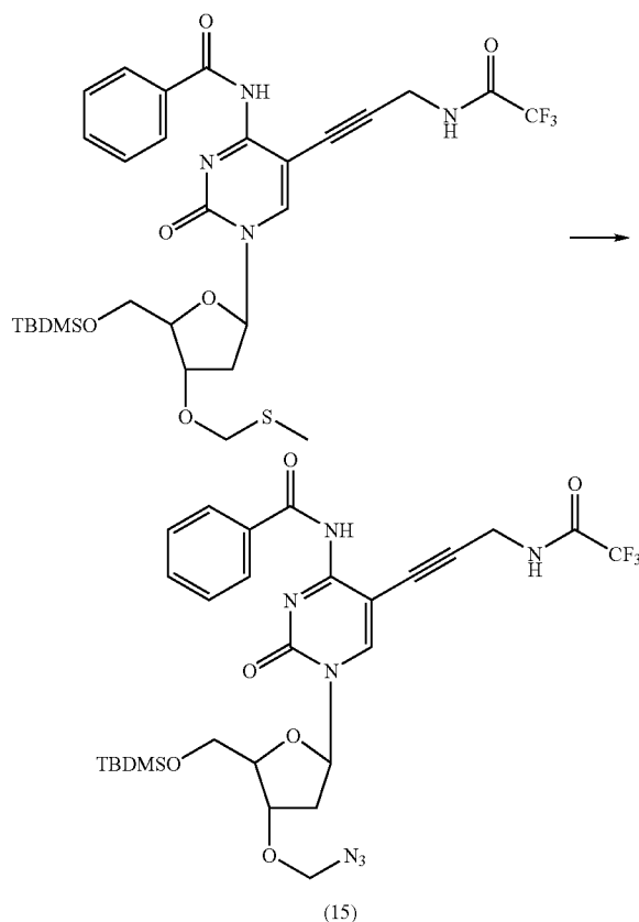
4-N-Benzoyl-5'-O-(tert-butyldimethylsilyl)-3'-O-azidomethyl-5-[3-(2,2,2-trifluoroacetamido)-prop-1-ynyl]-2'-deoxycytidine (15)
