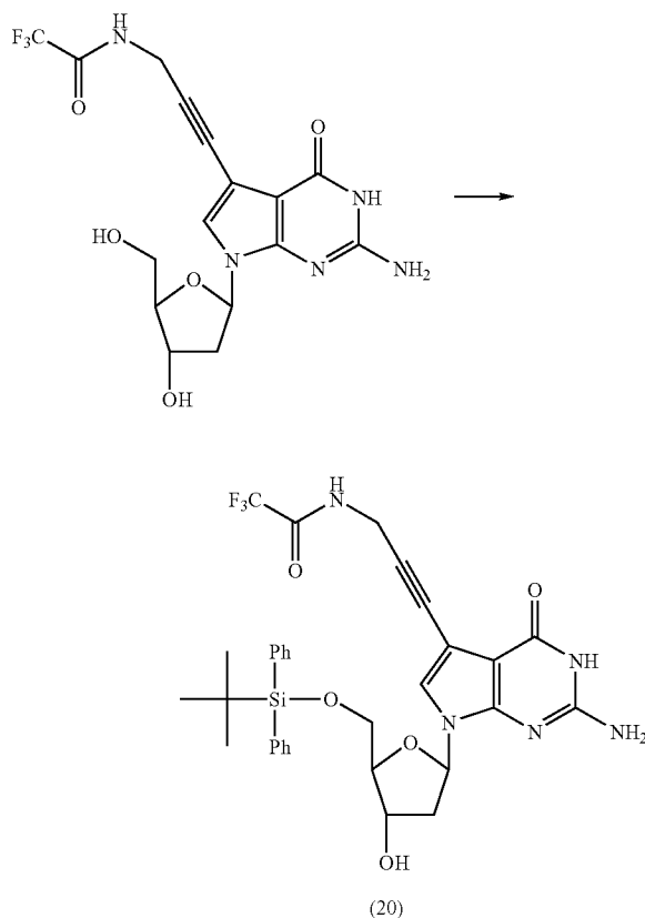
5'-O-(tert-Butyldiphenyl)-7-deaza-7-[3-(2,2,2-trifluoroacetamido)-prop-1-ynyl]-2'-deoxyguanosine (20)
