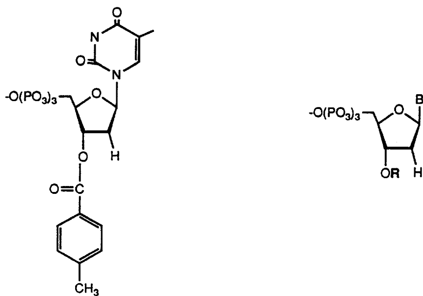
3'-TOLUIC ACID ESTER OF THYMIDINE 5'-TRIPHOSPHATE
