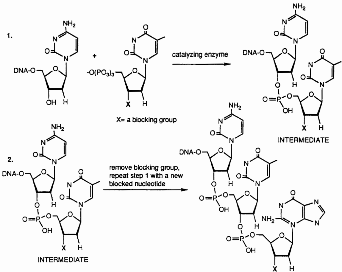
FIGURE 1. ENZYMAIC SYNTHESIS OF DNA USING A MODIFIED NUCLEOTIDE
