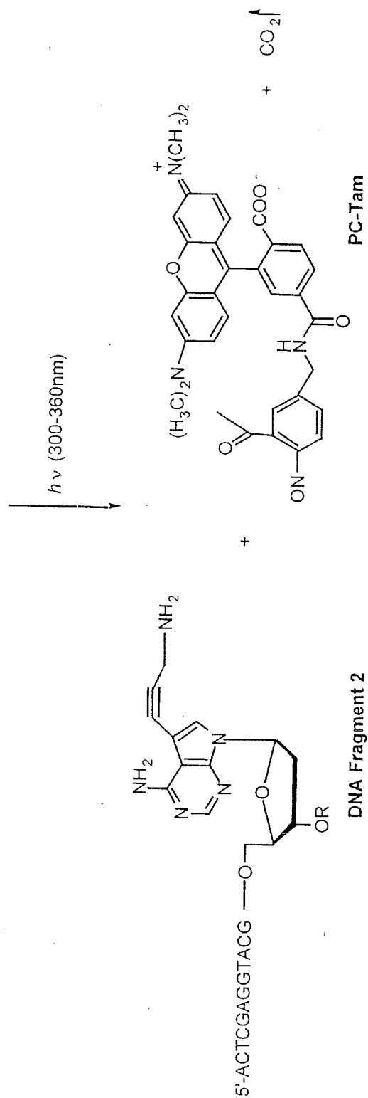
FIGURE 10 5'-ACTCGAGGTACG — O — DNA Fragment 1 (DNA-Photolinker 3 -RO-A-Tam)
