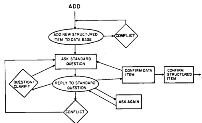
Fig. 28. User-oriented discourse model. (From Woods et al. [169].)
