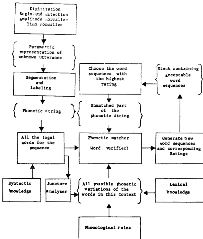
Fig. 10. Flow chart of a typical CSR system.
