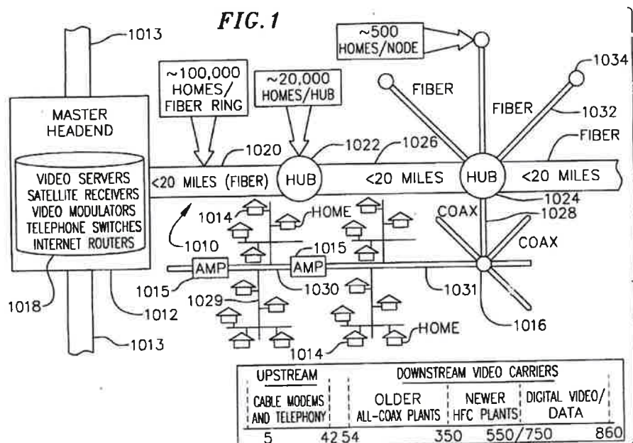
Figure 1 of Quigley “is a schematic diagram of a hybrid fiber coaxial (HFC) network showing typical pathways for data transmission between the
