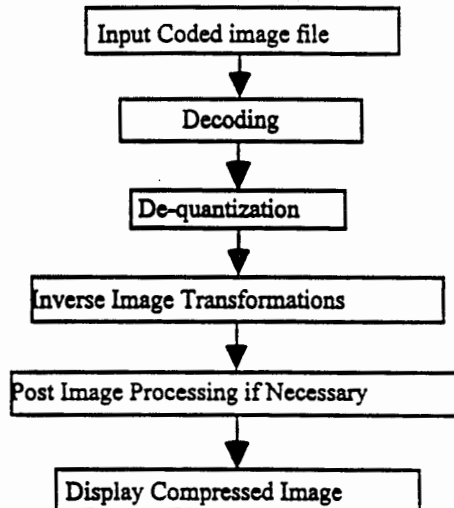
Figure 2: Image decompression
