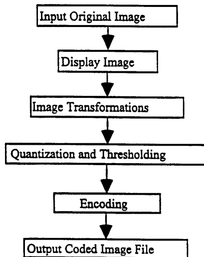
Figure 1: Image compression
