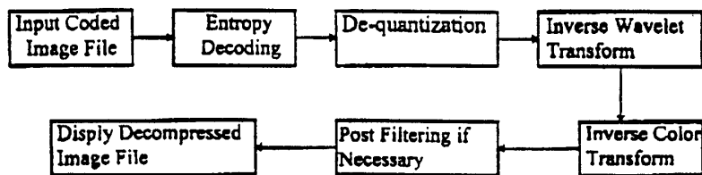
Figure 2: Decompression flow chart for Method 1
