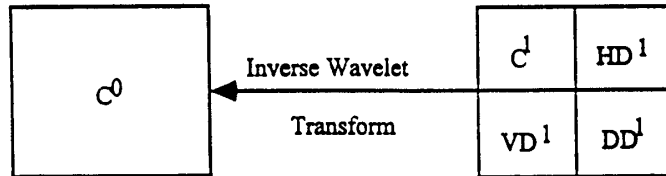
Figure 5. One-level wavelet reconstruction
