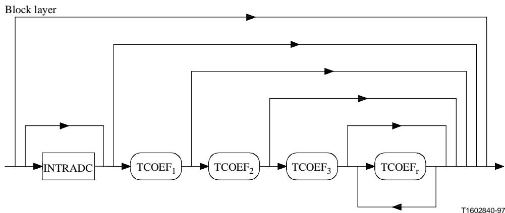
Figure E.1/H.263 – Structure of SAC Block layer
