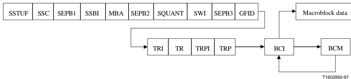
Figure N.3/H.263 – Structure of slice layer for NEWPRED
