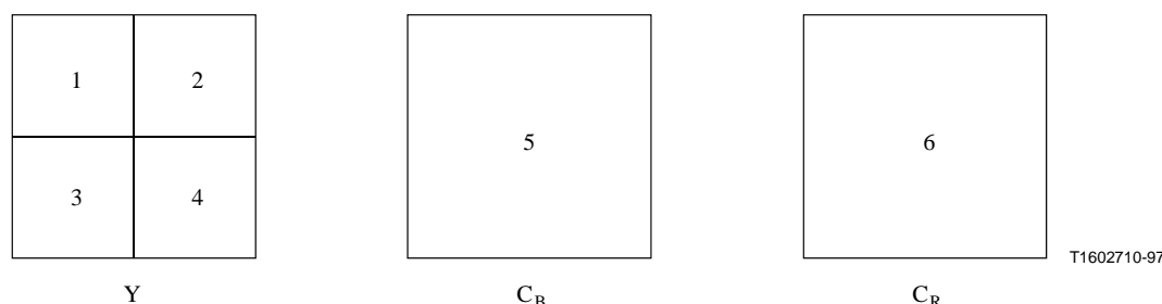
Figure 5/H.263 – Arrangement of blocks in a macroblock
