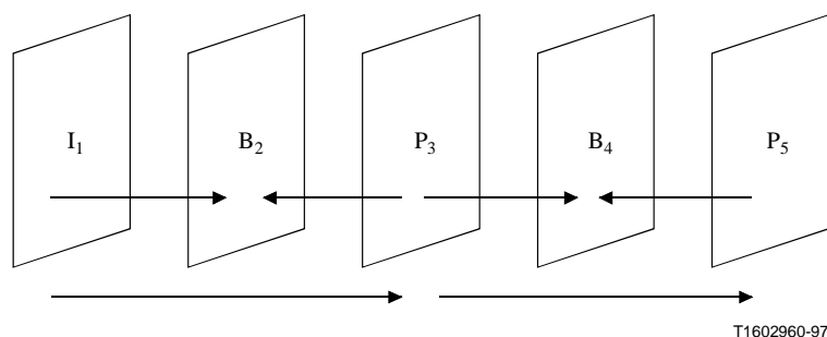
Figure O.1/H.263 – Illustration of B-picture prediction dependencies
