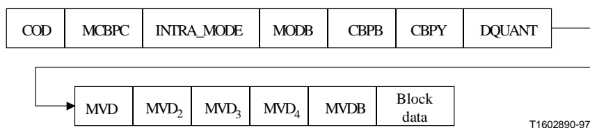
Figure I.1/H.263 – Structure of macroblock layer
