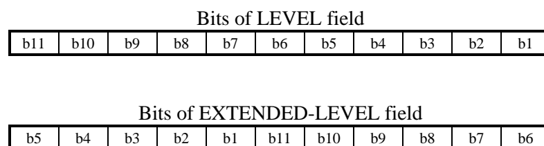
Figure T.1/H.263 – Cyclic rotation of coefficient representation
