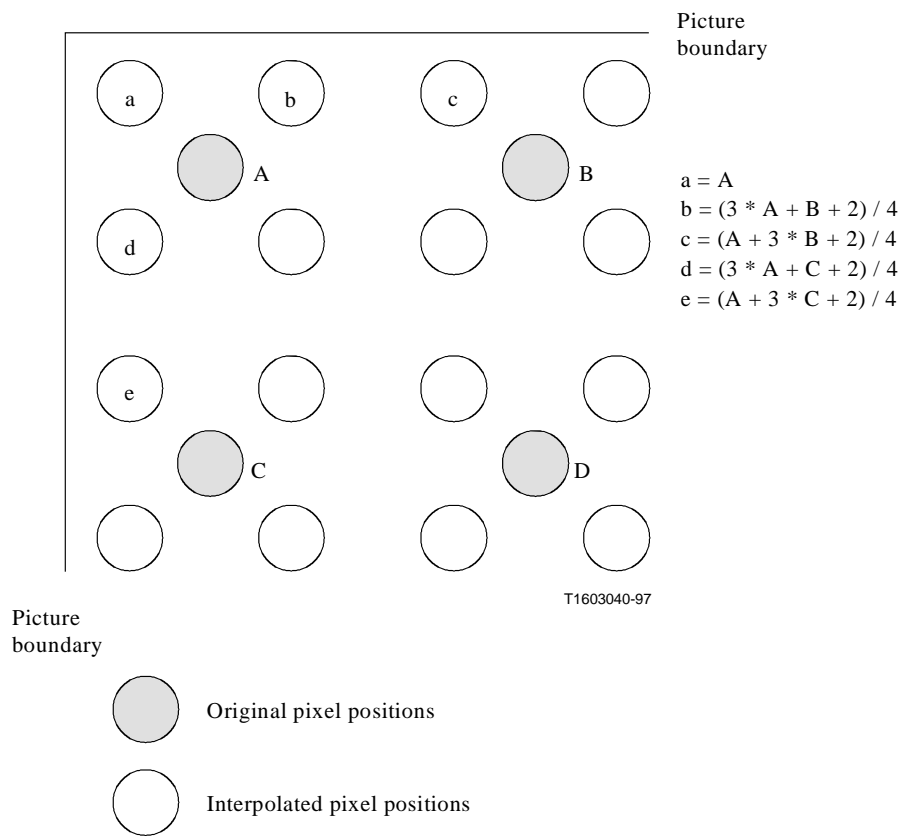
Figure O.9/H.263 – Method for 2-D interpolation at boundaries
