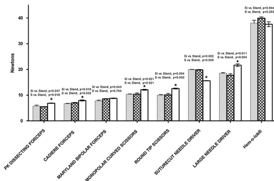
FIG. 6. Comparison of grip forces in various instruments among different da Vinci robotic platforms. White bar = da Vinci Standard; striped bar = da Vinci Si; gray bars = da Vinci S; * = Standard platforms significantly different from the Si and S platforms on post hoc analysis of variance test.
