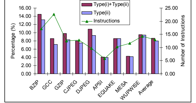
Figure 1. Percentage of wrong-path instruction over total instructions executed and average number of wrong-path instructions per mispredicted branch.
