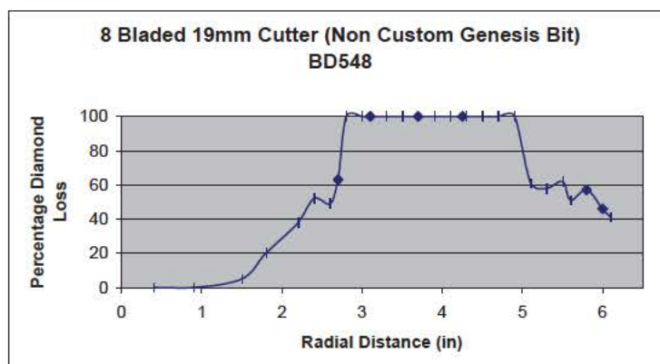
Figure 13b. Actual wear from dull analysis
