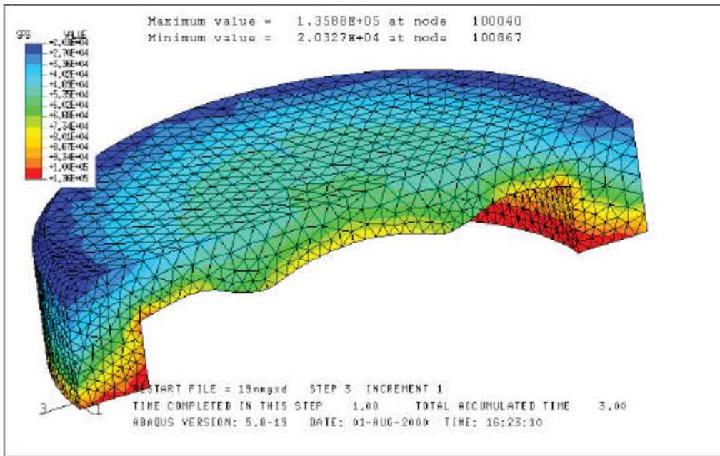
Figure 8. Variance of internal residual stress throughout the diamond layer
