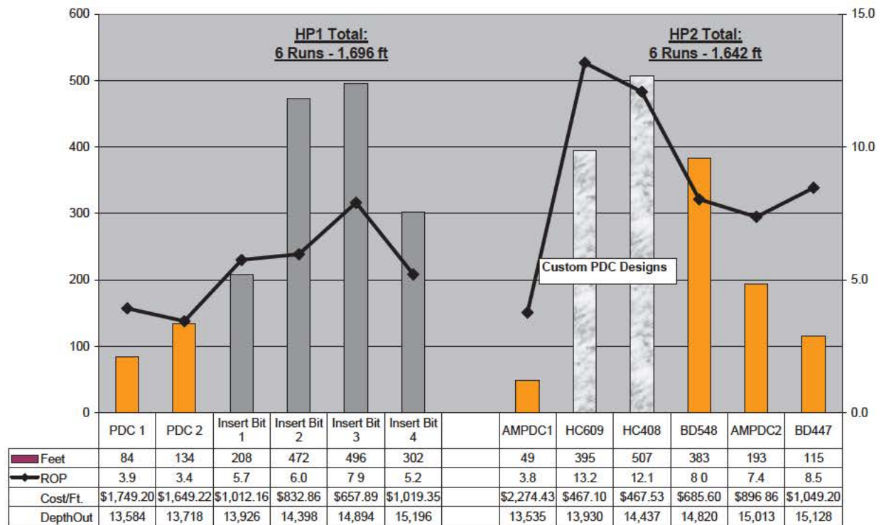
Figure 14. HP2 performance and comparison with HP1
