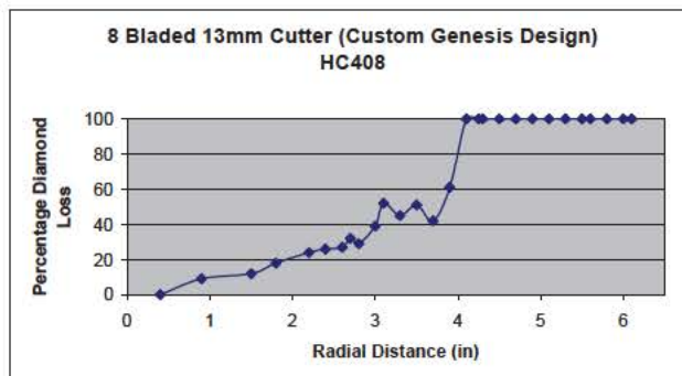
Figure 12d. Actual wear from dull analysis
