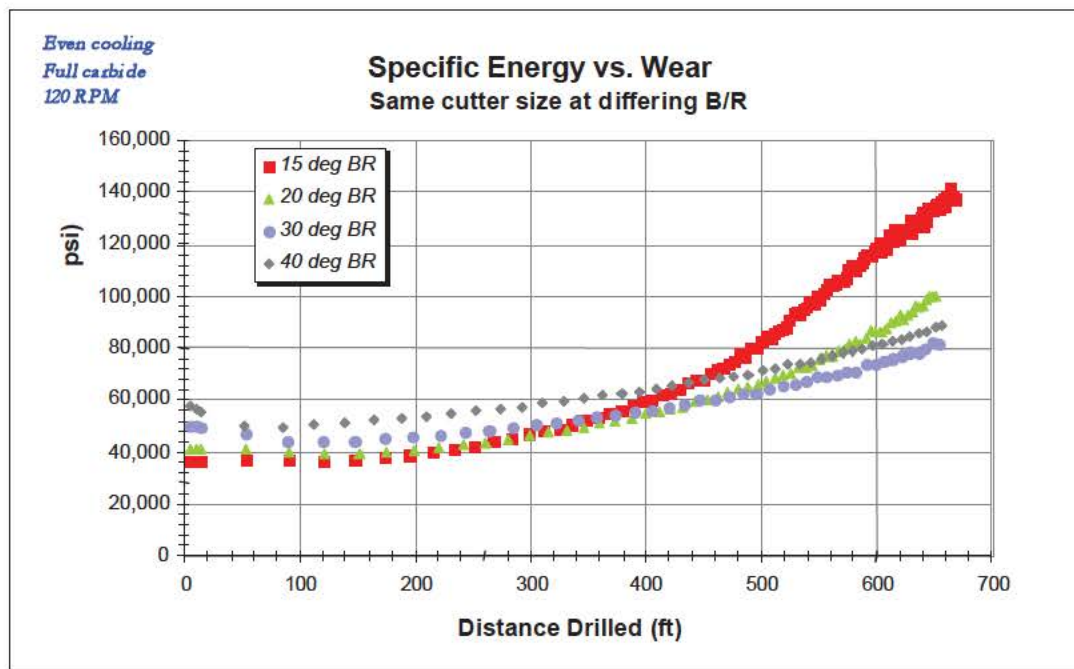
Figure 7: As cutters wear the higher Backrakes wear more slowly
