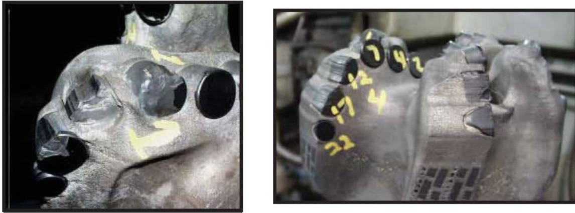
Figure 4. Dynamic and smooth wear of PDC cutters
