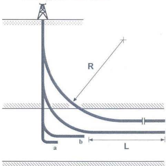
Fig. 1. Horizontal well profiles:
