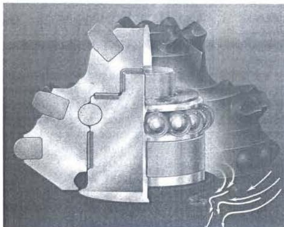
Fig. 2. Cross section of precision turned friction bearing for slim hole rock-bits. (Source: Smith International)
