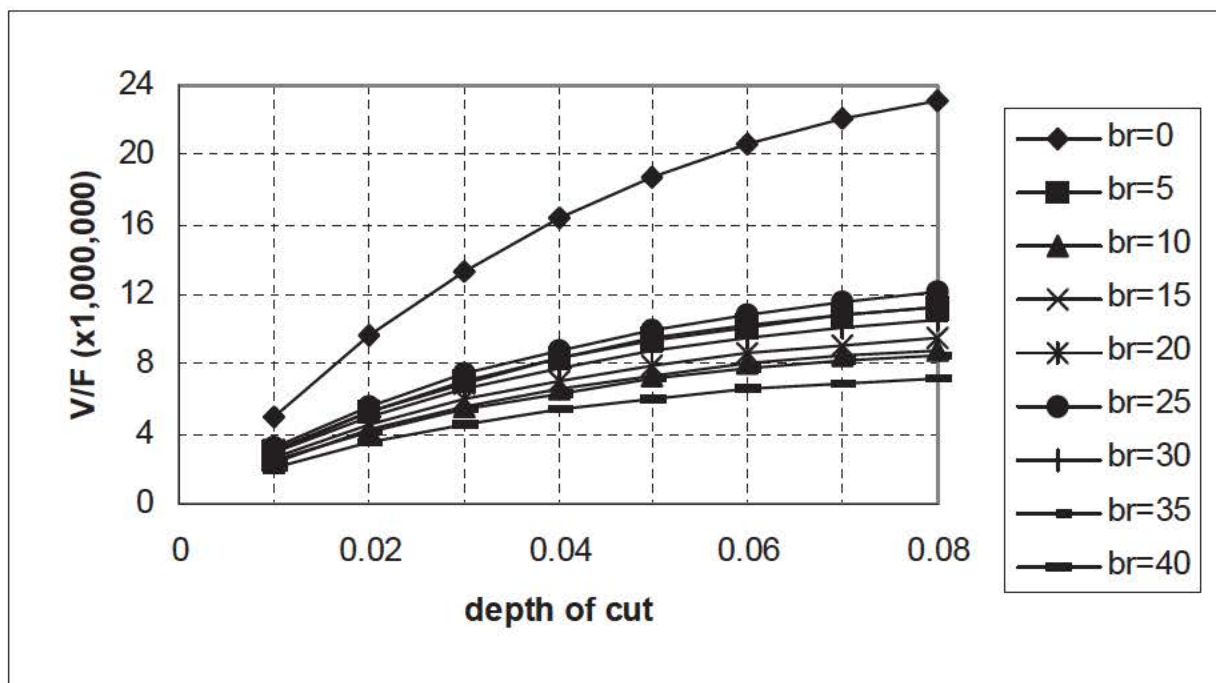
Figure 8. Specific volume versus depth of cut.
