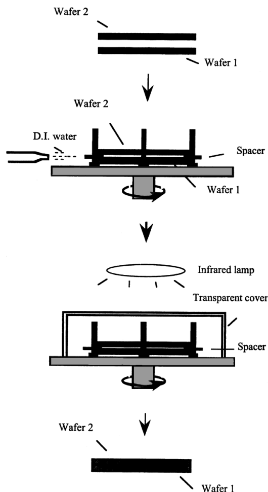
Fig. 6. Schematic of microcleanroom set-up and procedure.
