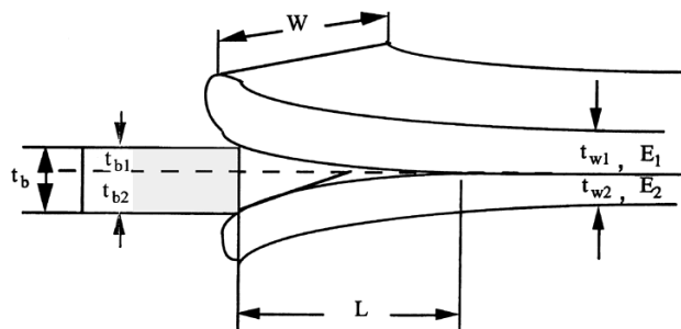
Fig. 2. Schematic of the crack-opening method for surface energy measurement.
