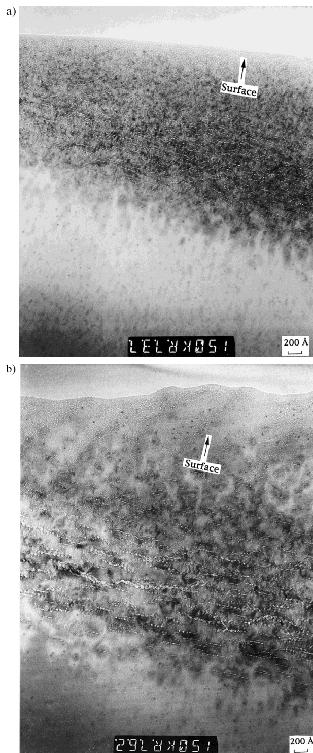
Fig. 13. TEM images of platelets in as-implanted c-cut sapphire that was implanted by H 2 + at a dose of 5 × 10 16 /cm 2 , an energy of 160 keV, and a temperature of a) 450 °C and b) 750 °C.
