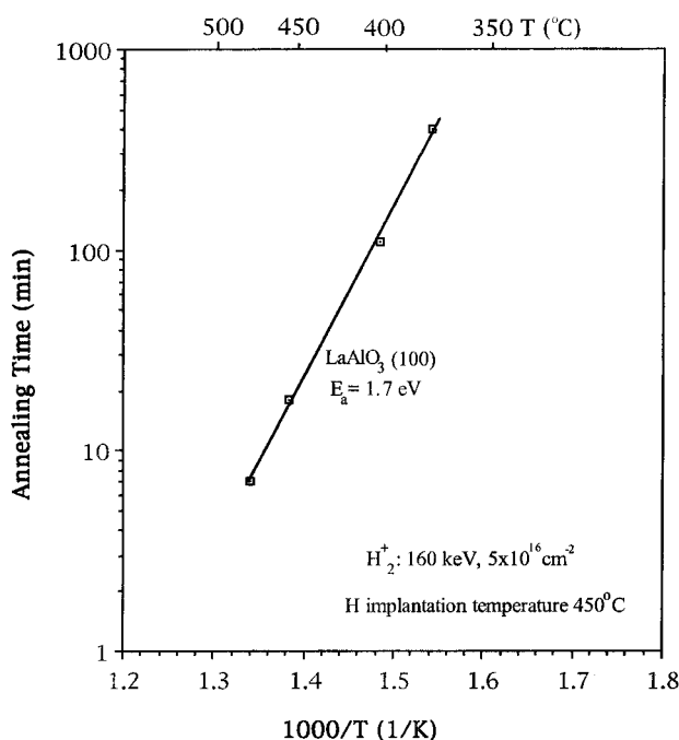
Fig. 14. Blistering time as a function of annealing temperature of \text{LaAlO}_3 samples that were implanted by \text{H}_2^+ at 450 °C with an \text{H}_2 dose of 5 \times 10^{16}/\text{cm}^2 at 160 keV.
