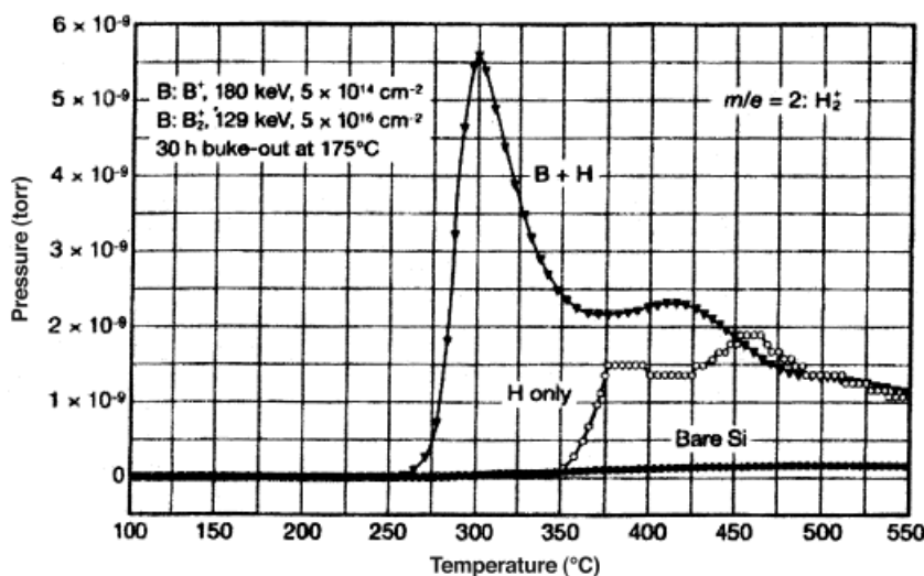
Fig. 12. H evolution with temperature for H-only and B + H co-implanted Si samples measured by quadrupole mass spectrometry.
