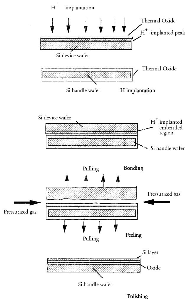
Fig. 15. Schematic of the H-induced embrittlement and layer peeling process.
