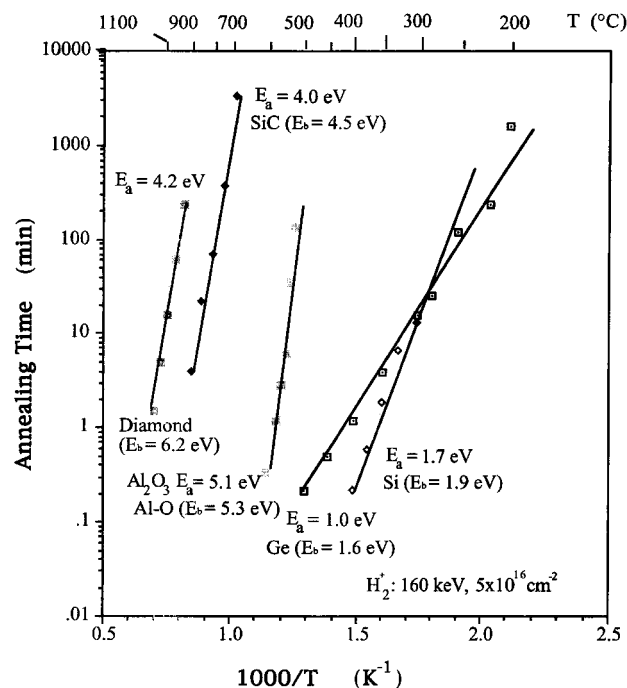
Fig. 11. Experimentally determined activation energies E_a of H-implanted Si, Ge, SiC, diamond, and sapphire samples and their corresponding bond energies E_b .
