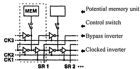
Fig.3 Configuration of the shift register.
