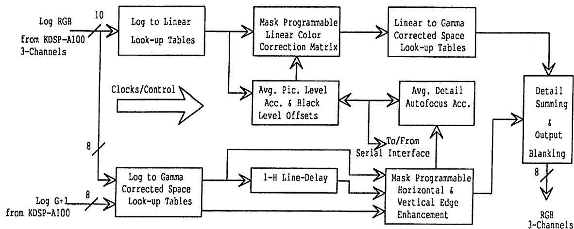
Fig. 12 RGB Post-Processor Functions
