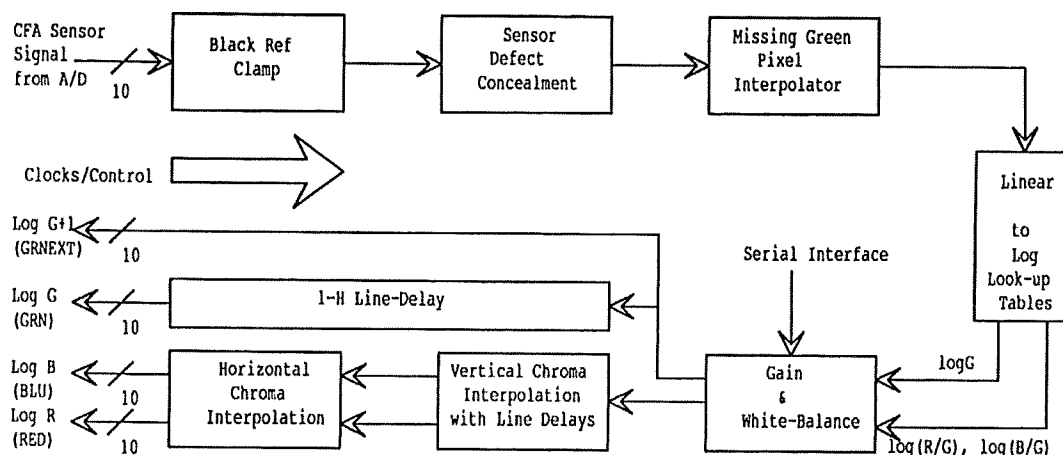
Fig. 10 CFA Processor Functions
