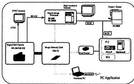
Fig. 2 Digital Still Camera System
