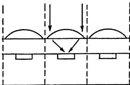
Fig. 8 Lenslet Structure
