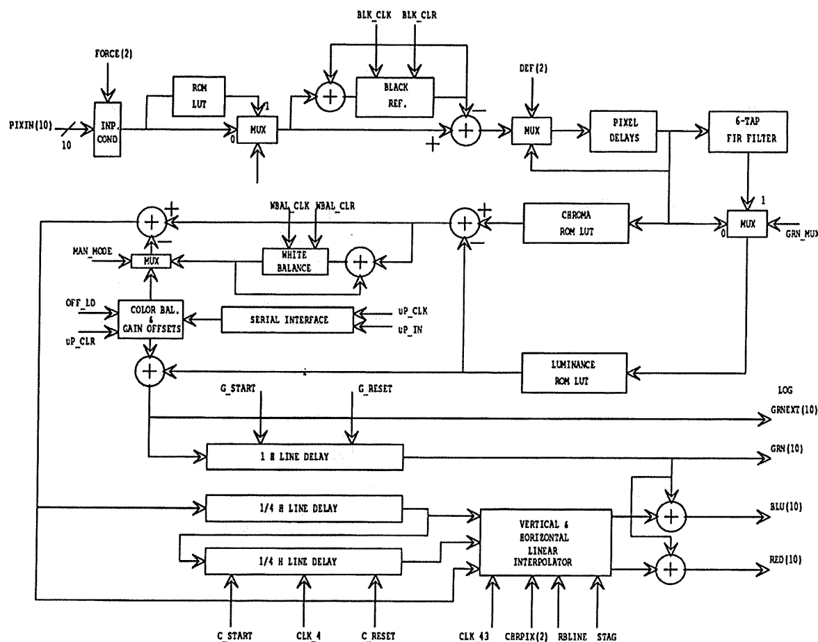
Fig. 11 CFA Processor Implementation
