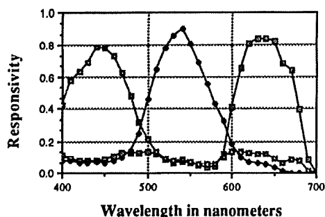
Fig. 14 CCD Camera Color Responsivities
