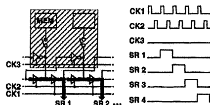
Fig.4 Timing diagram of the Full mode.
