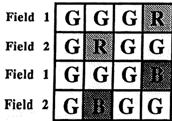
Fig. 6 Field Staggered 3G CFA
