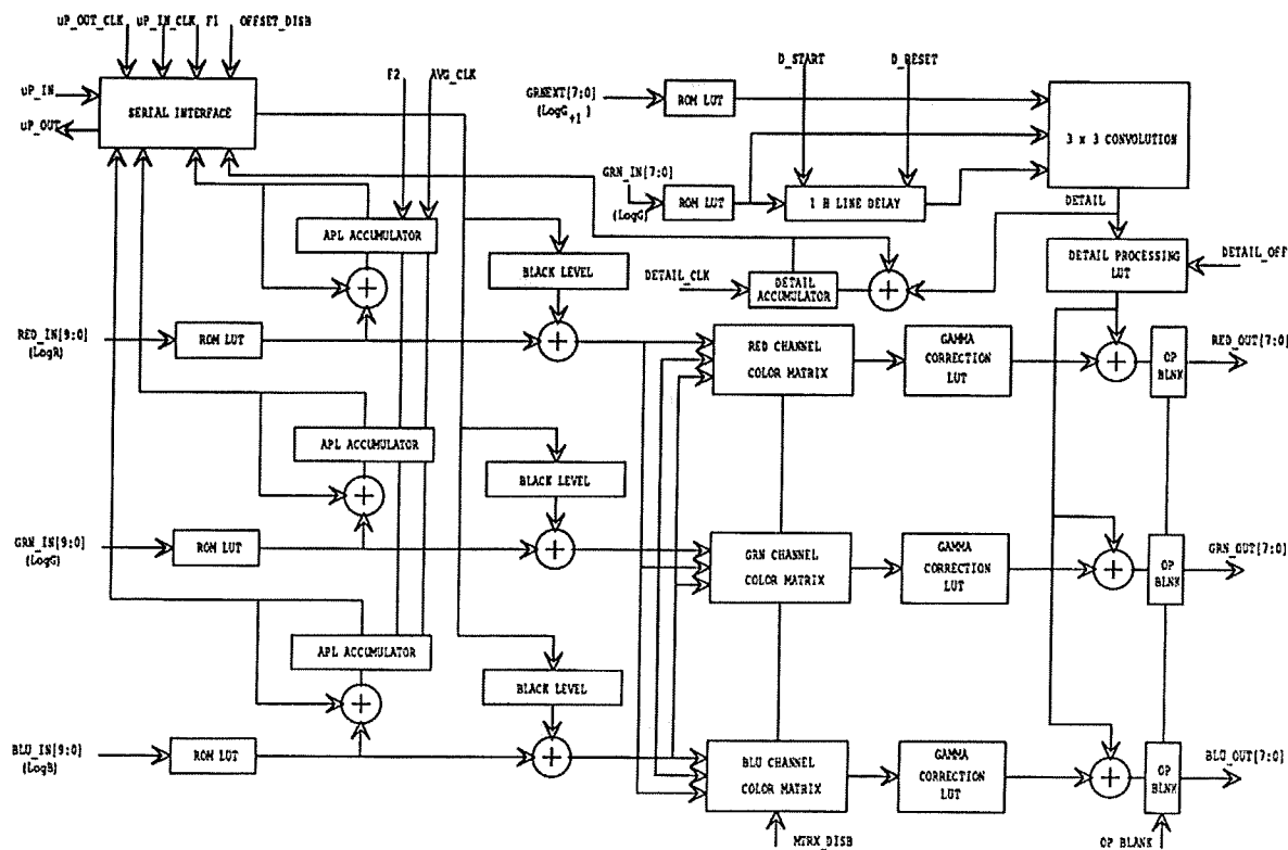
Fig. 13 RGB Post-Processor Implementation
