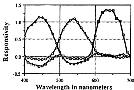
Fig. 16 Matrixed Camera Responsivities
