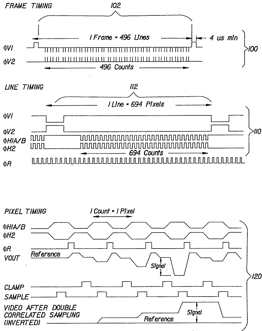
Timing Diagram - Normal Single Register Readout
