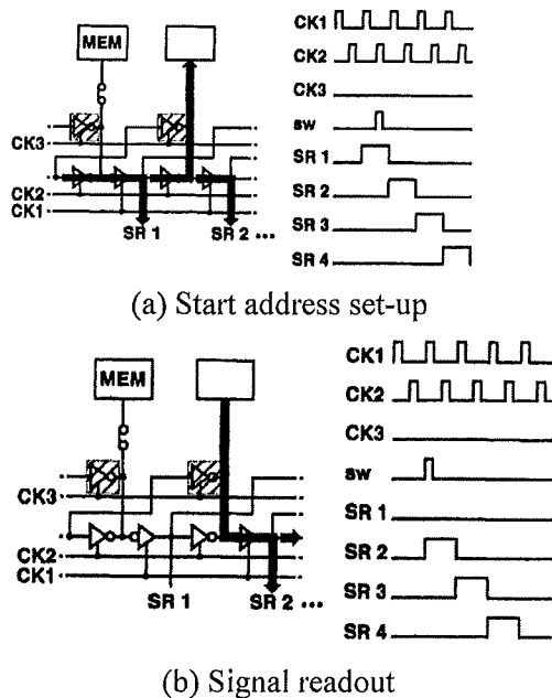
Fig.6 Timing diagram of the Block mode.
