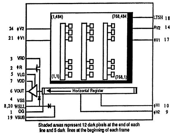
Fig. 2 CCD Sensor Block Diagram
