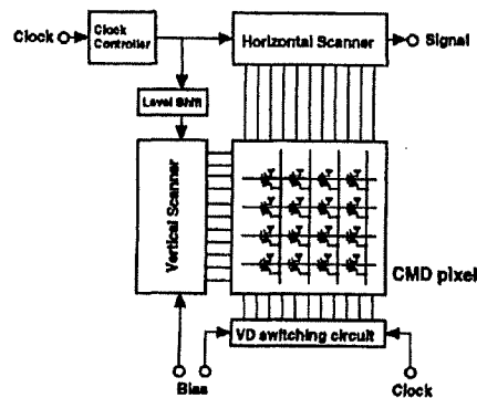
Fig.1 Block diagram of the CMD image sensor.
