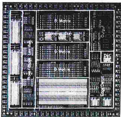
Photo 3 RGB Post-Processor Layout
