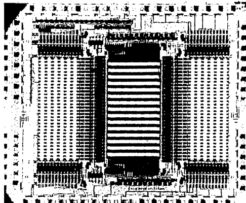
Fig. 1: EBS-1.1.1 Die Photograph
