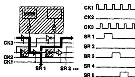
Fig.5 Timing diagram of the Skip mode.
