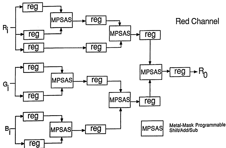
Fig. 17 Red Channel Matrix Implementation
