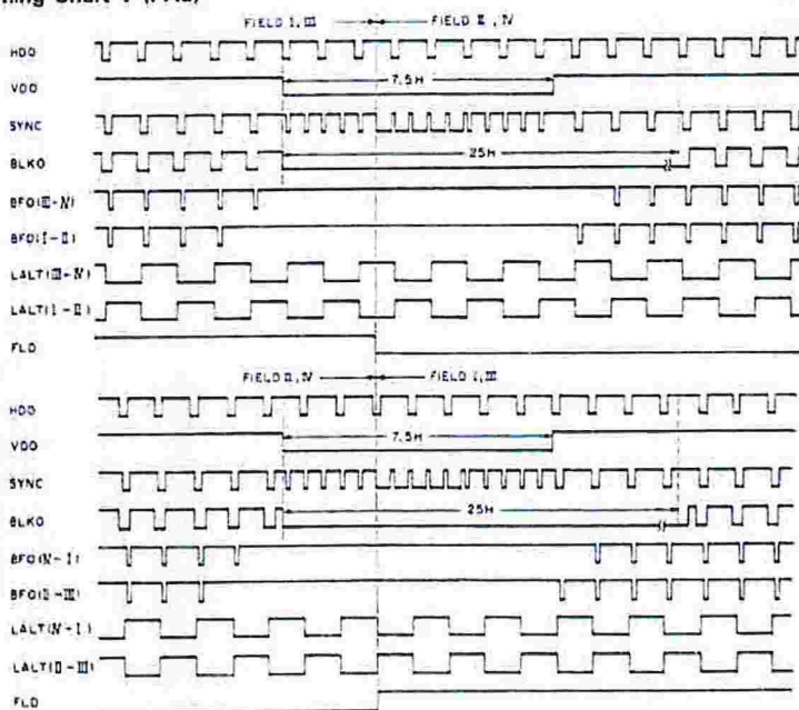
Timing Chart V (PAL)
