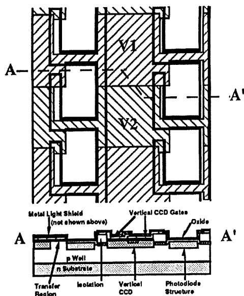
Fig. 4 CCD Pixel Architecture
