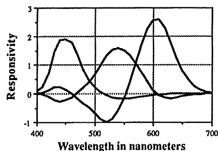
Fig. 15 Optimum Camera Responsivities
