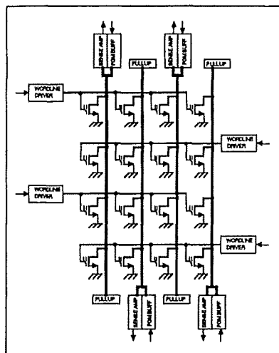
Fig. 3: EPLD NOR Plane
