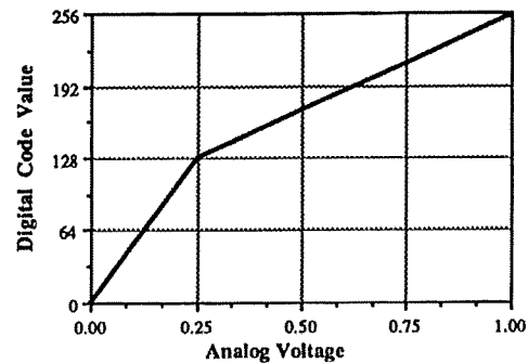
Fig. 9 Dual-Slope A/D Characteristic
