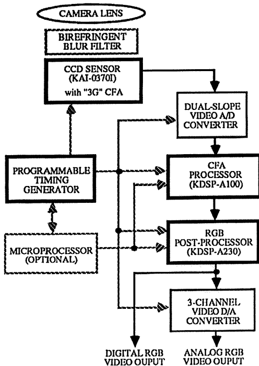
Fig. 1 Digital Camera Block Diagram
