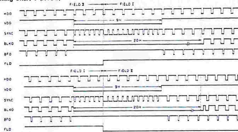
Timing Chart V (PAL)
