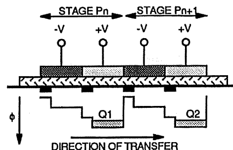
Fig. 3 True Two-Phase CCD Cross Section
