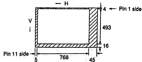
Fig. 1 Optical black configuration
