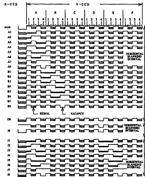
Fig.4 Potential diagram of VT-method
