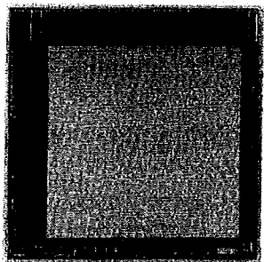
Fig. 10 CMD image sensor micrograph.
