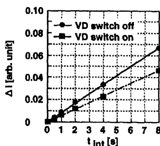
Fig.9 Dark current generation.
