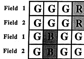
Fig. 7 Line Staggered 3G CFA
