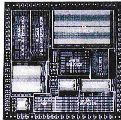
Photo 2 CFA Processor Layout
