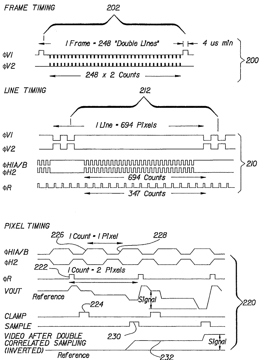
Timing Diagram - 2:1 Vertical and Horizontal "Binning"
