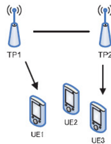
(b) Coordinated Scheduling/Beamforming (CS/CB)
